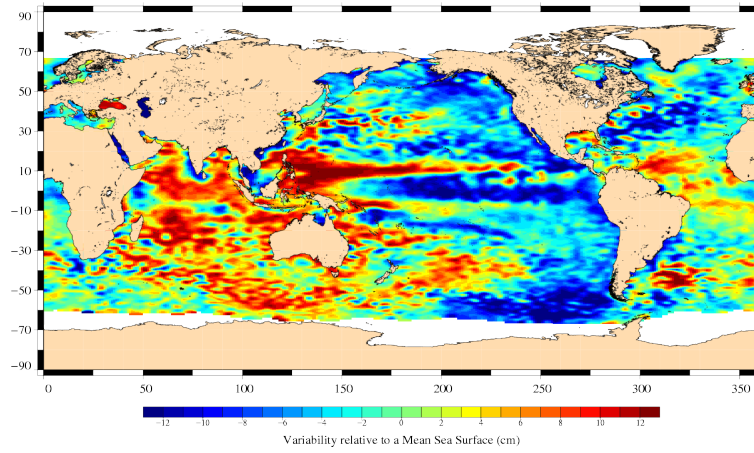
FIG. 18 – Sea level anomaly relative to MSS for cycle 073.
