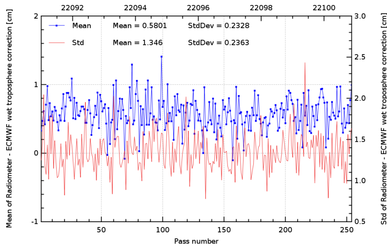
FIG. 11 – Pass monitoring of wet troposphere differences between radiometer and ECMWF model for Jason-2 cycle 073.
