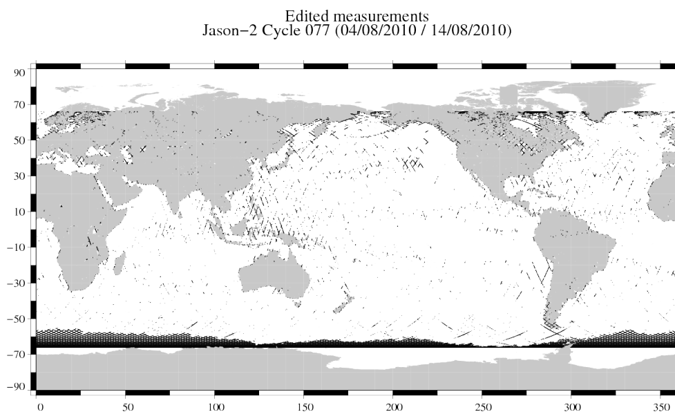
FIG. 2 – Edited measurements for cycle 077.
