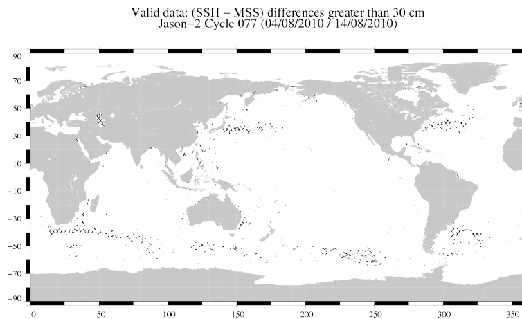
FIG. 19 – Differences higher than a 30 cm threshold for cycle 077.
