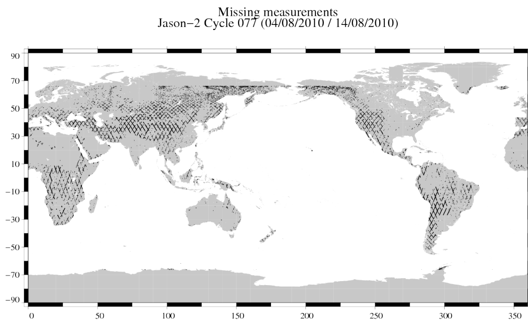
FIG. 1 – Missing measurements for cycle 077.
