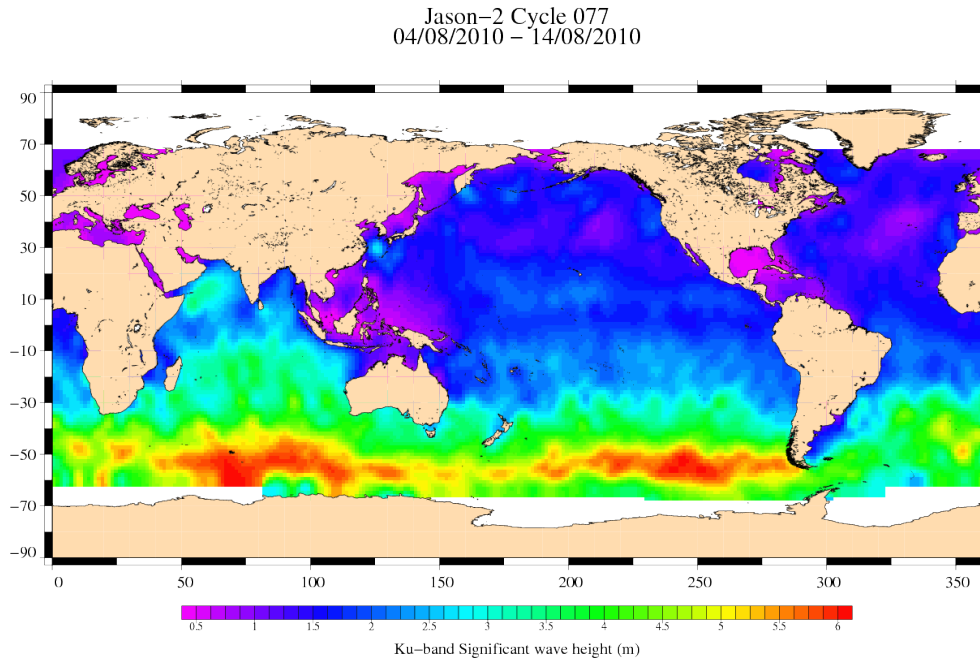
FIG. 5 – Significant wave height for cycle 077.
