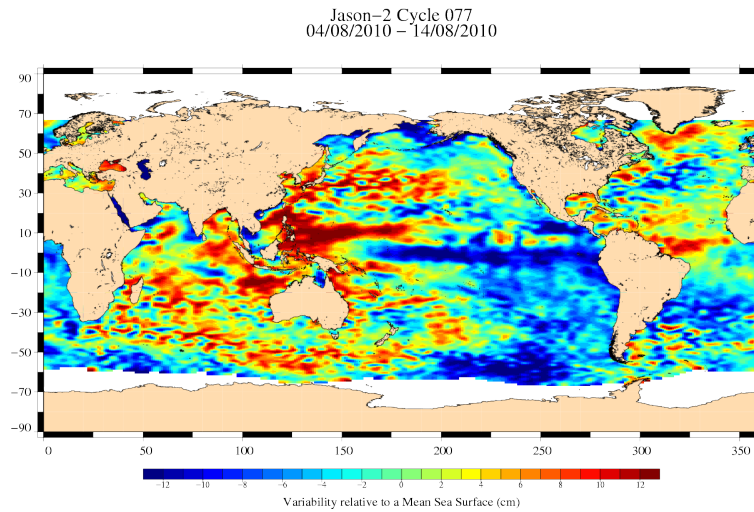
FIG. 18 – Sea level anomaly relative to MSS for cycle 077.
