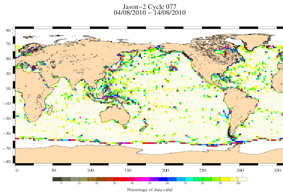
FIG. 3 – Percentage of valid measurements for cycle 077.
