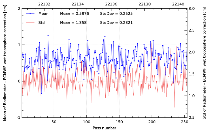
FIG. 11 – Pass monitoring of wet troposphere differences between radiometer and ECMWF model for Jason-2 cycle 077.
