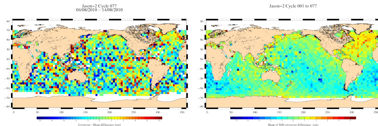
FIG. 13 – Mean SSH at crossovers for cycle 077 (left) and over the whole Jason-2 period (right).
