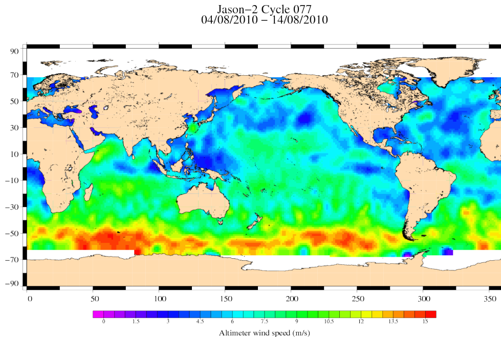
FIG. 9 – Altimeter wind speed for cycle 077.
