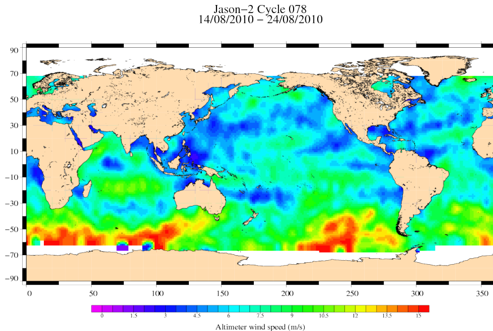
FIG. 9 – Altimeter wind speed for cycle 078.
