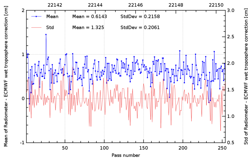
FIG. 11 – Pass monitoring of wet troposphere differences between radiometer and ECMWF model for Jason-2 cycle 078.
