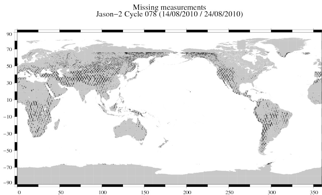
FIG. 1 – Missing measurements for cycle 078.
