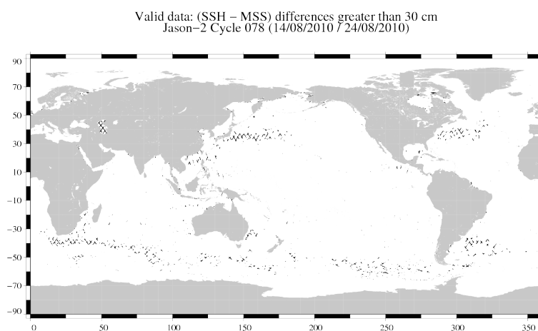
FIG. 19 – Differences higher than a 30 cm threshold for cycle 078.
