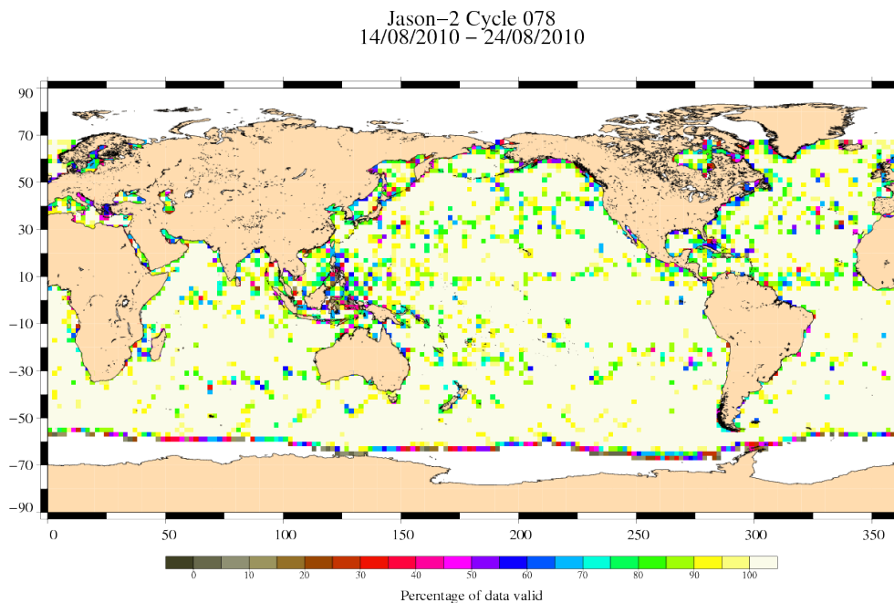
FIG. 3 – Percentage of valid measurements for cycle 078.
