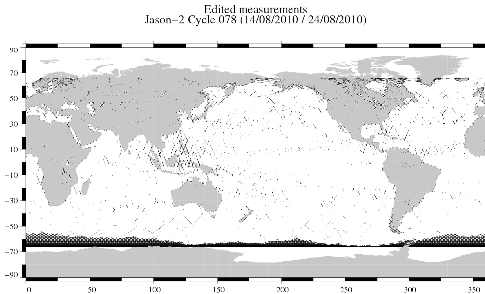
FIG. 2 – Edited measurements for cycle 078.
