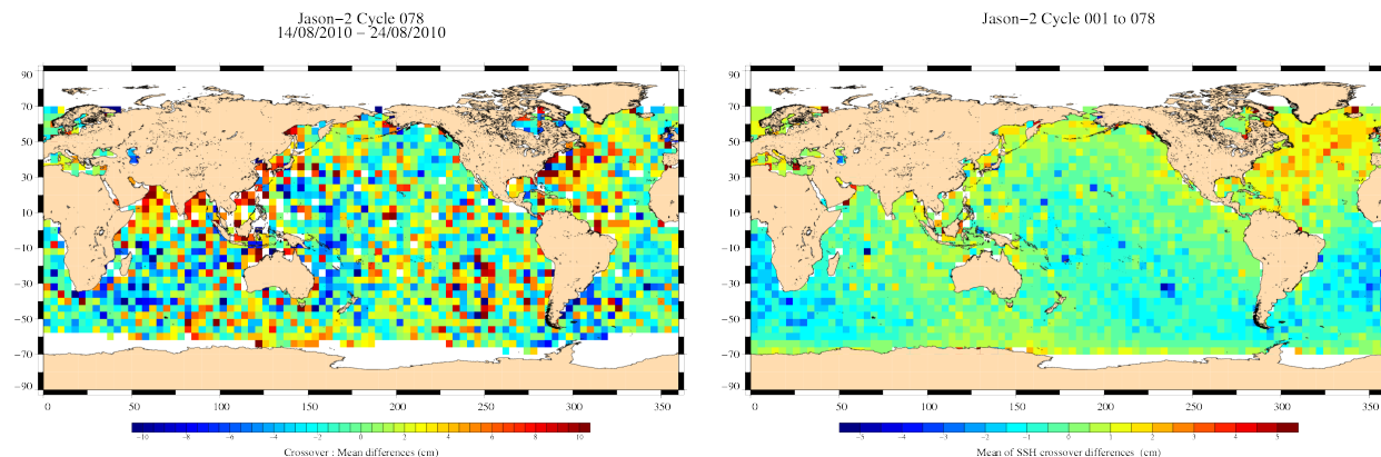
FIG. 13 – Mean SSH at crossovers for cycle 078 (left) and over the whole Jason-2 period (right).
