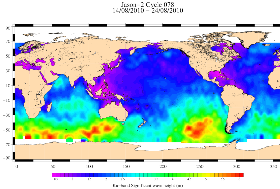
FIG. 5 – Significant wave height for cycle 078.
