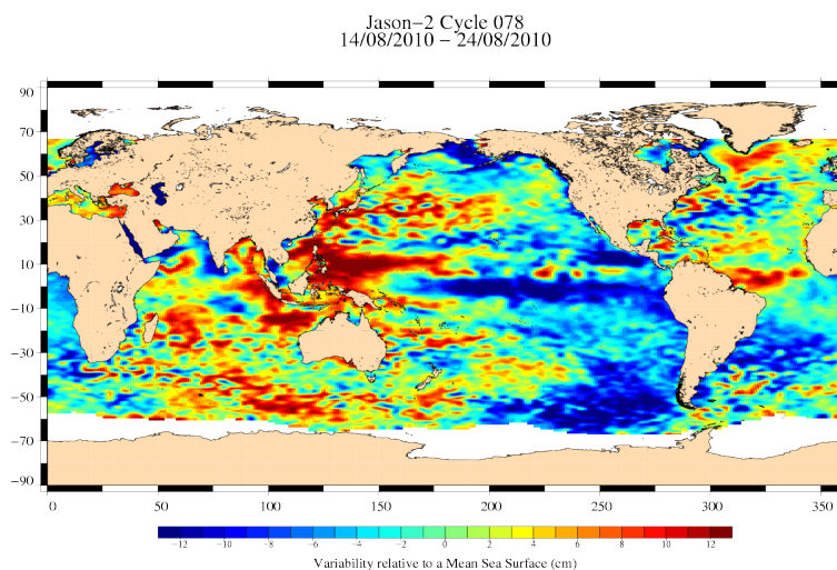
FIG. 18 – Sea level anomaly relative to MSS for cycle 078.
