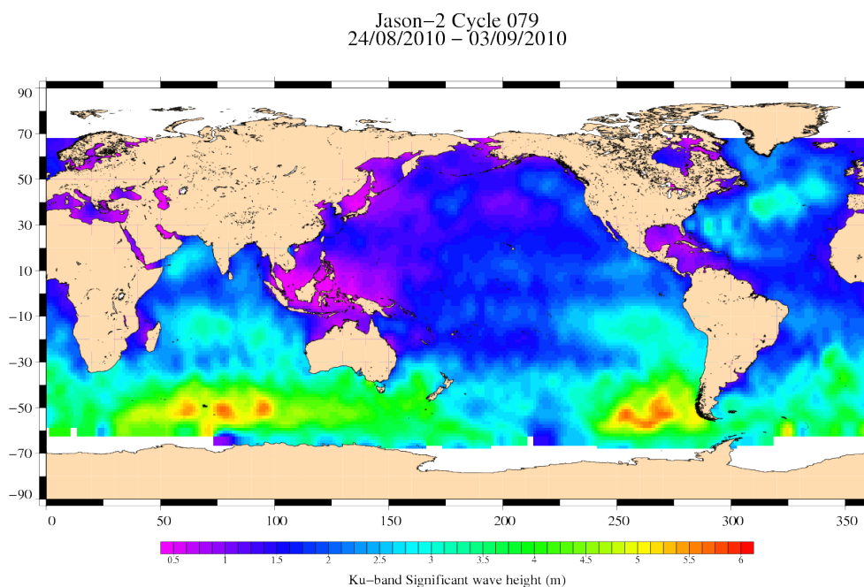
FIG. 5 – Significant wave height for cycle 079.
