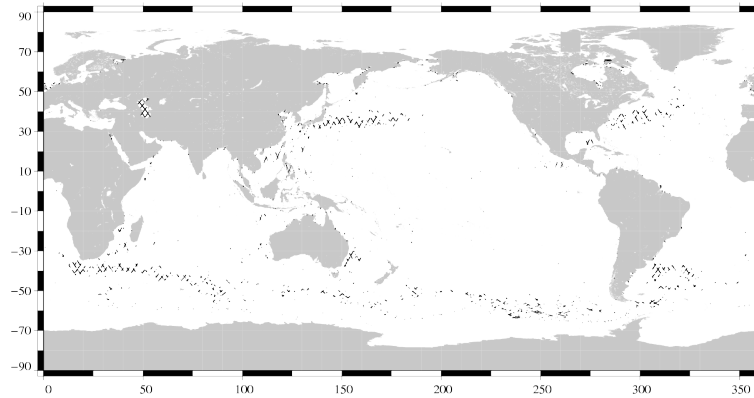
FIG. 19 – Differences higher than a 30 cm threshold for cycle 079.
