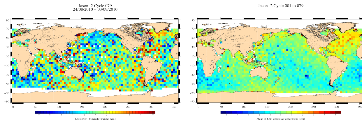
FIG. 13 – Mean SSH at crossovers for cycle 079 (left) and over the whole Jason-2 period (right).
