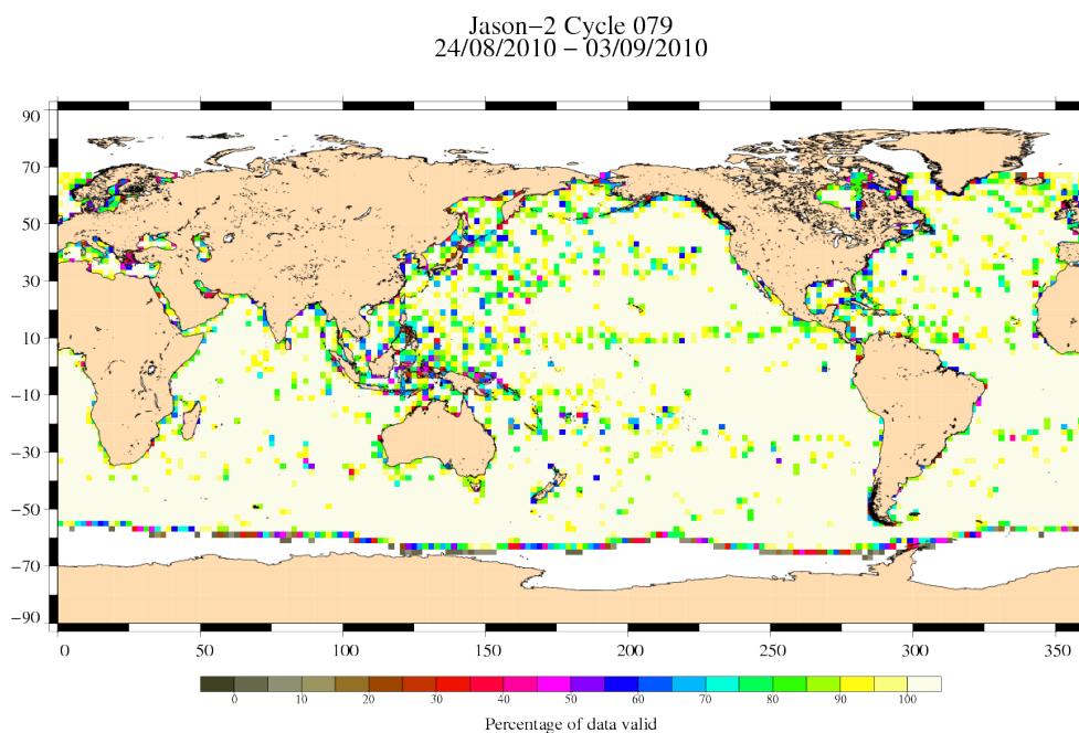
FIG. 3 – Percentage of valid measurements for cycle 079.
