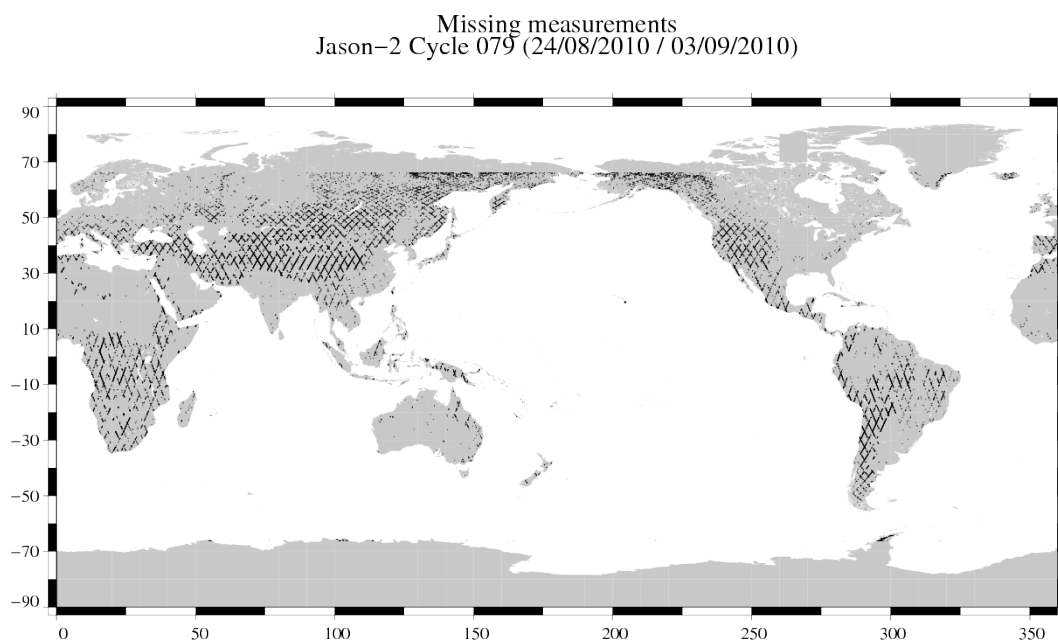
FIG. 1 – Missing measurements for cycle 079.
