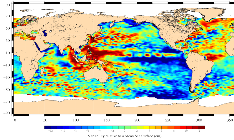
FIG. 18 – Sea level anomaly relative to MSS for cycle 079.
