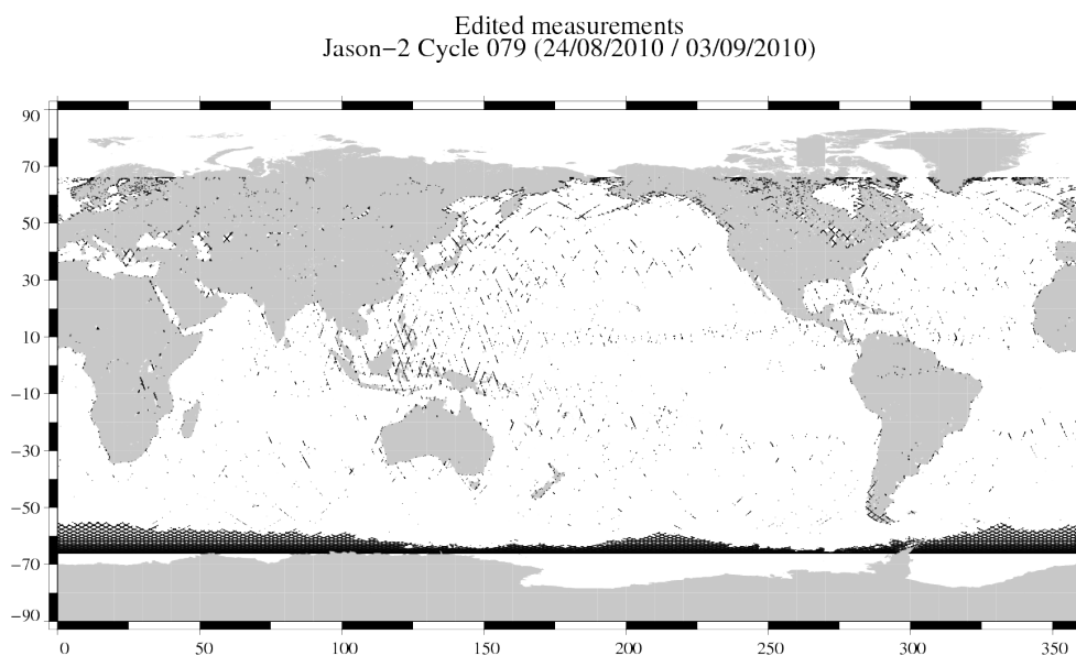
FIG. 2 – Edited measurements for cycle 079.
