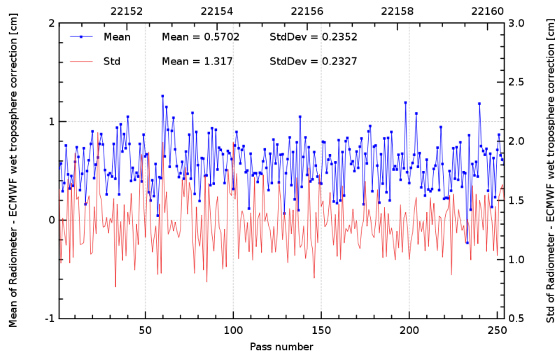
FIG. 11 – Pass monitoring of wet troposphere differences between radiometer and ECMWF model for Jason-2 cycle 079.
