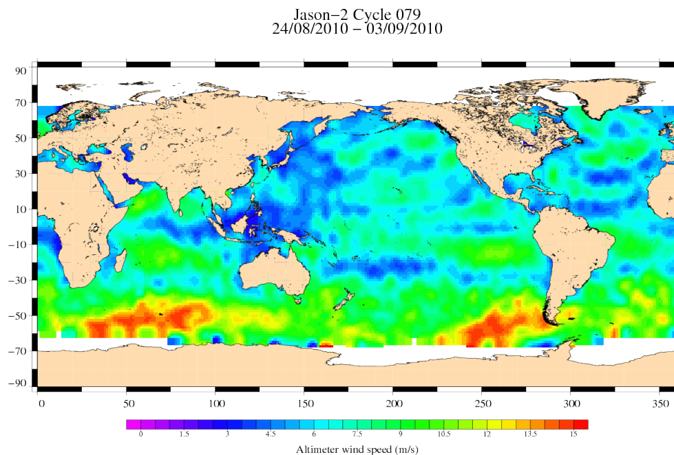
FIG. 9 – Altimeter wind speed for cycle 079.
