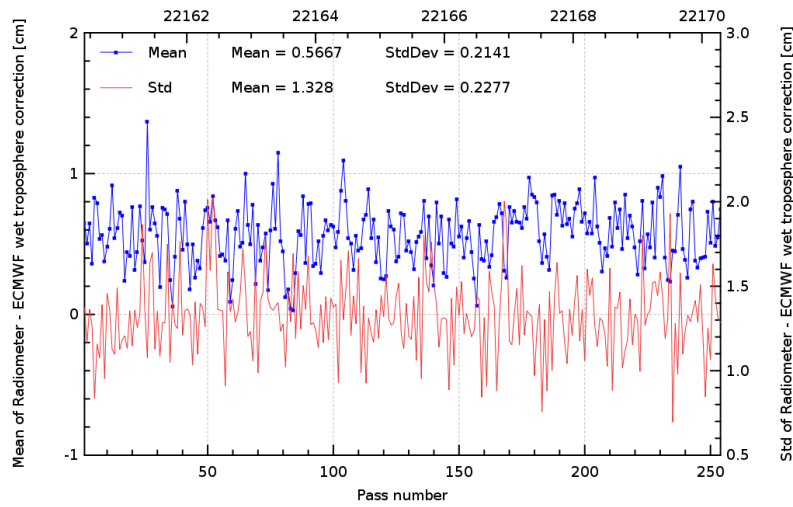
FIG. 11 – Pass monitoring of wet troposphere differences between radiometer and ECMWF model for Jason-2 cycle 080.
