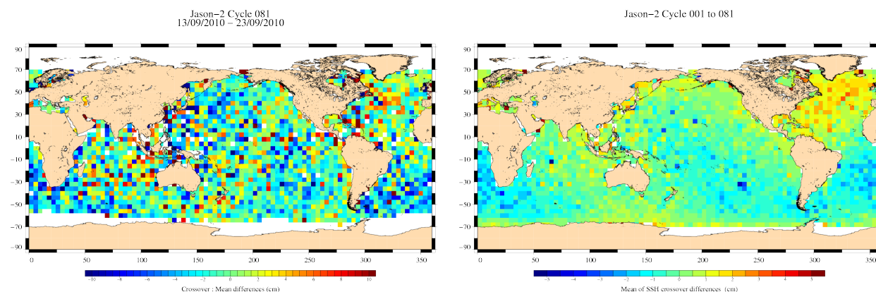
FIG. 13 – Mean SSH at crossovers for cycle 081 (left) and over the whole Jason-2 period (right).
