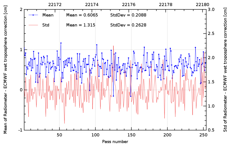
FIG. 11 – Pass monitoring of wet troposphere differences between radiometer and ECMWF model for Jason-2 cycle 081.
