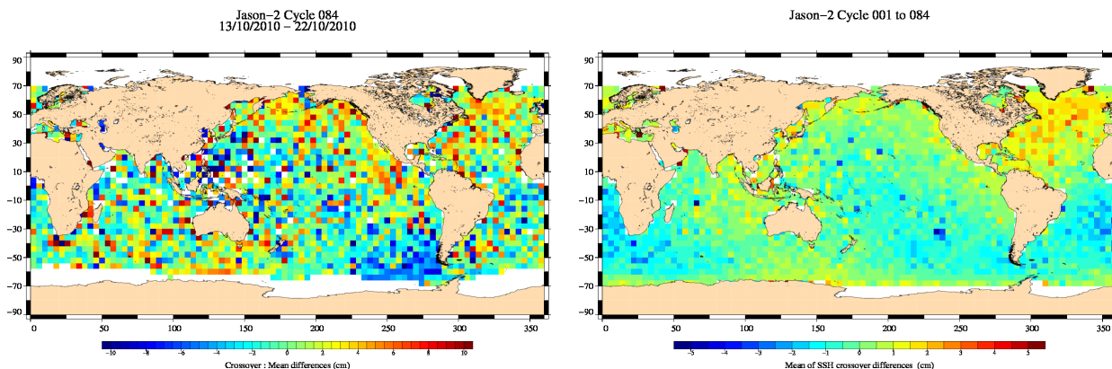
FIG. 13 – Mean SSH at crossovers for cycle 084 (left) and over the whole Jason-2 period (right).
