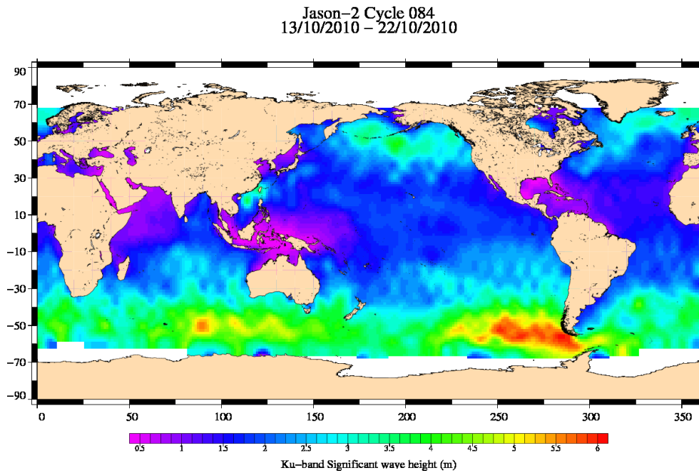
FIG. 5 – Significant wave height for cycle 084.
