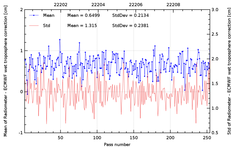
FIG. 11 – Pass monitoring of wet troposphere differences between radiometer and ECMWF model for Jason-2 cycle 084.
