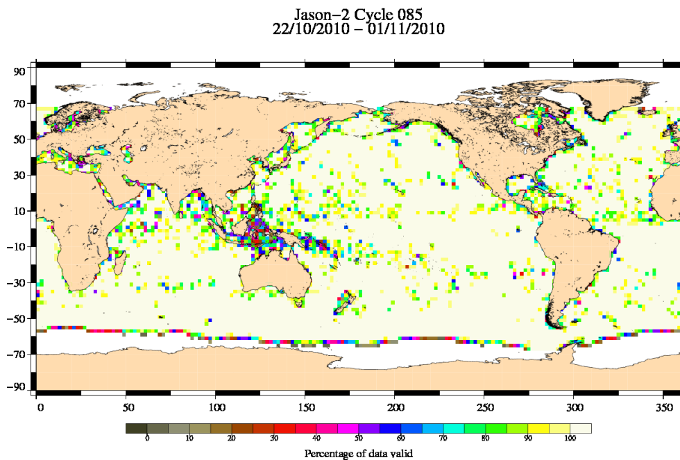
FIG. 3 – Percentage of valid measurements for cycle 085.
