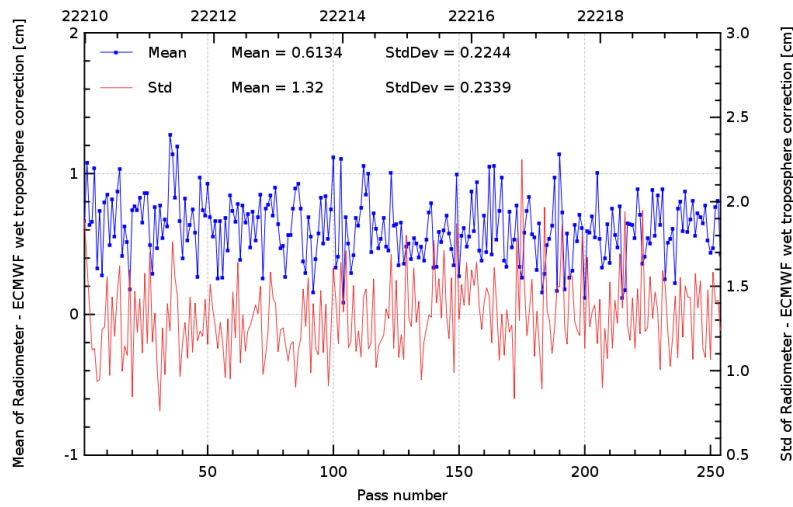
FIG. 11 – Pass monitoring of wet troposphere differences between radiometer and ECMWF model for Jason-2 cycle 085.
