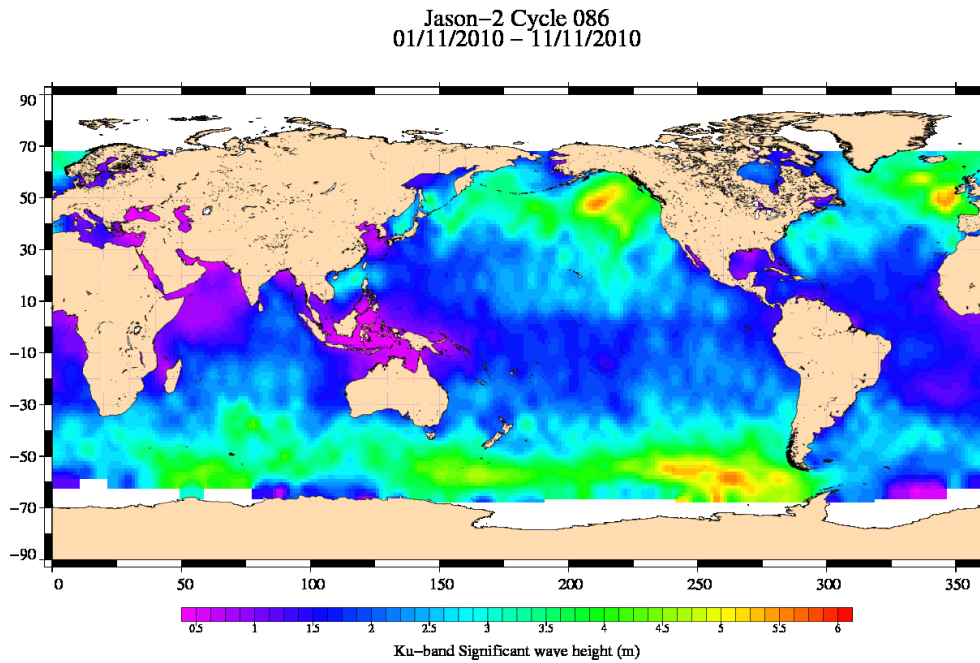
FIG. 5 – Significant wave height for cycle 086.
