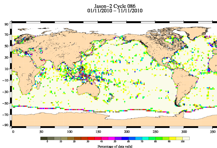
FIG. 3 – Percentage of valid measurements for cycle 086.
