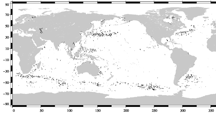
Valid data: (SSH – MSS) differences greater than 30 cm Jason-2 Cycle 086 (01/11/2010 / 11/11/2010)
