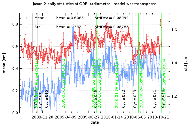
FIG. 13 – Daily monitoring of wet troposphere differences (mean and std) between radiometer and ECMWF model
