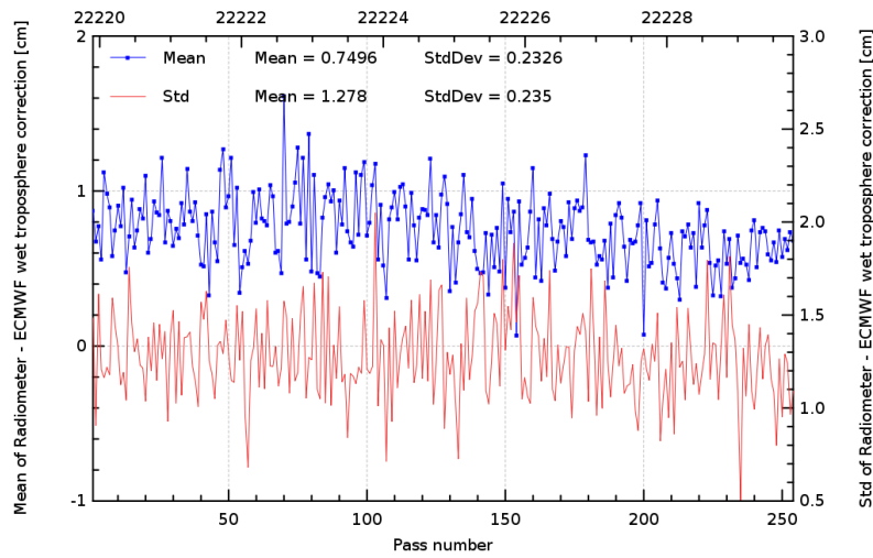
FIG. 11 – Pass monitoring of wet troposphere differences between radiometer and ECMWF model for Jason-2 cycle 086.
