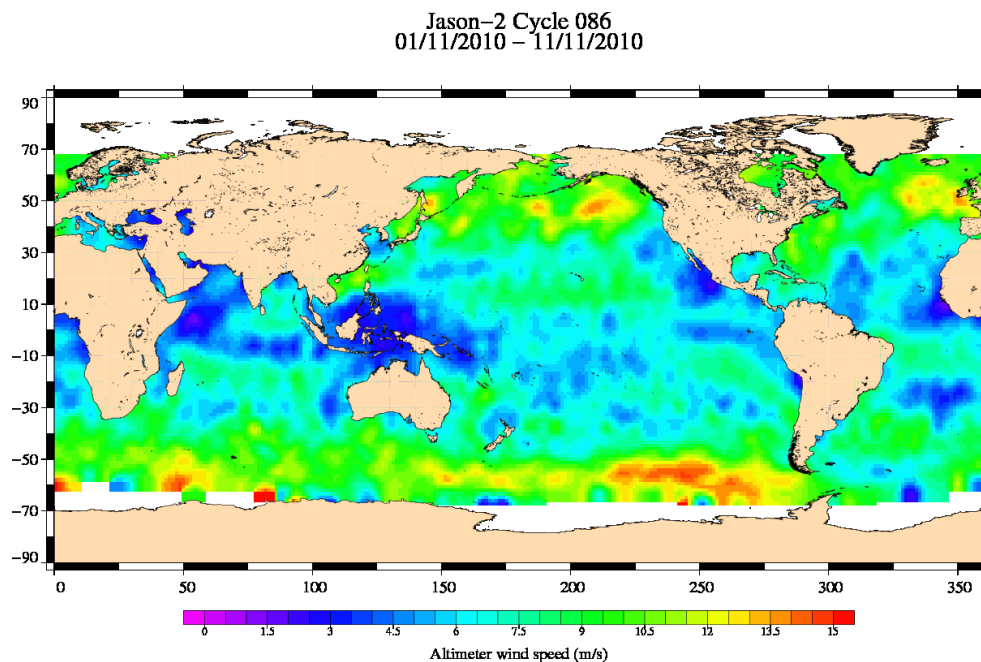
FIG. 9 – Altimeter wind speed for cycle 086.
