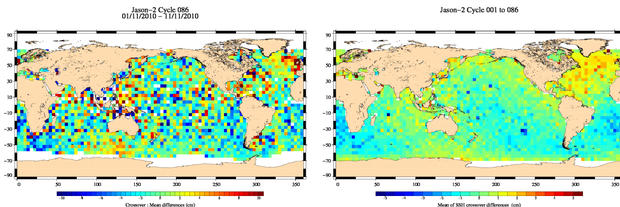
FIG. 14 – Mean SSH at crossovers for cycle 086 (left) and over the whole Jason-2 period (right).
