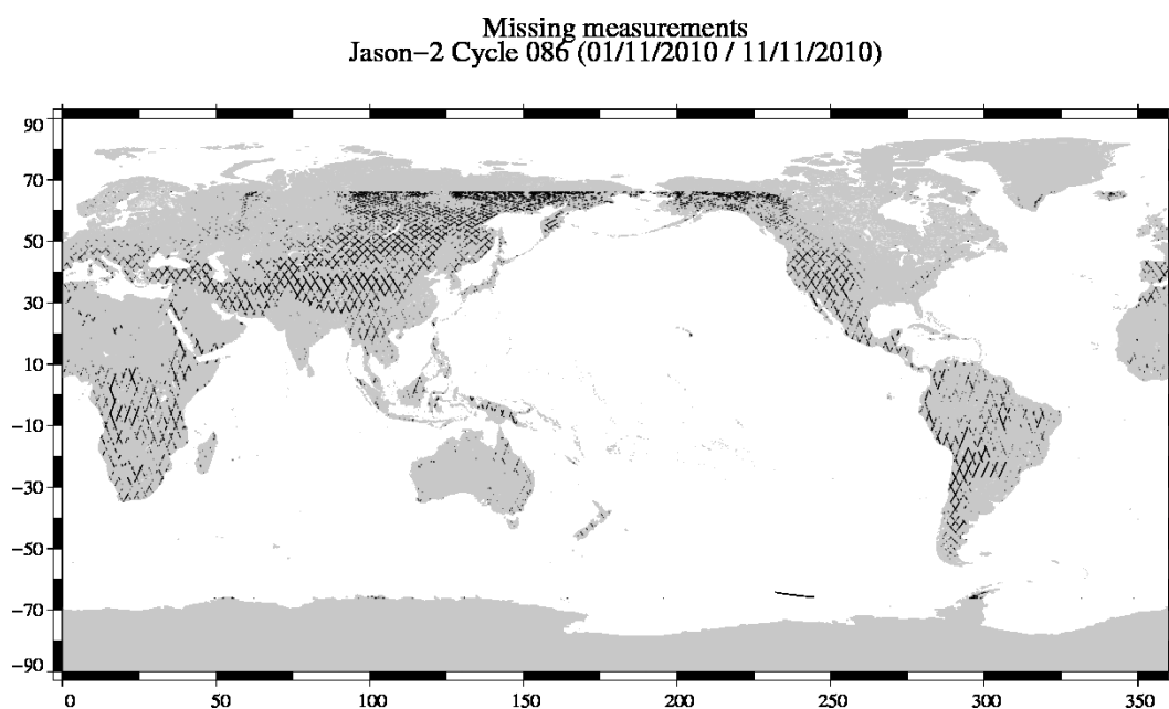
FIG. 1 – Missing measurements for cycle 086.
