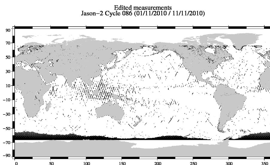
FIG. 2 – Edited measurements for cycle 086.
