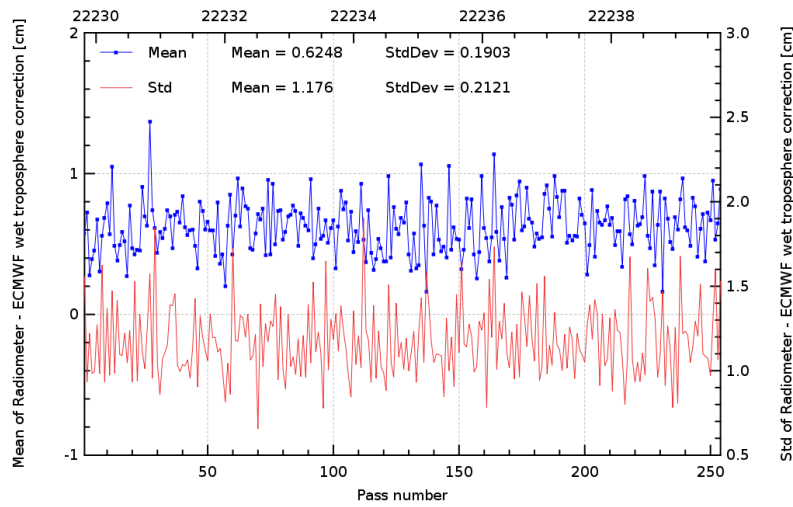
FIG. 11 – Pass monitoring of wet troposphere differences between radiometer and ECMWF model for Jason-2 cycle 087.
