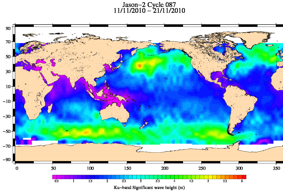
FIG. 5 – Significant wave height for cycle 087.
