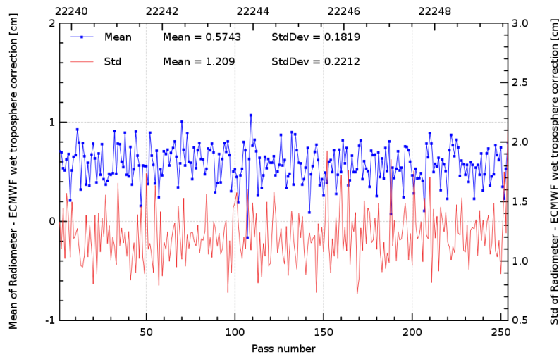
FIG. 11 – Pass monitoring of wet troposphere differences between radiometer and ECMWF model for Jason-2 cycle 088.
