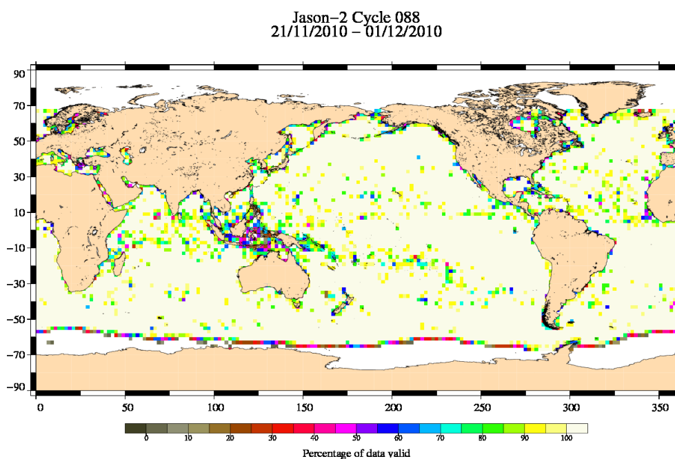
FIG. 3 – Percentage of valid measurements for cycle 088.
