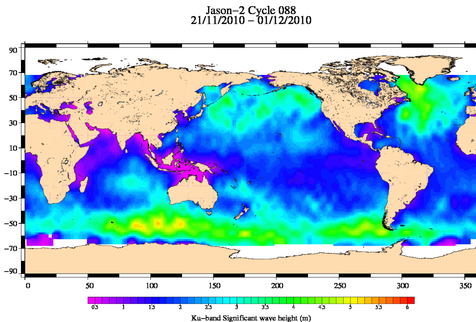
FIG. 5 – Significant wave height for cycle 088.
