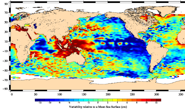
FIG. 18 – Sea level anomaly relative to MSS for cycle 088.
