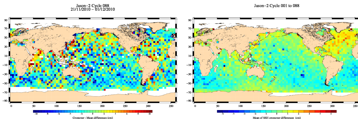
FIG. 13 – Mean SSH at crossovers for cycle 088 (left) and over the whole Jason-2 period (right).
