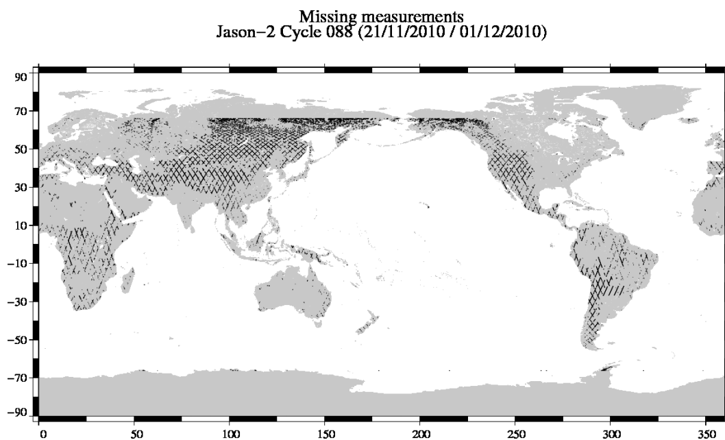
FIG. 1 – Missing measurements for cycle 088.
