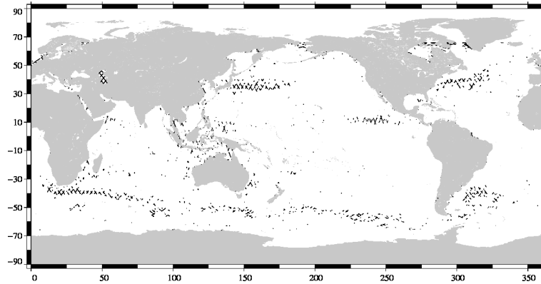
FIG. 19 – Differences higher than a 30 cm threshold for cycle 088.
