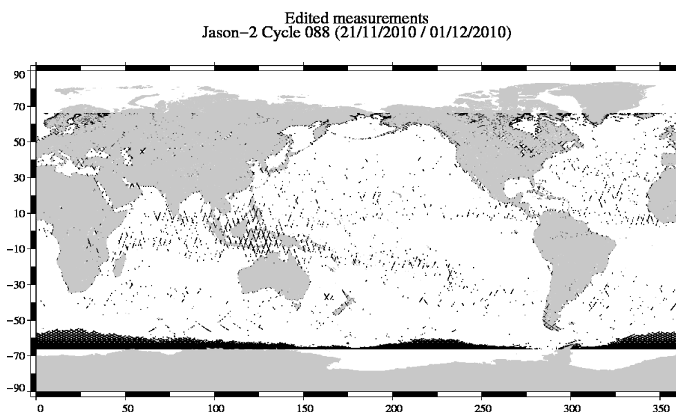
FIG. 2 – Edited measurements for cycle 088.
