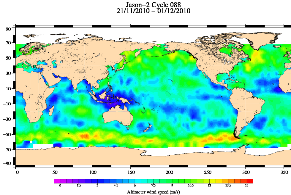
FIG. 9 – Altimeter wind speed for cycle 088.
