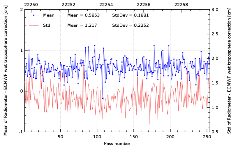
FIG. 11 – Pass monitoring of wet troposphere differences between radiometer and ECMWF model for Jason-2 cycle 089.
