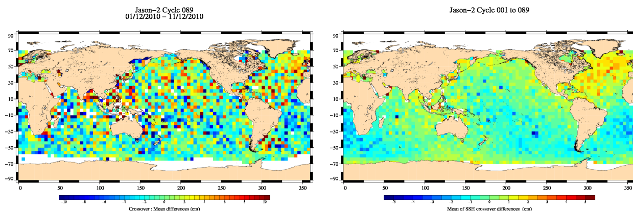
FIG. 13 – Mean SSH at crossovers for cycle 089 (left) and over the whole Jason-2 period (right).
