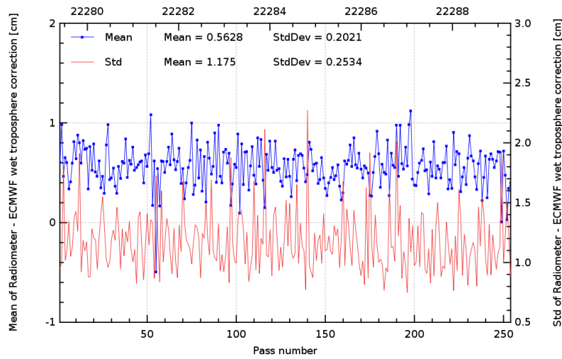
FIG. 11 – Pass monitoring of wet troposphere differences between radiometer and ECMWF model for Jason-2 cycle 092.
