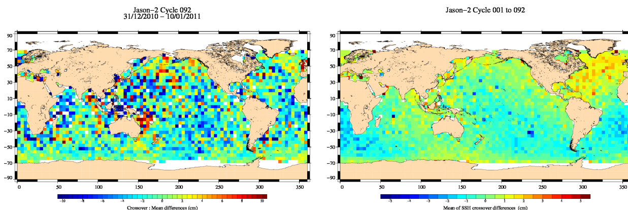
FIG. 13 – Mean SSH at crossovers for cycle 092 (left) and over the whole Jason-2 period (right).
