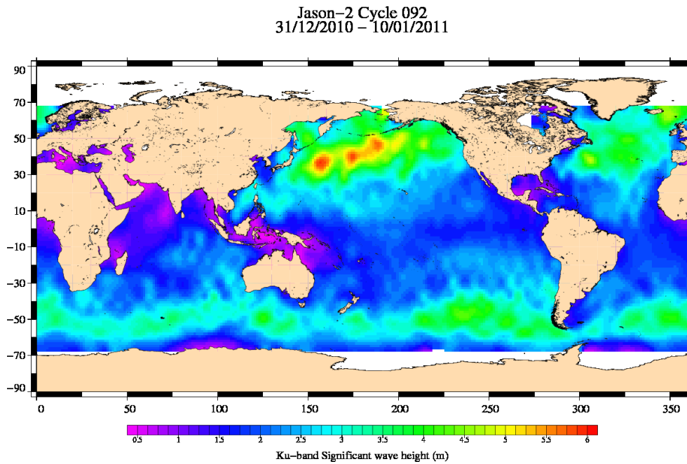
FIG. 5 – Significant wave height for cycle 092.
