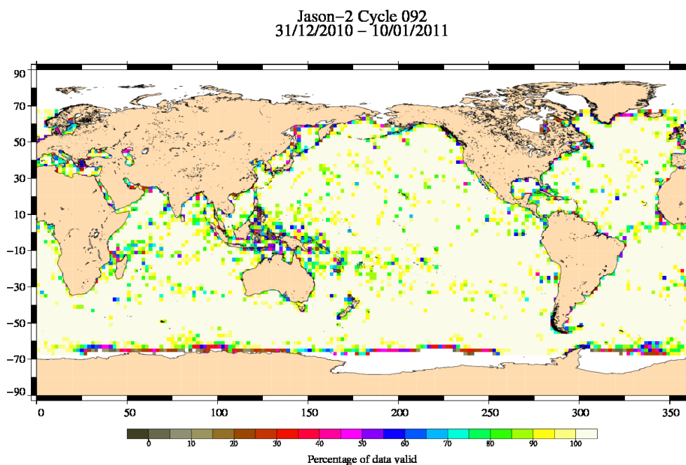
FIG. 3 – Percentage of valid measurements for cycle 092.
