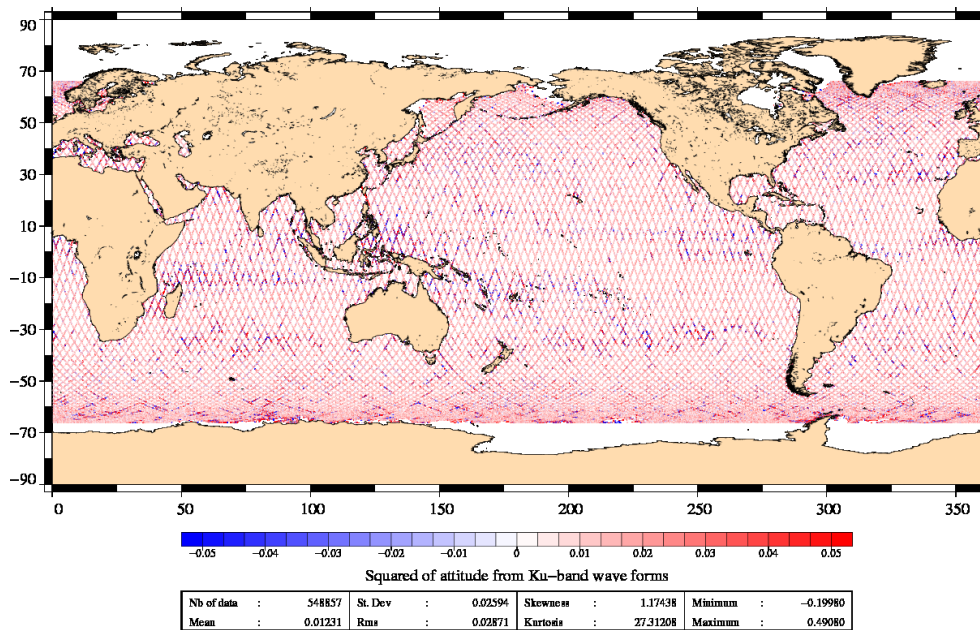
FIG. 4 – Apparent squared mispointing from waveforms for cycle 093.
