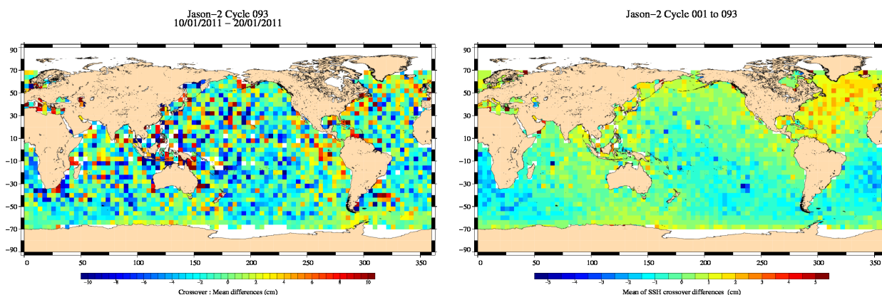
FIG. 14 – Mean SSH at crossovers for cycle 093 (left) and over the whole Jason-2 period (right).
