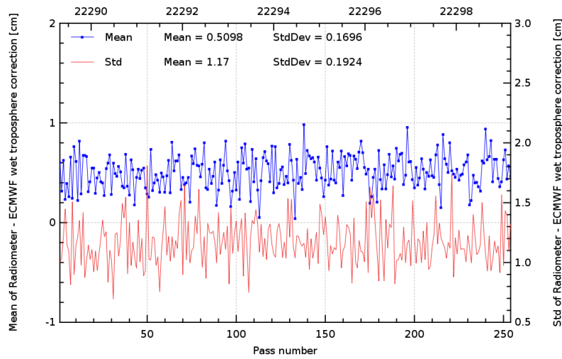
FIG. 12 – Pass monitoring of wet troposphere differences between radiometer and ECMWF model for Jason-2 cycle 093.
