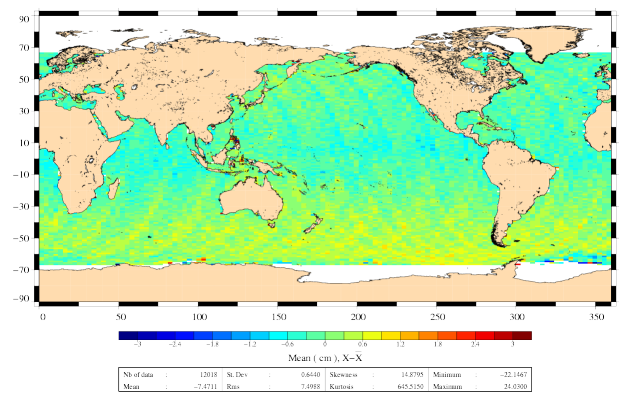
Differences of SLA before orbit error correction Jason-1 – Jason-2 (Cycle 001 – 020)
