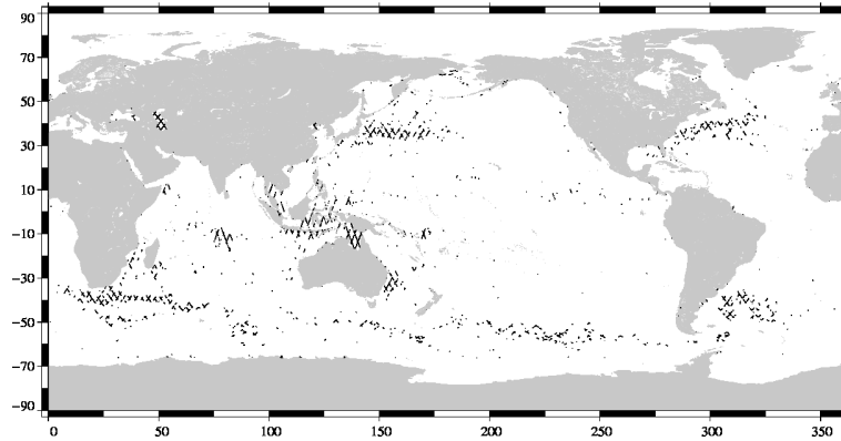
Valid data: (SSH – MSS) differences greater than 30 cm Jason-2 Cycle 093 (10/01/2011 / 20/01/2011)
