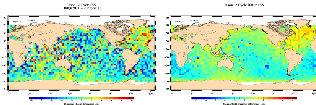
FIG. 13 – Mean SSH at crossovers for cycle 099 (left) and over the whole Jason-2 period (right).
