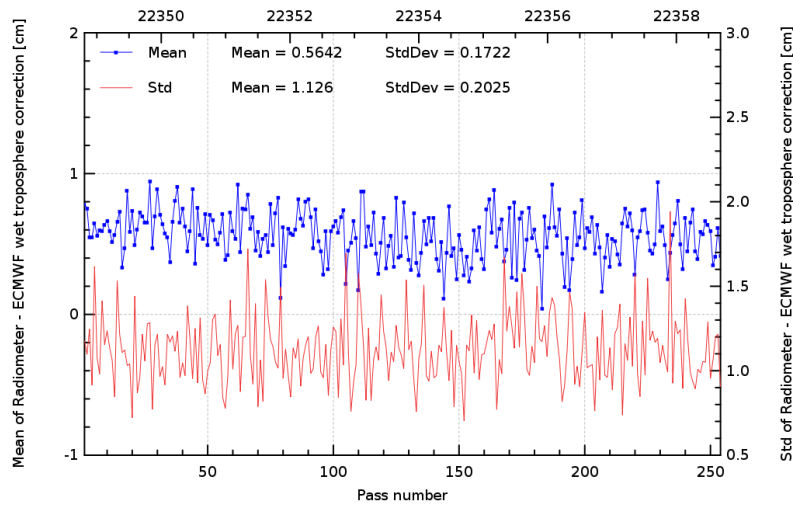
FIG. 11 – Pass monitoring of wet troposphere differences between radiometer and ECMWF model for Jason-2 cycle 099.
