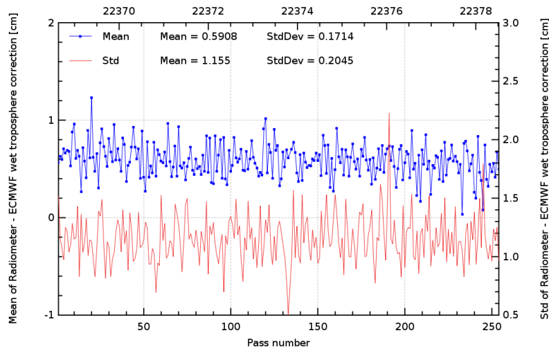
FIG. 11 – Pass monitoring of wet troposphere differences between radiometer and ECMWF model for Jason-2 cycle 101.
