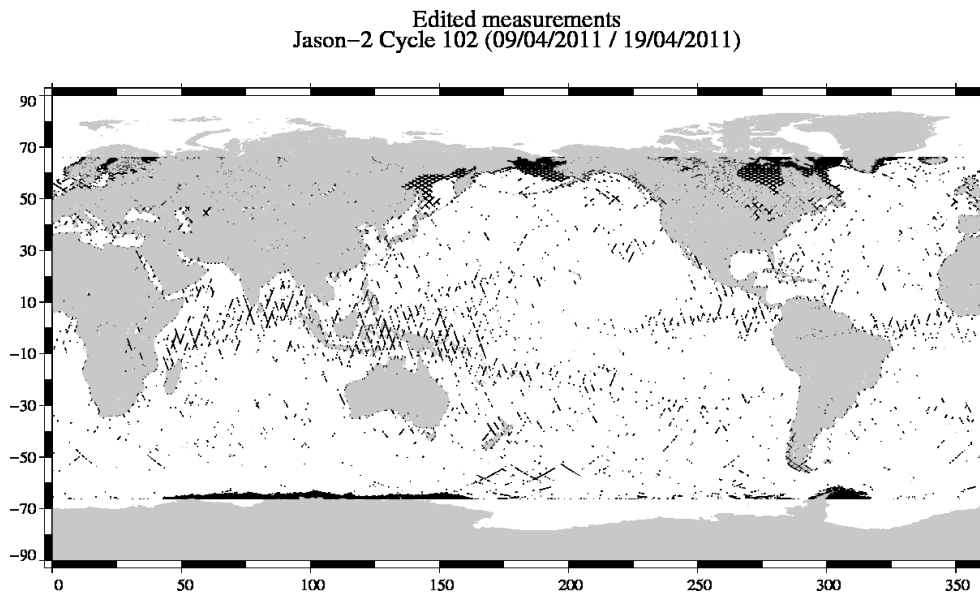
FIG. 2 – Edited measurements for cycle 102.
