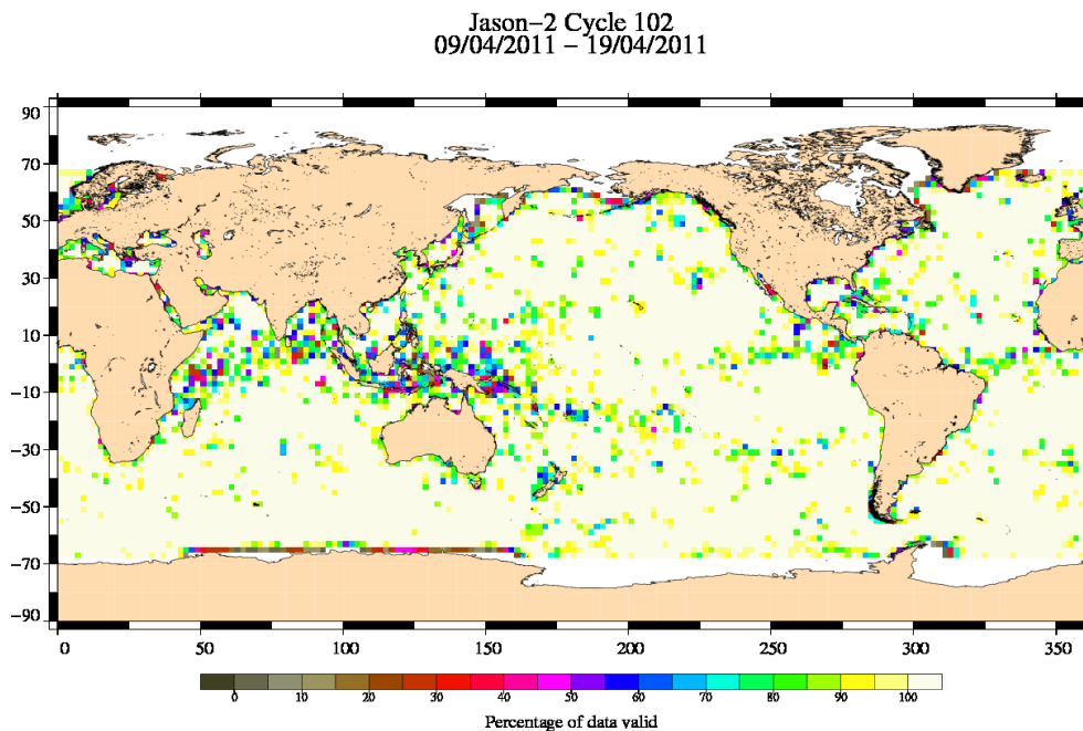
FIG. 3 – Percentage of valid measurements for cycle 102.
