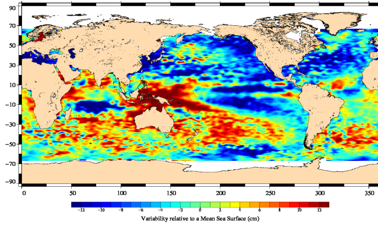
Jason-2 Cycle 102 09/04/2011 - 19/04/2011
