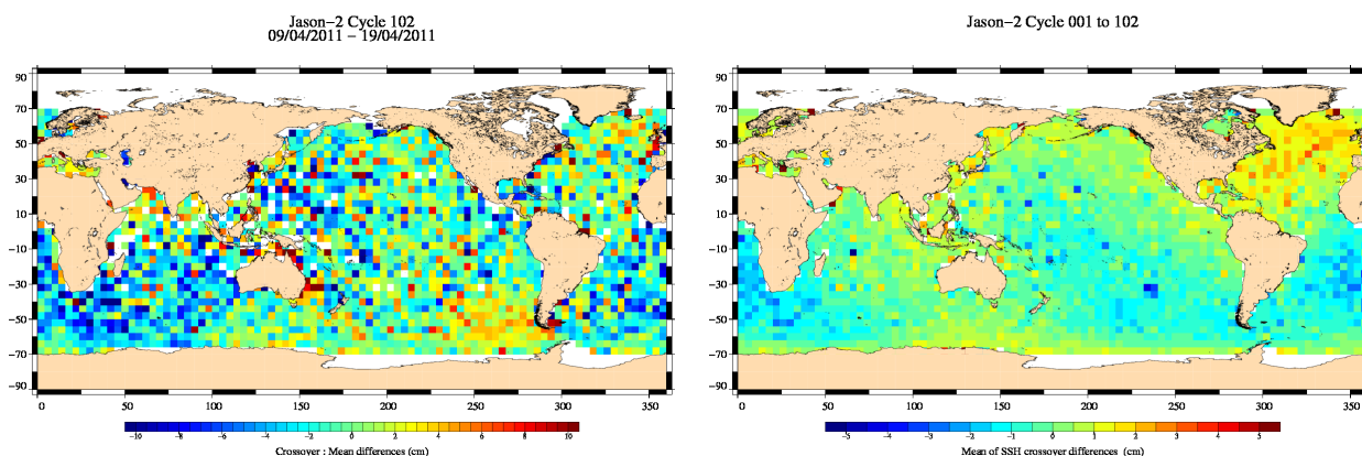
FIG. 13 – Mean SSH at crossovers for cycle 102 (left) and over the whole Jason-2 period (right).
