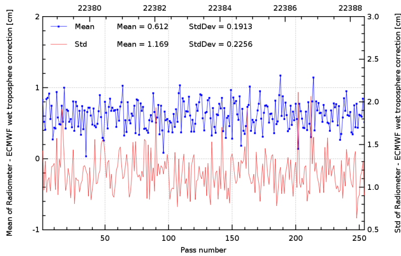
FIG. 11 – Pass monitoring of wet troposphere differences between radiometer and ECMWF model for Jason-2 cycle 102.
