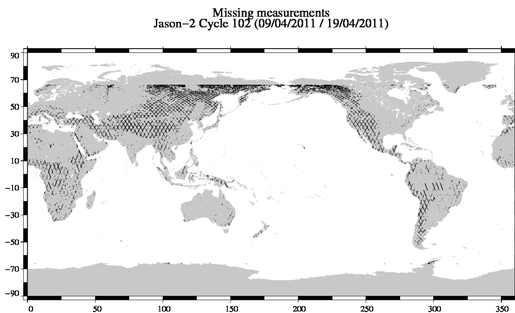
FIG. 1 – Missing measurements for cycle 102.
