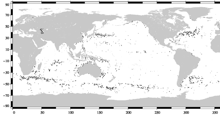
Valid data: (SSH – MSS) differences greater than 30 cm Jason-2 Cycle 102 (09/04/2011 / 19/04/2011)
