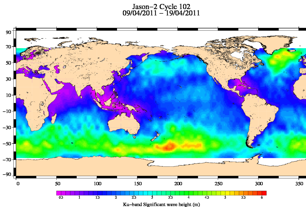
FIG. 5 – Significant wave height for cycle 102.
