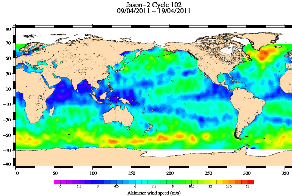
FIG. 9 – Altimeter wind speed for cycle 102.
