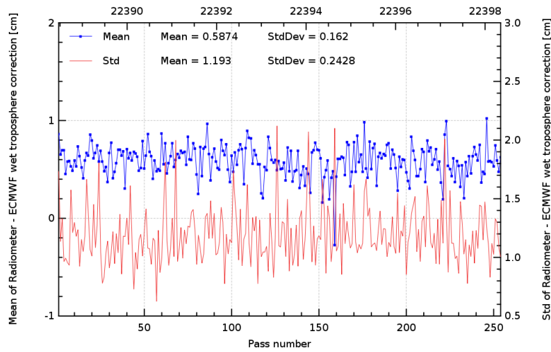
FIG. 11 – Pass monitoring of wet troposphere differences between radiometer and ECMWF model for Jason-2 cycle 103.
