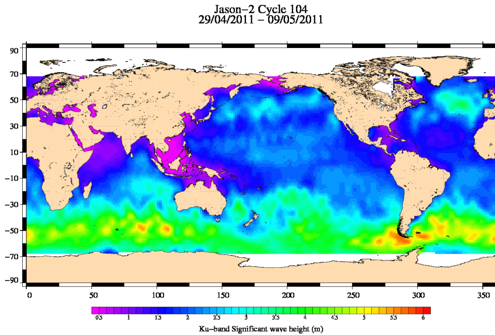
FIG. 5 – Significant wave height for cycle 104.
