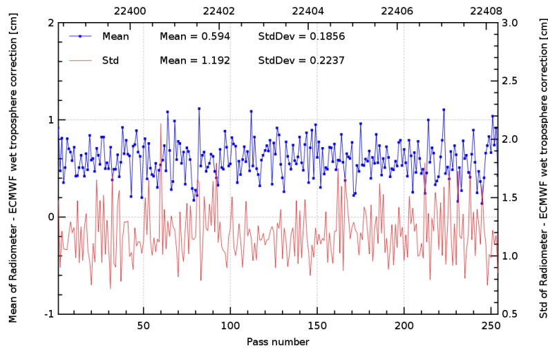
FIG. 11 – Pass monitoring of wet troposphere differences between radiometer and ECMWF model for Jason-2 cycle 104.
