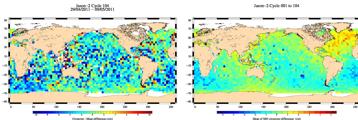
FIG. 13 – Mean SSH at crossovers for cycle 104 (left) and over the whole Jason-2 period (right).
