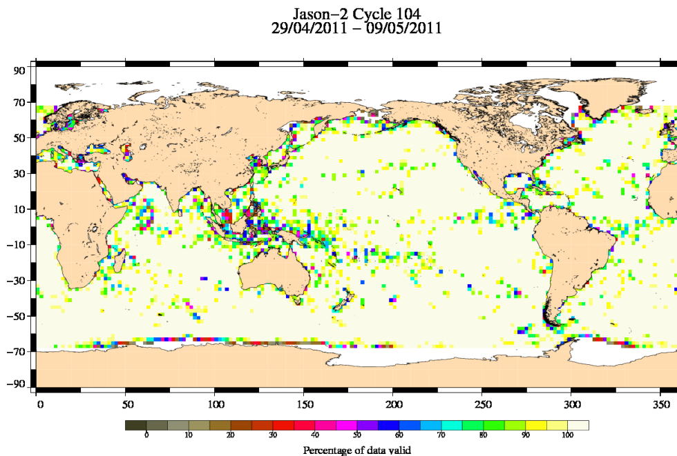
FIG. 3 – Percentage of valid measurements for cycle 104.
