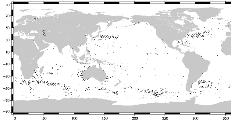
FIG. 19 – Differences higher than a 30 cm threshold for cycle 105.
