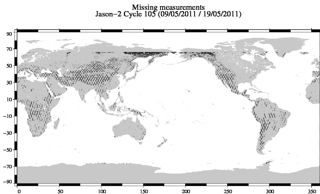
FIG. 1 – Missing measurements for cycle 105.
