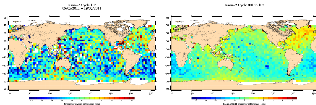
FIG. 13 – Mean SSH at crossovers for cycle 105 (left) and over the whole Jason-2 period (right).
