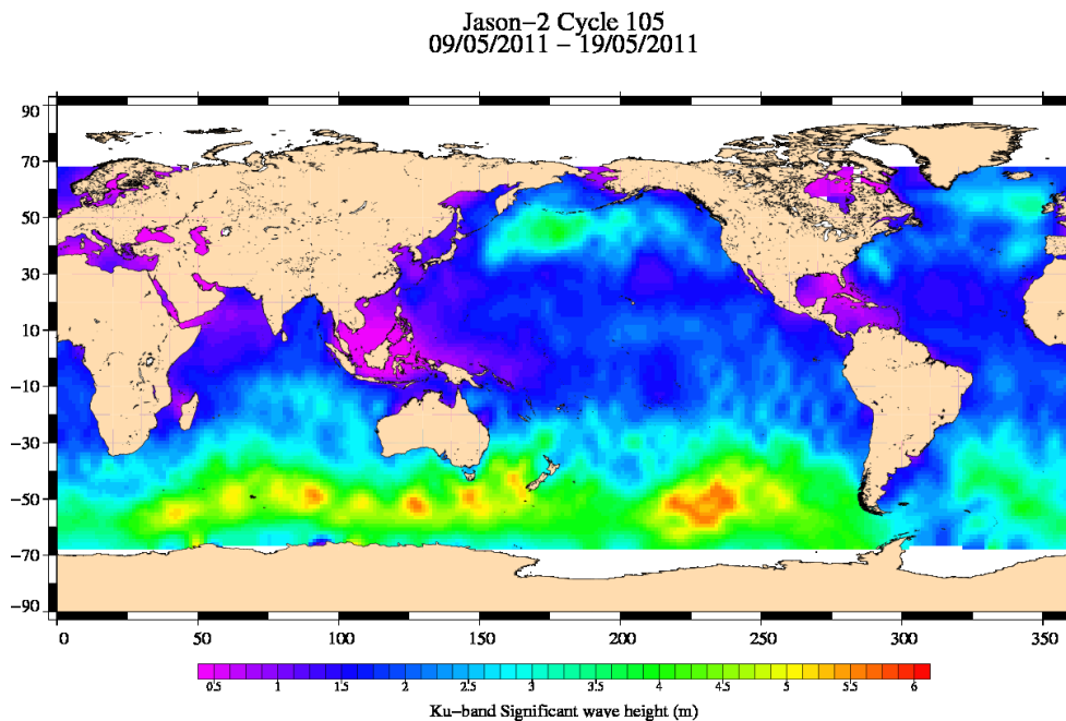
FIG. 5 – Significant wave height for cycle 105.
