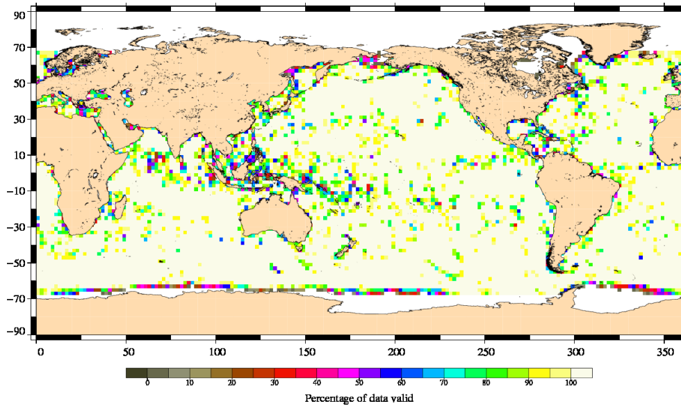
FIG. 3 – Percentage of valid measurements for cycle 105.
