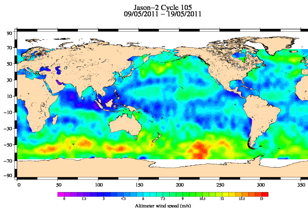
FIG. 9 – Altimeter wind speed for cycle 105.
