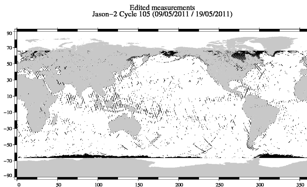
FIG. 2 – Edited measurements for cycle 105.
