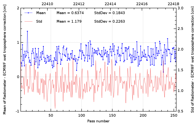
FIG. 11 – Pass monitoring of wet troposphere differences between radiometer and ECMWF model for Jason-2 cycle 105.
