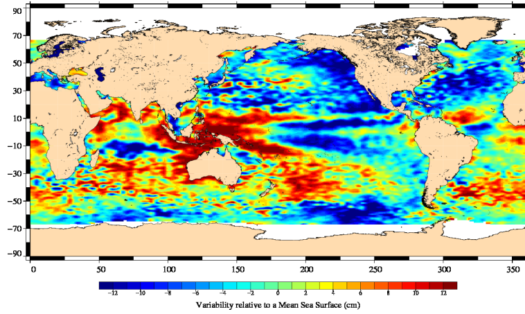
FIG. 18 – Sea level anomaly relative to MSS for cycle 105.
