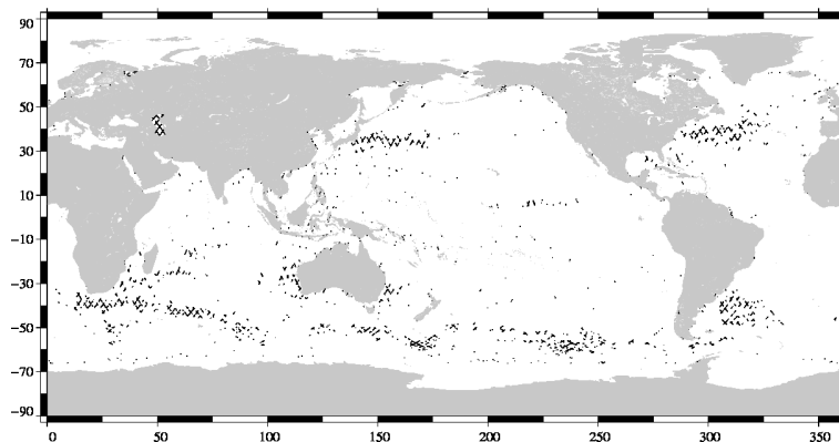
FIG. 20 – Differences higher than a 30 cm threshold for cycle 106.
