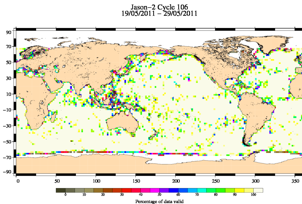
FIG. 3 – Percentage of valid measurements for cycle 106.
