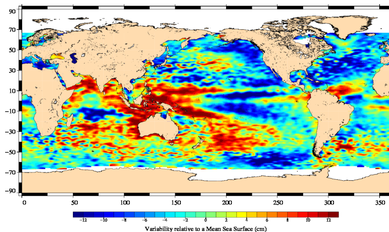
FIG. 19 – Sea level anomaly relative to MSS for cycle 106.
