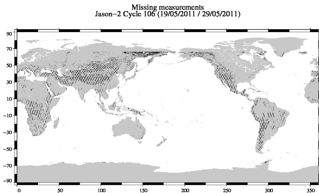
FIG. 1 – Missing measurements for cycle 106.
