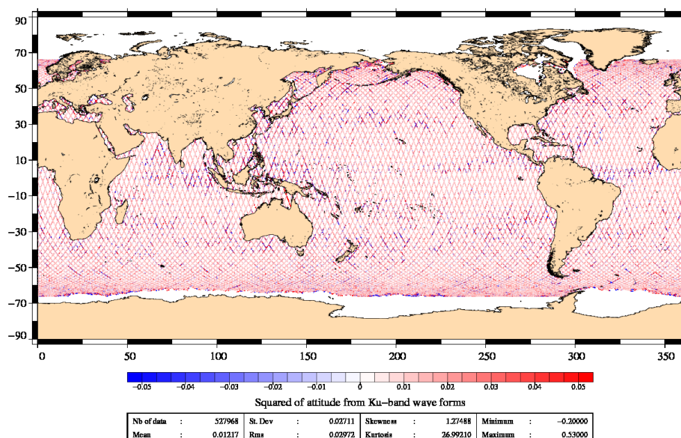
FIG. 4 – Apparent squared mispointing from waveforms for cycle 106.
