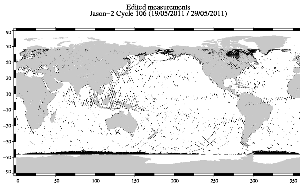
FIG. 2 – Edited measurements for cycle 106.
