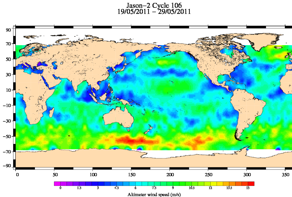
FIG. 10 – Altimeter wind speed for cycle 106.
