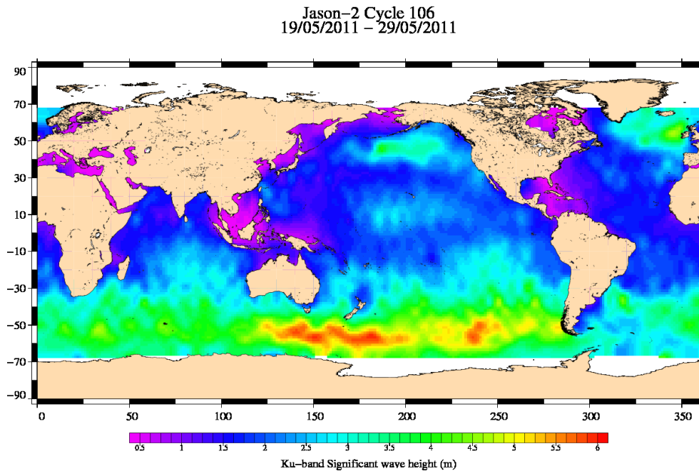
FIG. 6 – Significant wave height for cycle 106.
