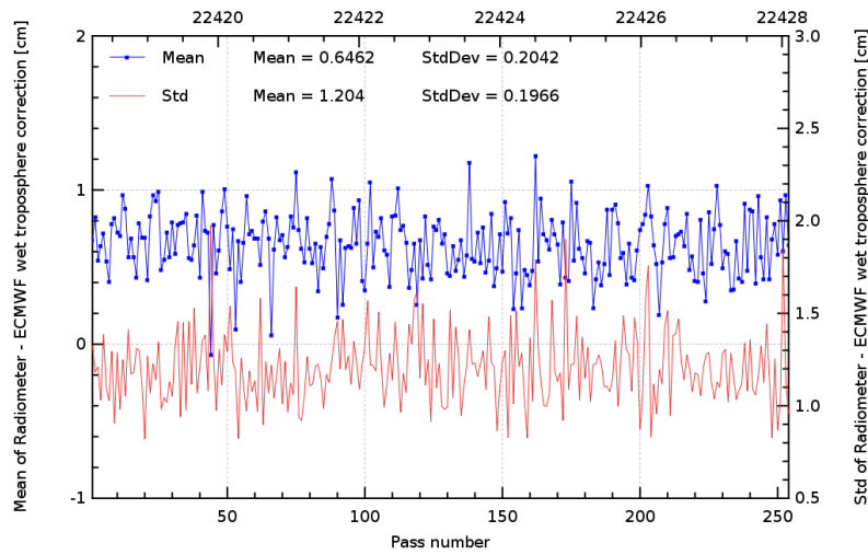
FIG. 12 – Pass monitoring of wet troposphere differences between radiometer and ECMWF model for Jason-2 cycle 106.
