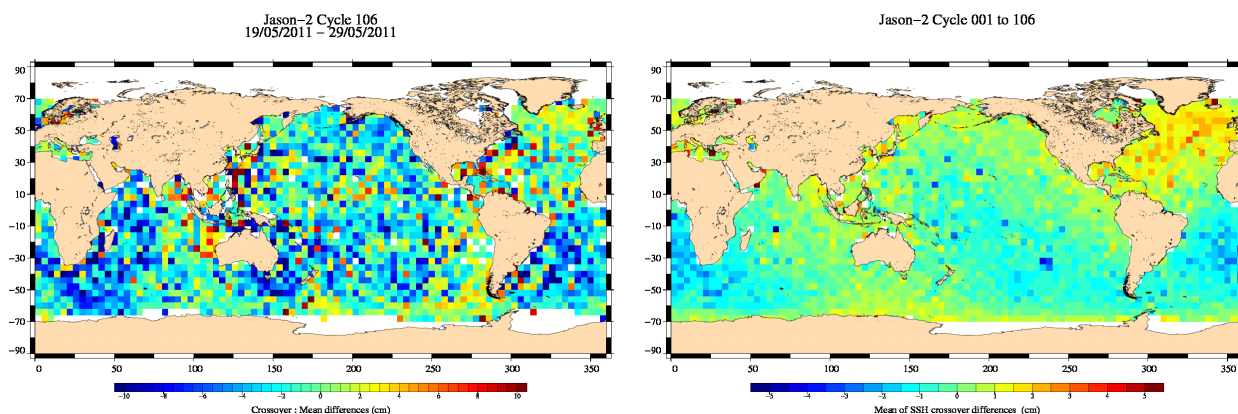
FIG. 14 – Mean SSH at crossovers for cycle 106 (left) and over the whole Jason-2 period (right).
