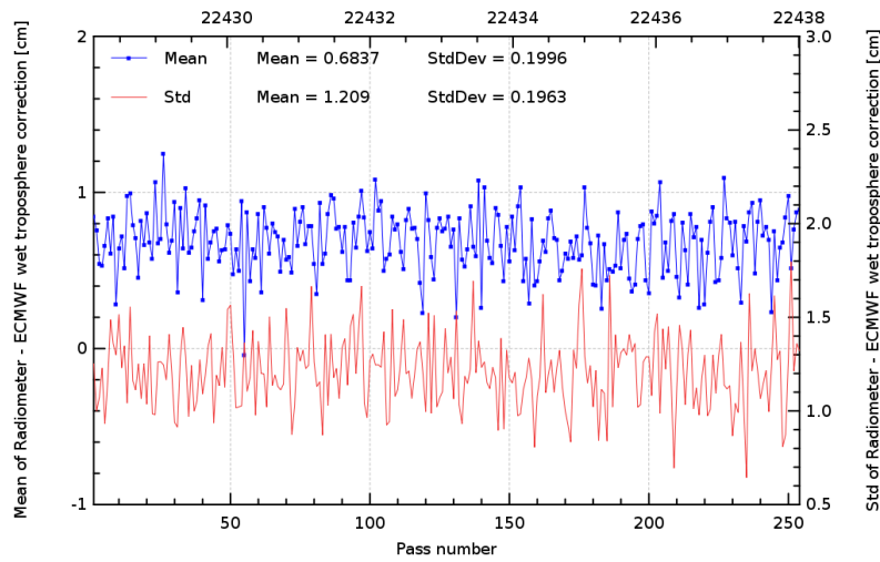
FIG. 11 – Pass monitoring of wet troposphere differences between radiometer and ECMWF model for Jason-2 cycle 107.
