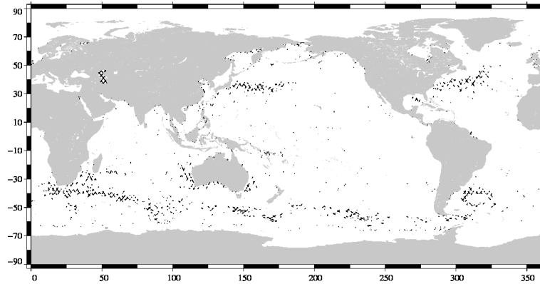
Valid data: (SSH – MSS) differences greater than 30 cm Jason-2 Cycle 109 (17/06/2011 / 27/06/2011)
