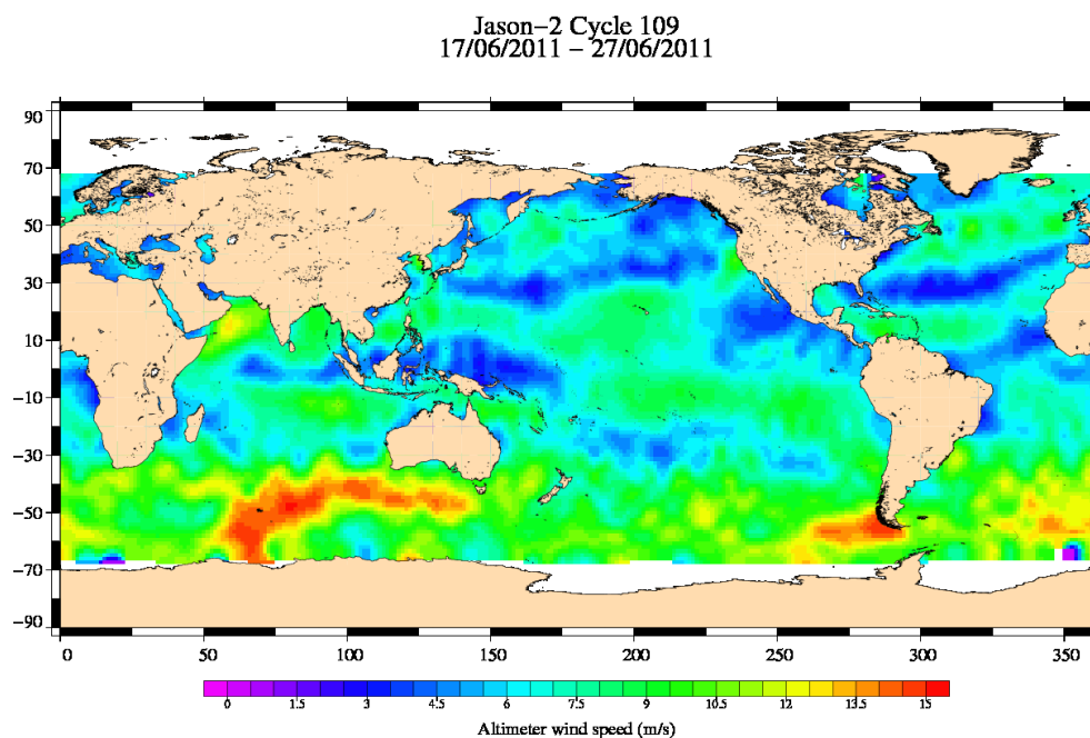
FIG. 9 – Altimeter wind speed for cycle 109.
