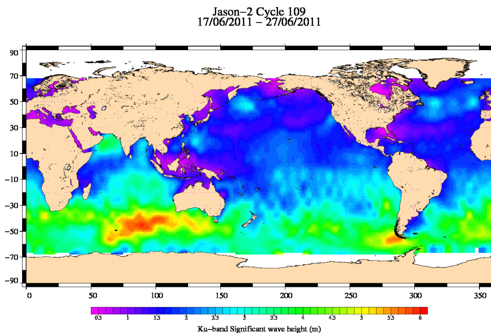
FIG. 5 – Significant wave height for cycle 109.
