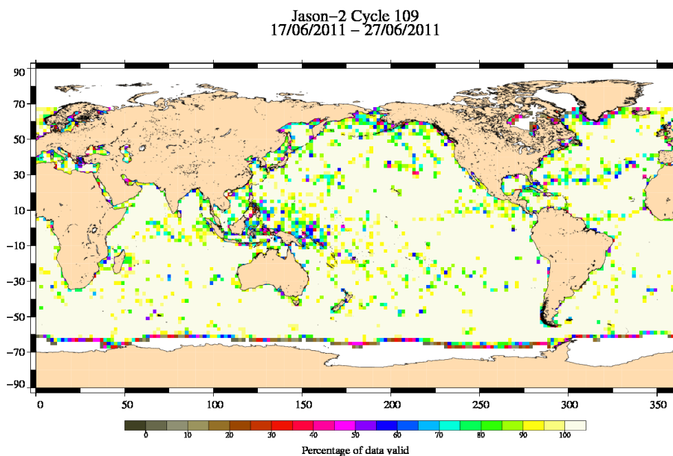
FIG. 3 – Percentage of valid measurements for cycle 109.
