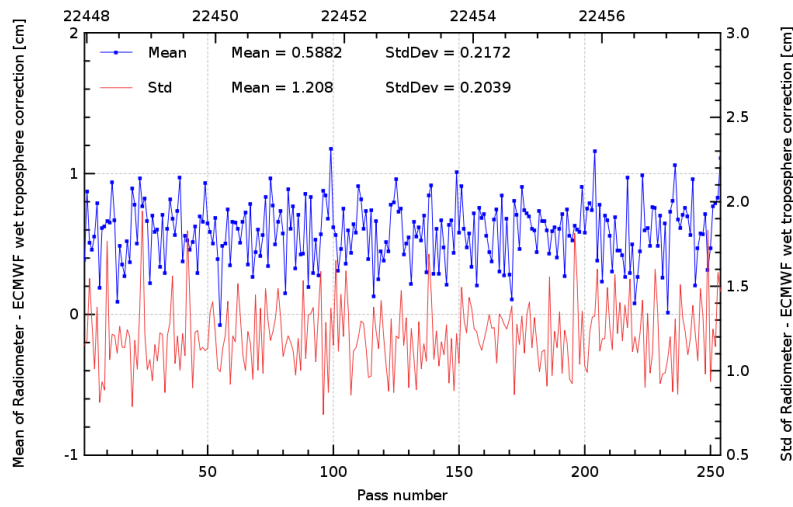
FIG. 11 – Pass monitoring of wet troposphere differences between radiometer and ECMWF model for Jason-2 cycle 109.
