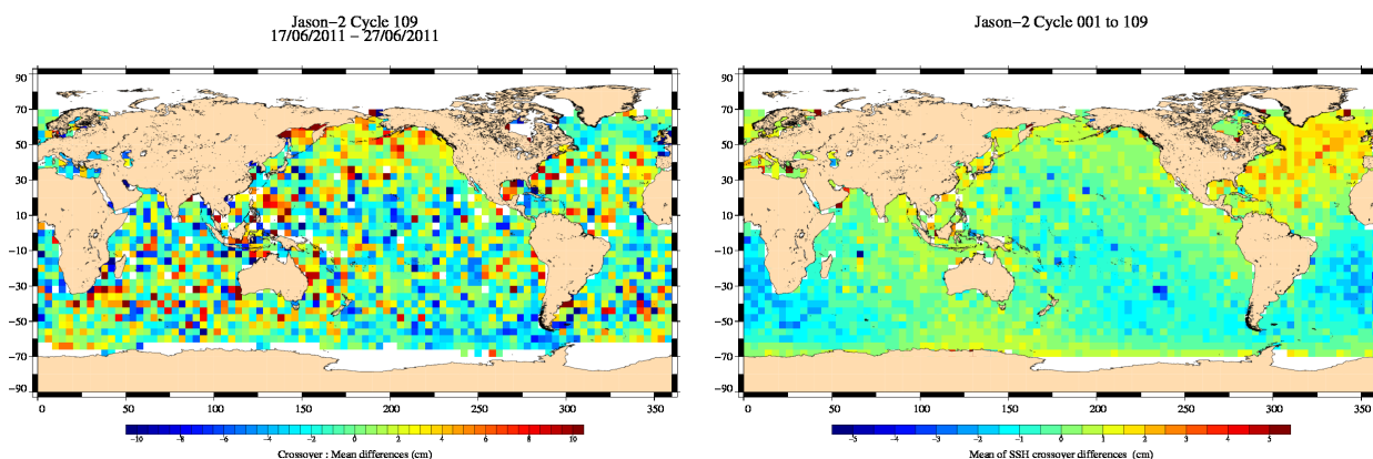
FIG. 13 – Mean SSH at crossovers for cycle 109 (left) and over the whole Jason-2 period (right).
