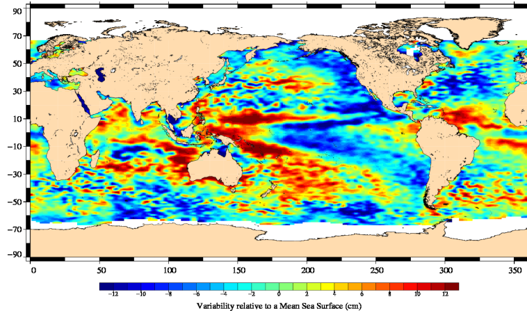
Jason-2 Cycle 109 17/06/2011 – 27/06/2011
