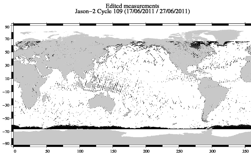
FIG. 2 – Edited measurements for cycle 109.
