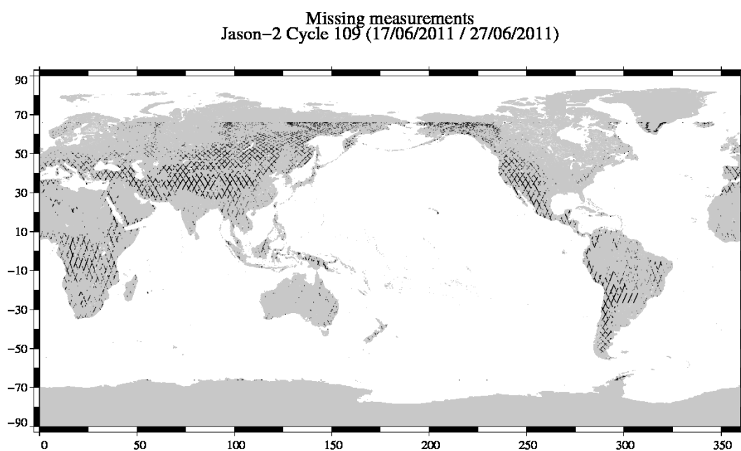
FIG. 1 – Missing measurements for cycle 109.
