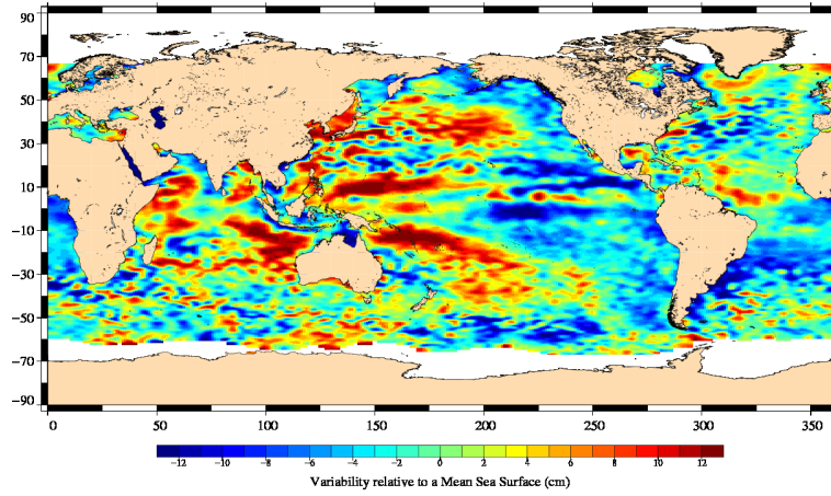
Jason-2 Cycle 114 06/08/2011 - 16/08/2011
