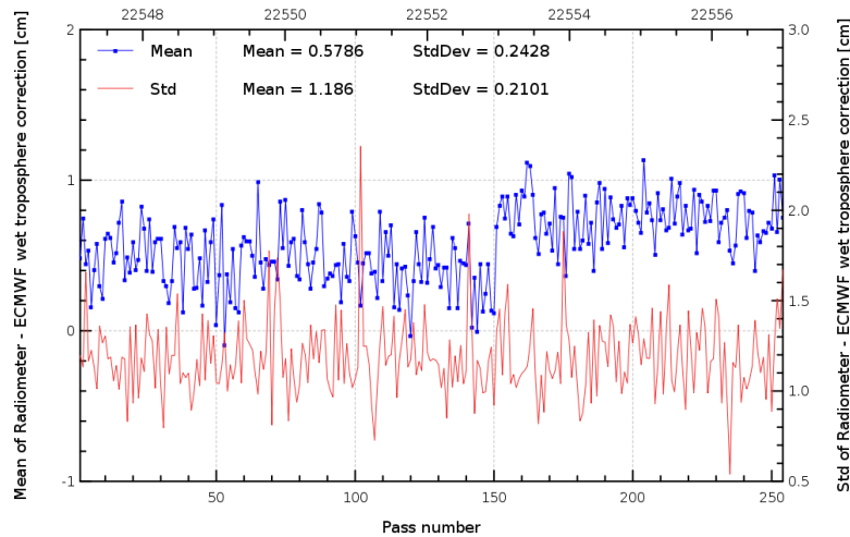
FIG. 11 – Pass monitoring of wet troposphere differences between radiometer and ECMWF model for Jason-2 cycle 119.
