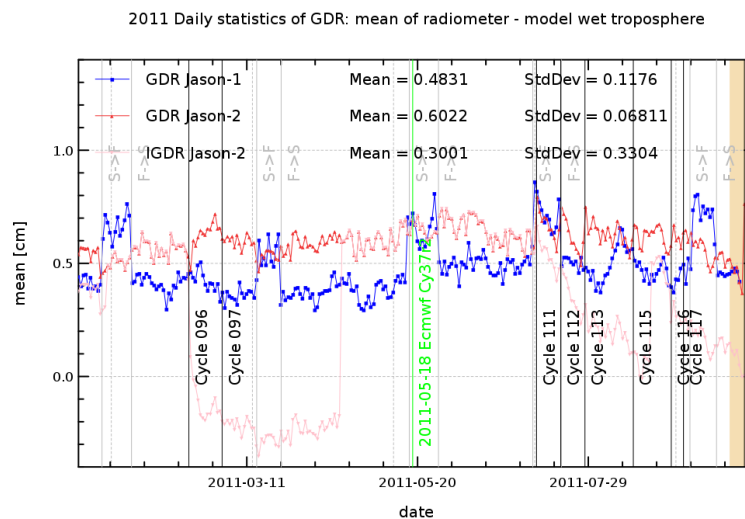
FIG. 13 – Daily monitoring of wet troposphere differences between radiometer and ECMWF model for year 2011.
