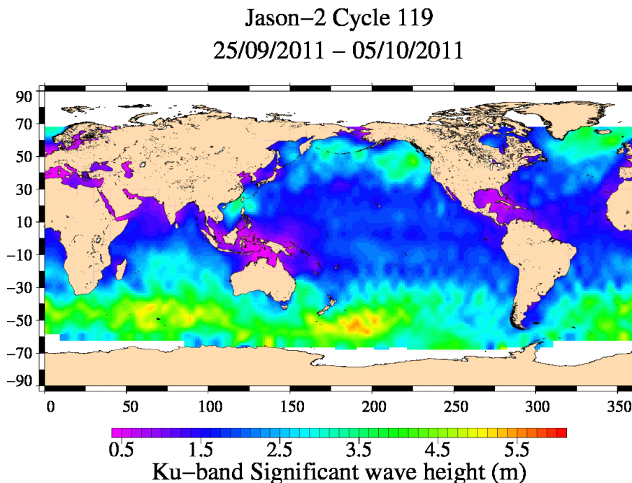
FIG. 5 – Significant wave height for cycle 119.
