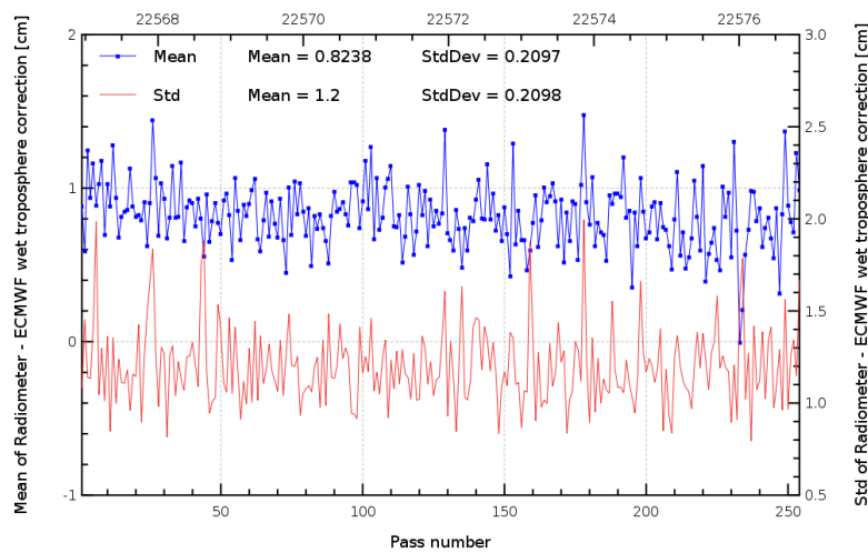
FIG. 11 – Pass monitoring of wet troposphere differences between radiometer and ECMWF model for Jason-2 cycle 121.
