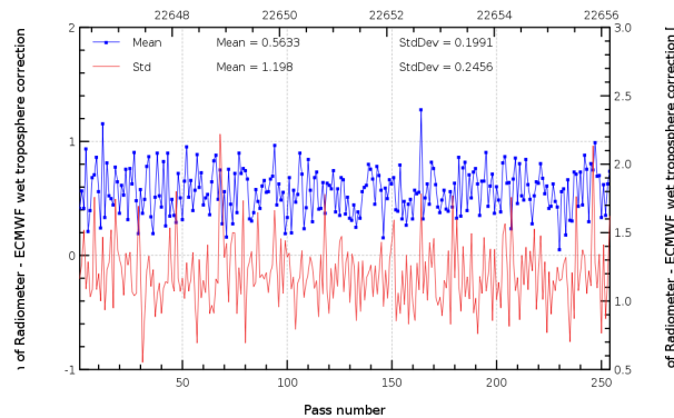
FIG. 12 – Pass monitoring of wet troposphere differences between radiometer and ECMWF model for Jason-2 cycle 129.
