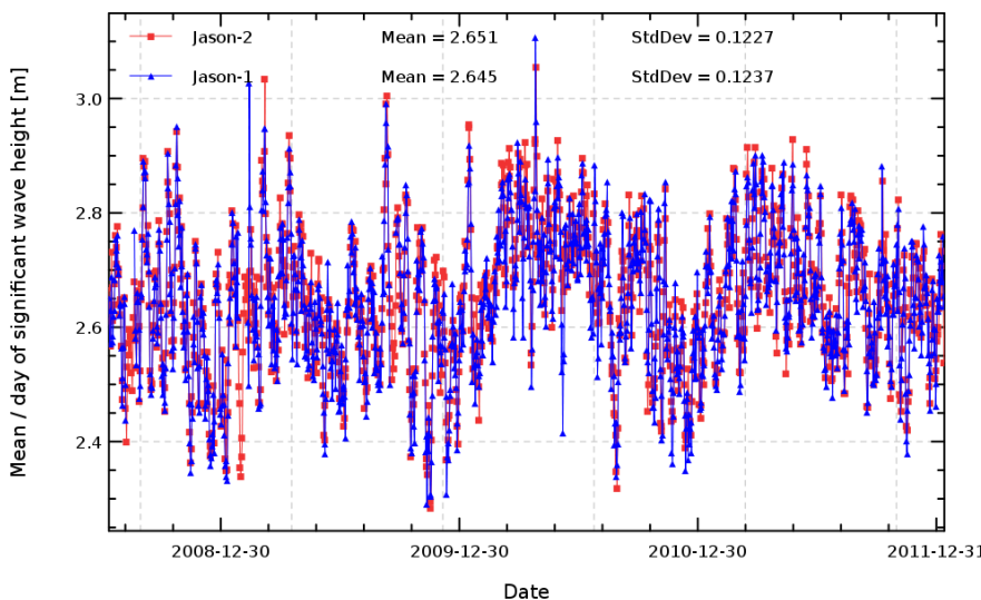
FIG. 7 – Daily monitoring of Ku-band significant wave height for Jason-2 and Jason-1.
