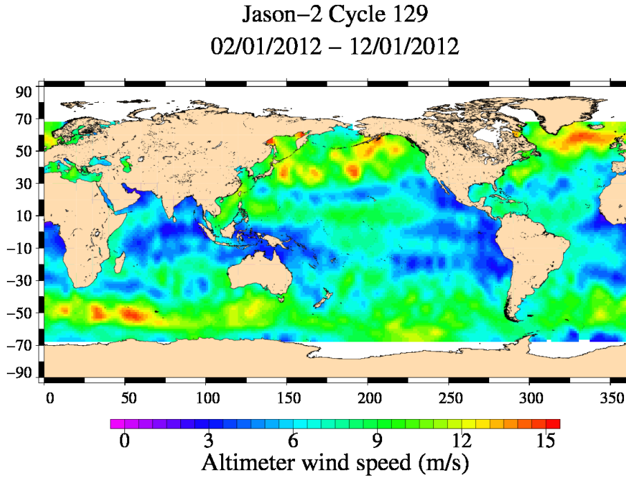
FIG. 10 – Altimeter wind speed for cycle 129.
