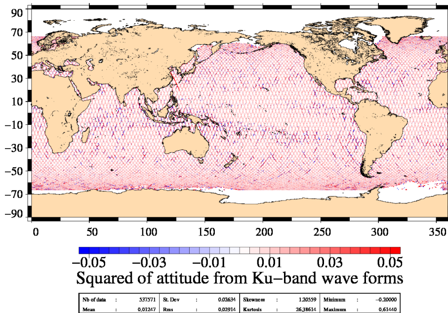
FIG. 4 – Apparent squared mispointing from waveforms for cycle 129.
