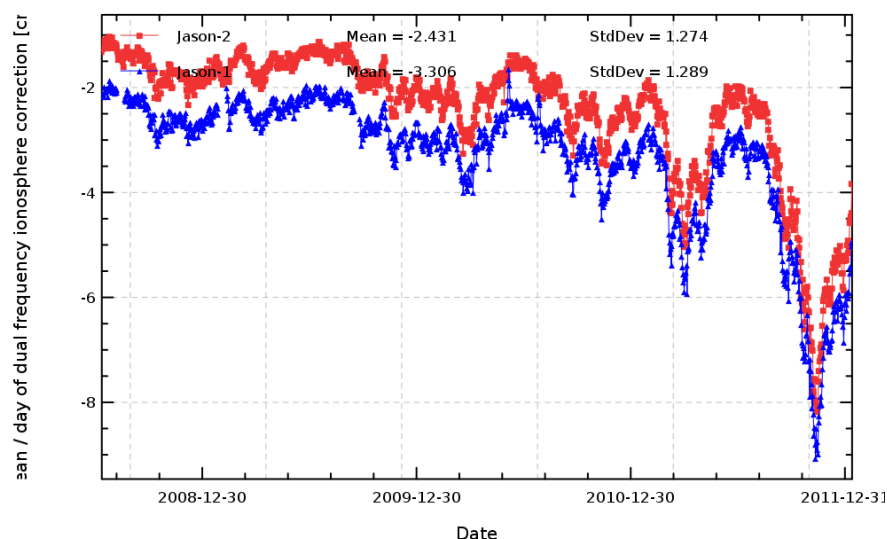
FIG. 9 – Daily monitoring of dual-frequency ionosphere correction for Jason-2 and Jason-1.
