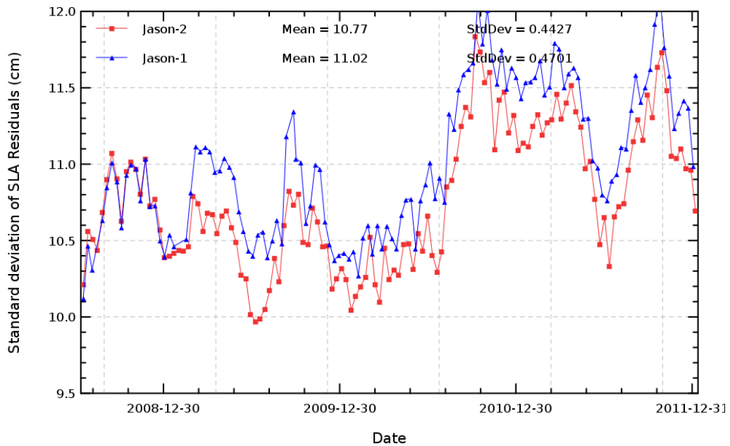
FIG. 22 – Cyclic monitoring standard deviation of along track SLA for Jason-1 and Jason-2.
