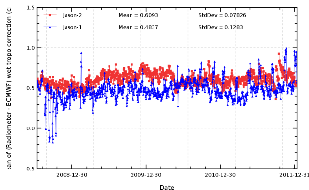
FIG. 13 – Daily monitoring of wet troposphere differences between radiometer and ECMWF model
