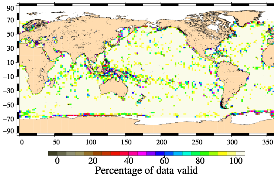
FIG. 3 – Percentage of valid measurements for cycle 129.
