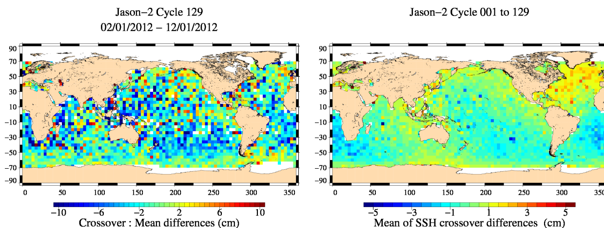
FIG. 14 – Mean SSH at crossovers for cycle 129 (left) and over the whole Jason-2 period (right).
