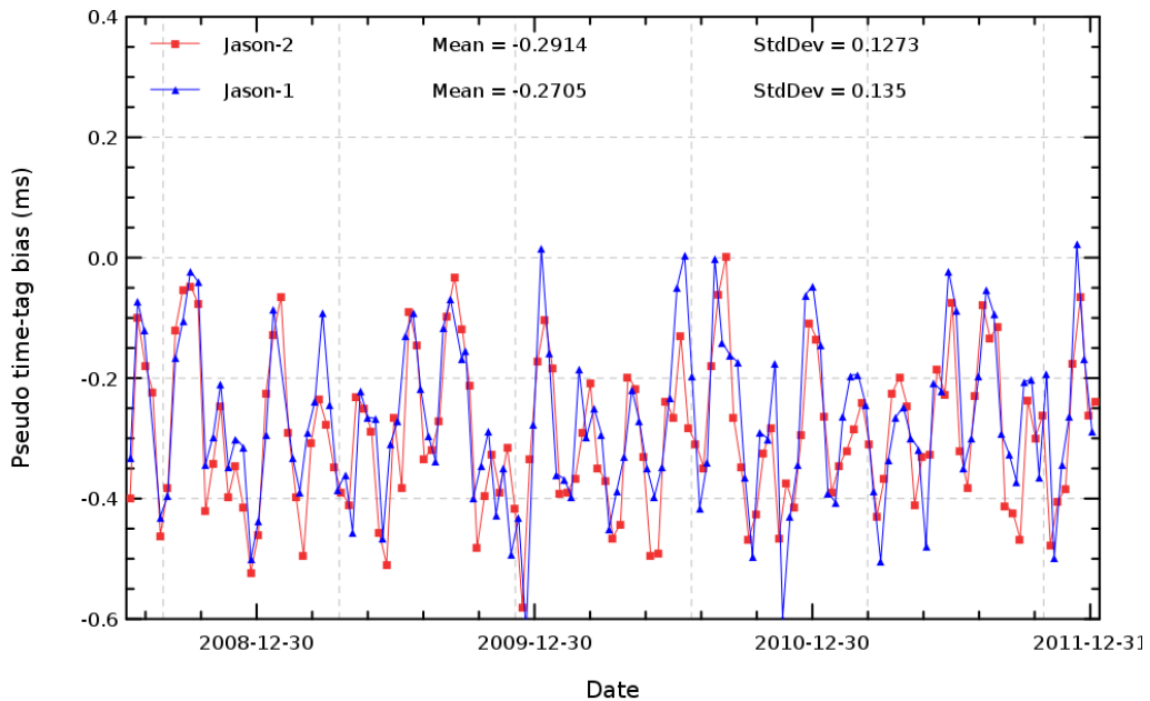
FIG. 17 – Cyclic monitoring of pseudo time tag bias for Jason-1 and Jason-2.
