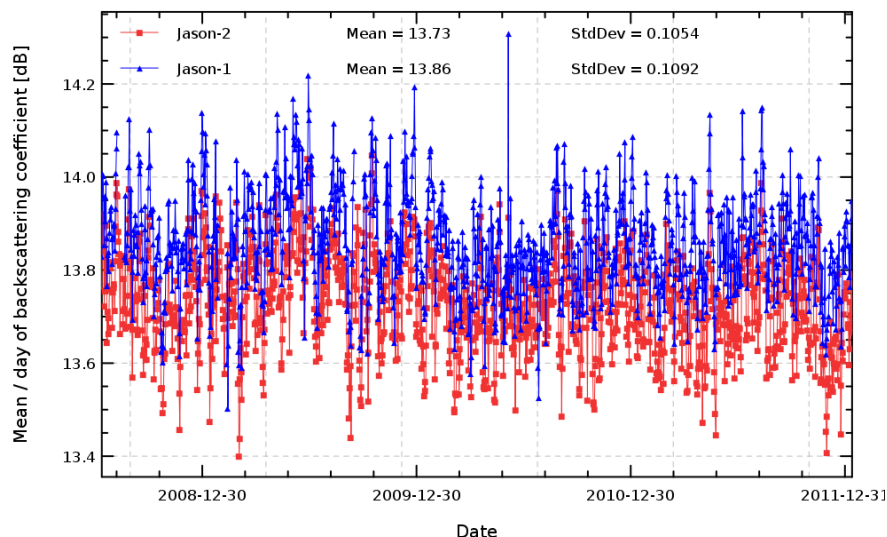
FIG. 8 – Daily monitoring of Ku-band backscattering coefficient for Jason-2 and Jason-1.
