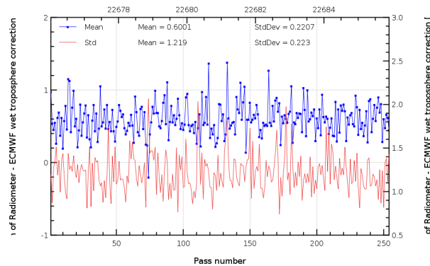
FIG. 11 – Pass monitoring of wet troposphere differences between radiometer and ECMWF model for Jason-2 cycle 132.
