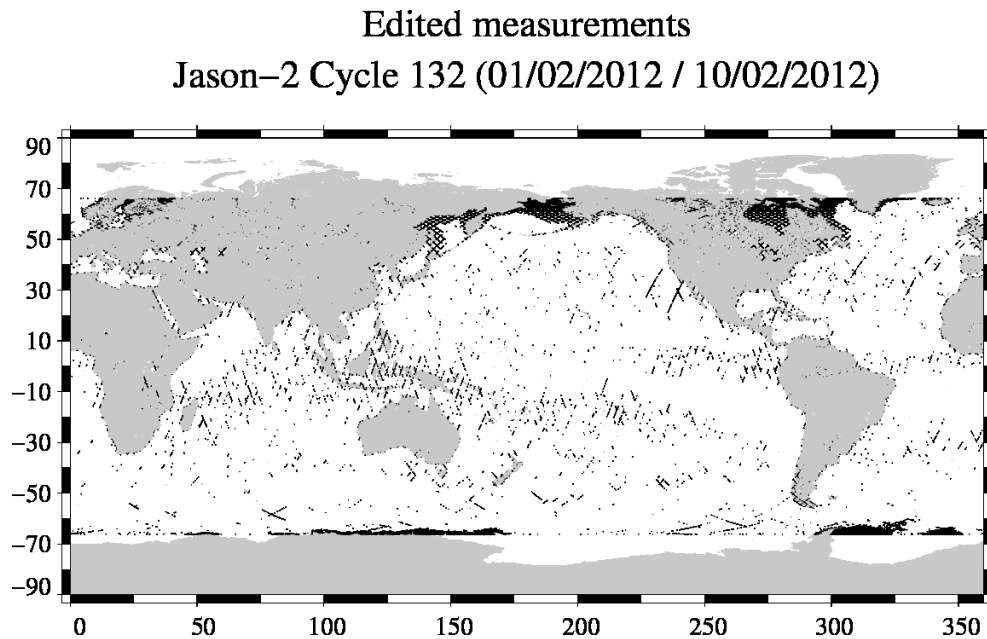
FIG. 2 – Edited measurements for cycle 132.
