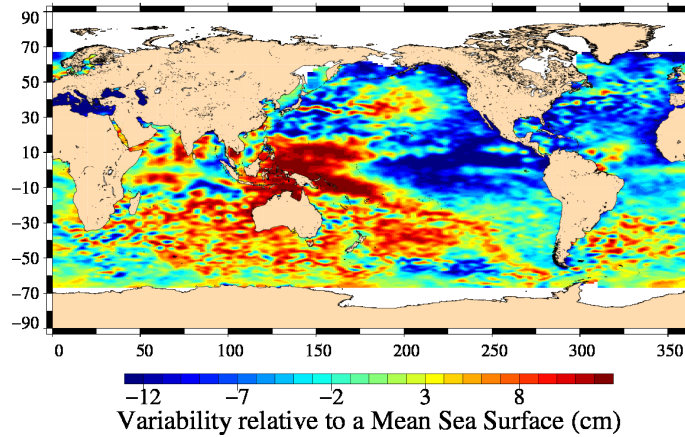
FIG. 19 – Sea level anomaly relative to MSS for cycle 134.
