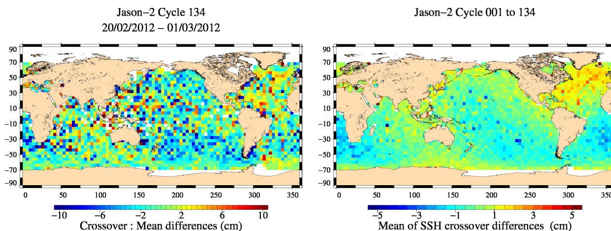
FIG. 14 – Mean SSH at crossovers for cycle 134 (left) and over the whole Jason-2 period (right).
