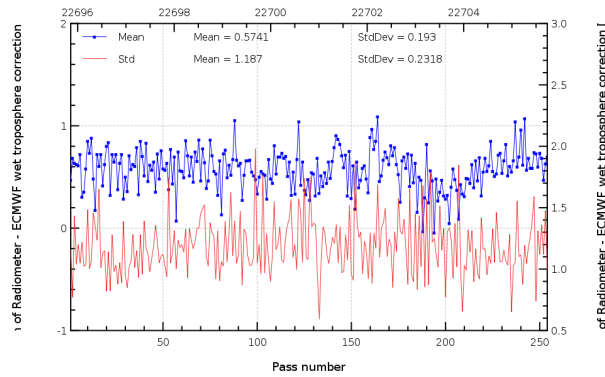
FIG. 11 – Pass monitoring of wet troposphere differences between radiometer and ECMWF model for Jason-2 cycle 134.
