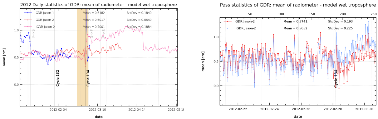
FIG. 12 – Left : Daily monitoring of wet troposphere differences between radiometer and ECMWF model for year 2012 - Right : Pass monitoring of wet troposphere differences between radiometer and ECMWF model for Jason-2 Gdrs and IGDRs during cycle 134.
