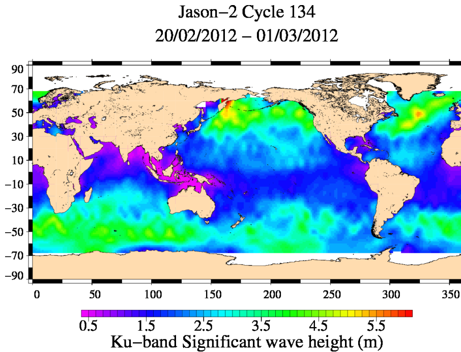
FIG. 5 – Significant wave height for cycle 134.
