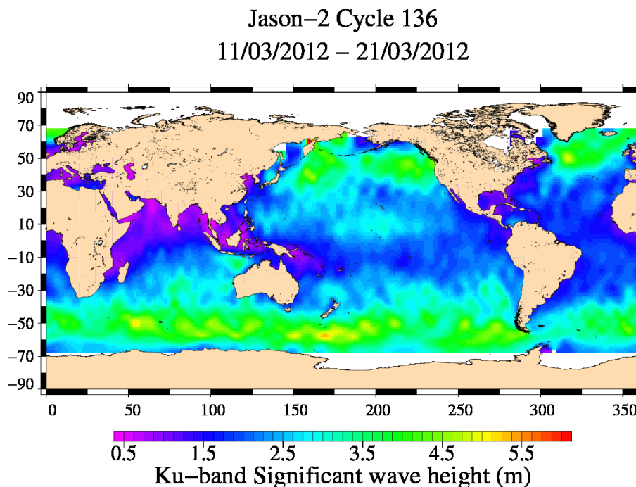
FIG. 5 – Significant wave height for cycle 136.
