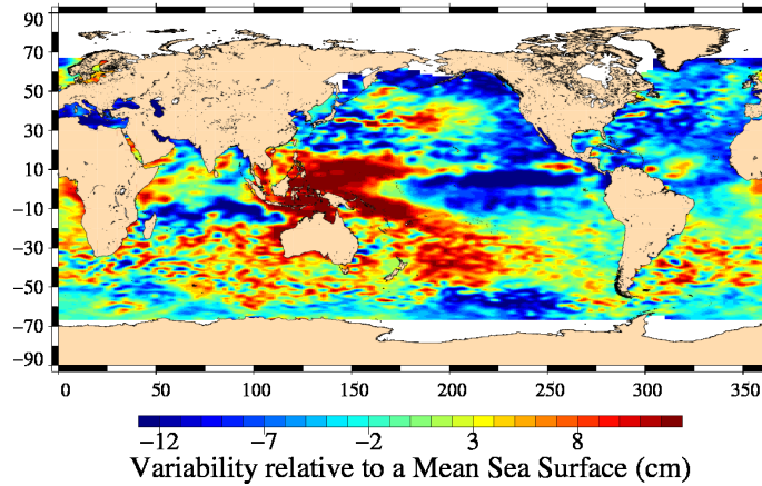
FIG. 18 – Sea level anomaly relative to MSS for cycle 136.
