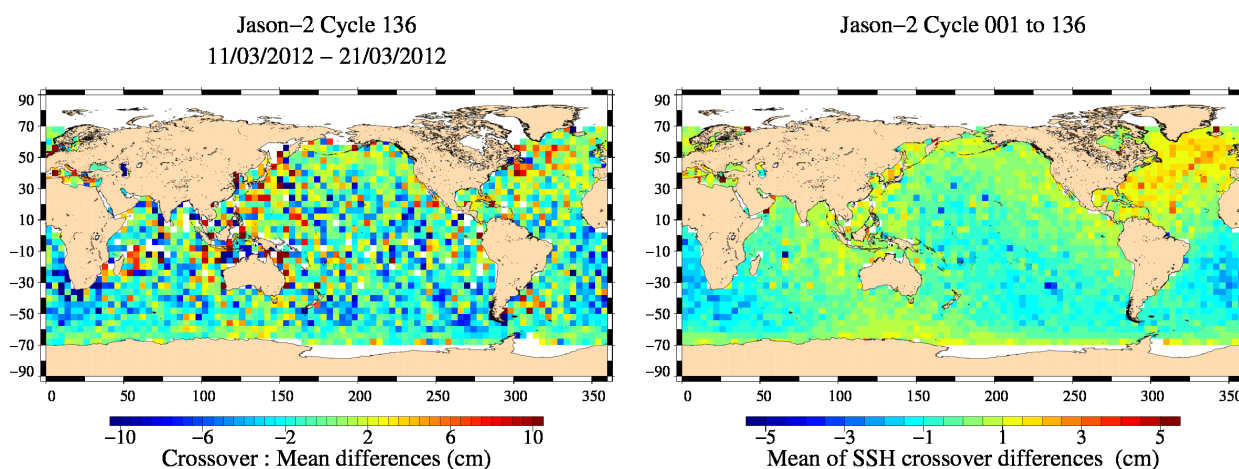
FIG. 13 – Mean SSH at crossovers for cycle 136 (left) and over the whole Jason-2 period (right).
