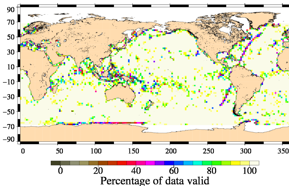
FIG. 3 – Percentage of valid measurements for cycle 136.
