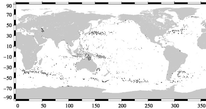
FIG. 19 – Differences higher than a 30 cm threshold for cycle 136.
