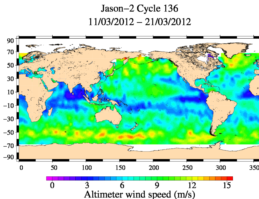
FIG. 9 – Altimeter wind speed for cycle 136.
