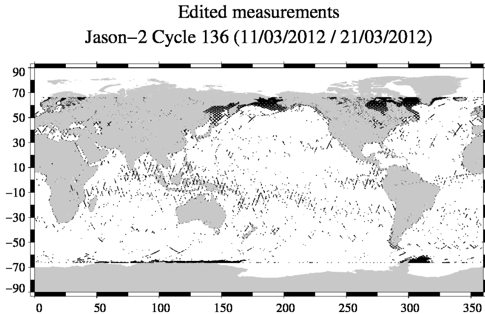
FIG. 2 – Edited measurements for cycle 136.
