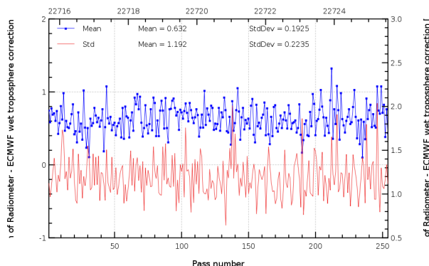
FIG. 11 – Pass monitoring of wet troposphere differences between radiometer and ECMWF model for Jason-2 cycle 136.
