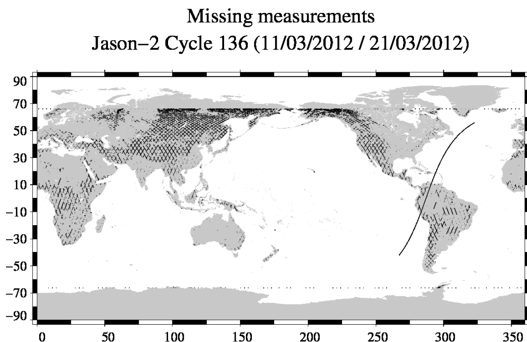
FIG. 1 – Missing measurements for cycle 136.
