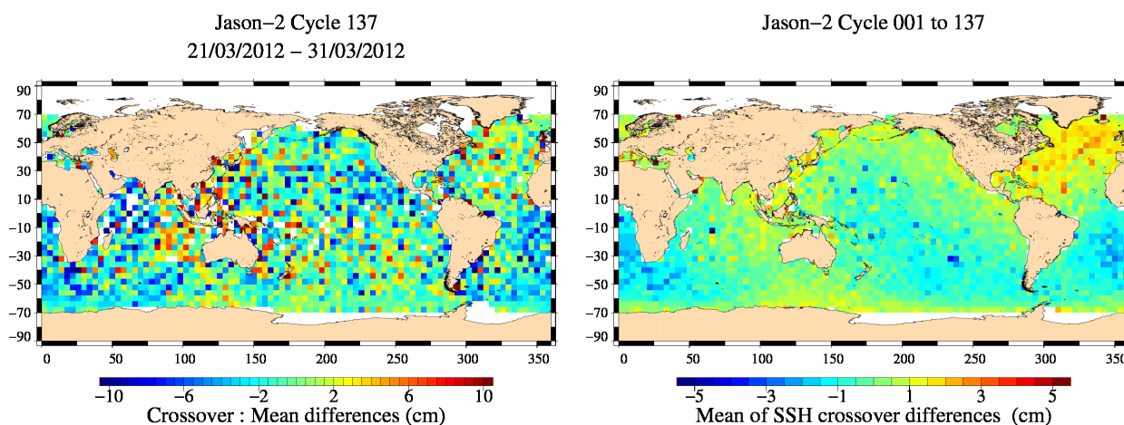
FIG. 13 – Mean SSH at crossovers for cycle 137 (left) and over the whole Jason-2 period (right).
