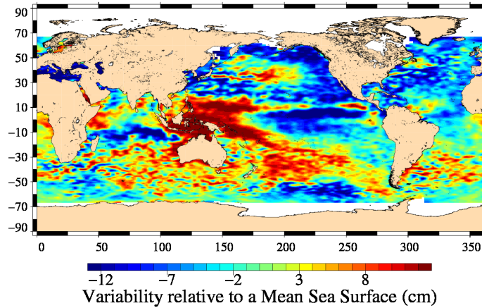
FIG. 18 – Sea level anomaly relative to MSS for cycle 137.
