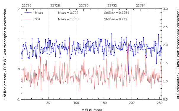
FIG. 11 – Pass monitoring of wet troposphere differences between radiometer and ECMWF model for Jason-2 cycle 137.
