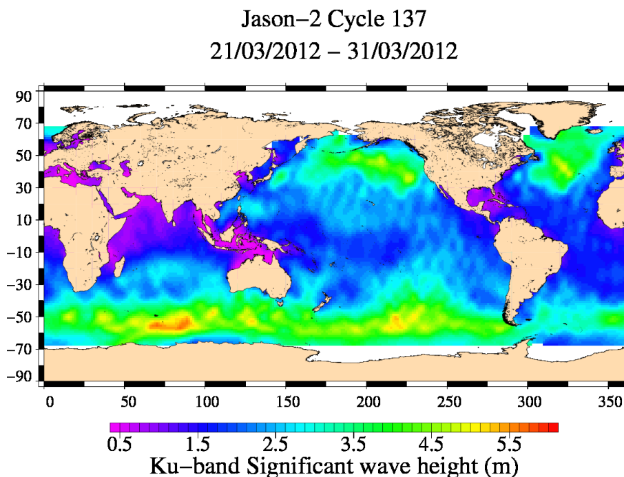
FIG. 5 – Significant wave height for cycle 137.
