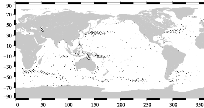
FIG. 19 – Differences higher than a 30 cm threshold for cycle 137.
