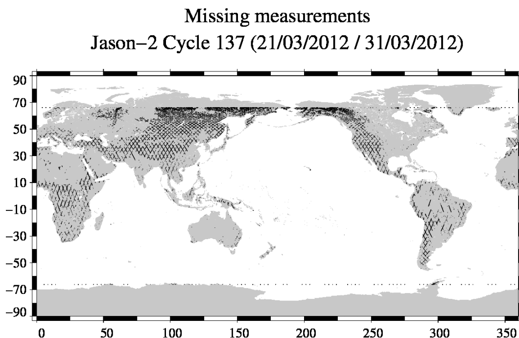
FIG. 1 – Missing measurements for cycle 137.
