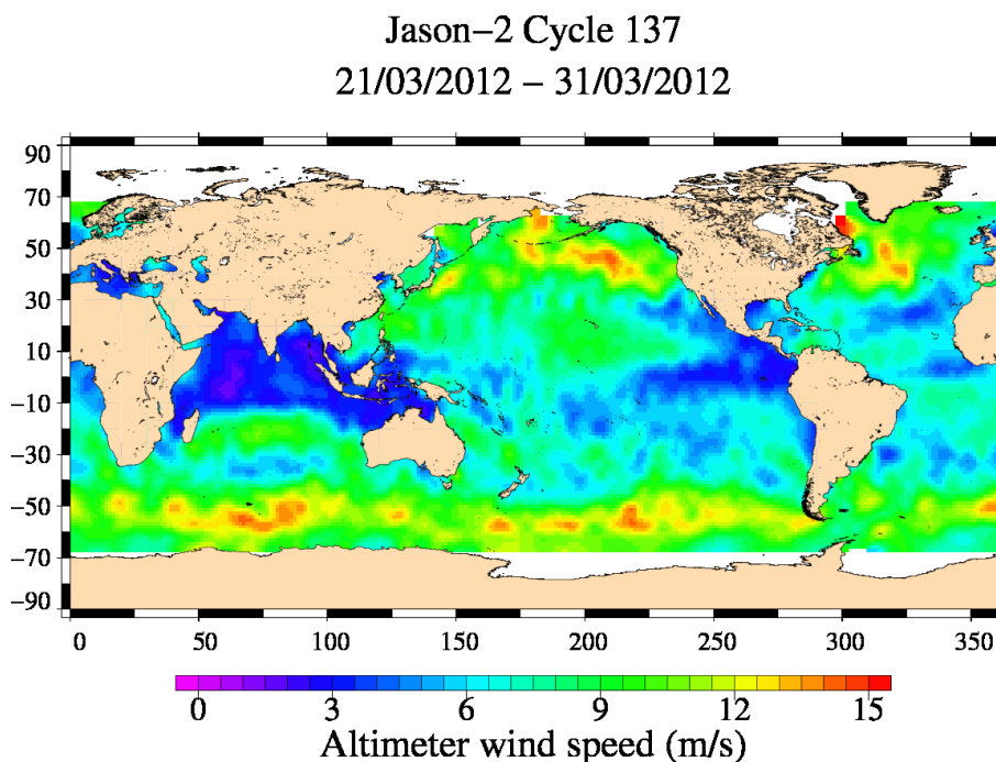
FIG. 9 – Altimeter wind speed for cycle 137.
