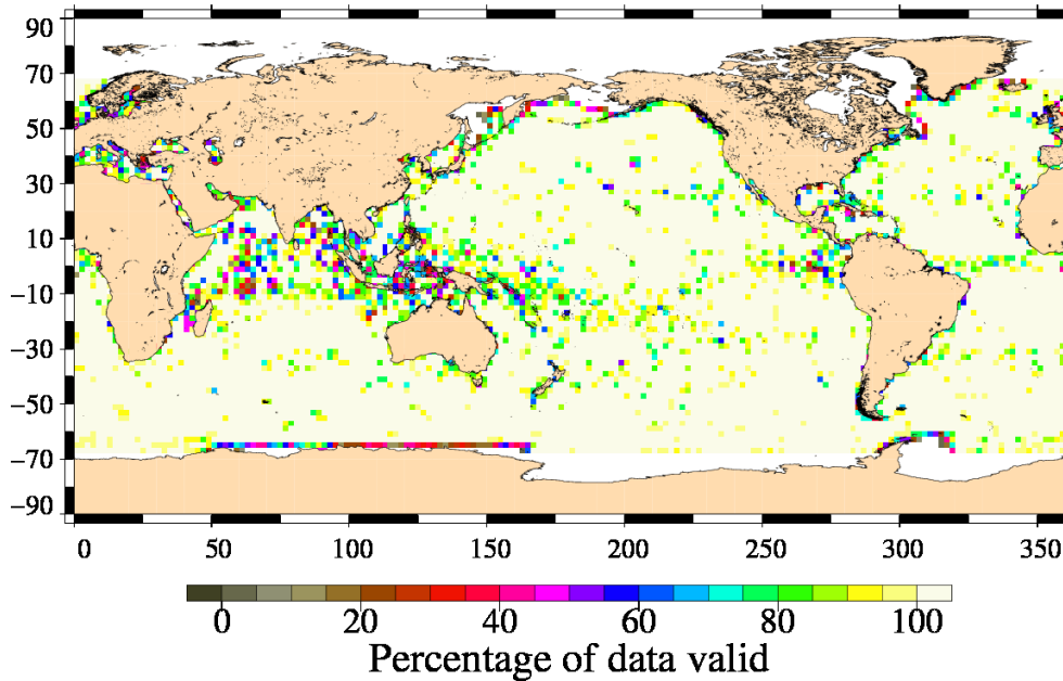
FIG. 3 – Percentage of valid measurements for cycle 137.
