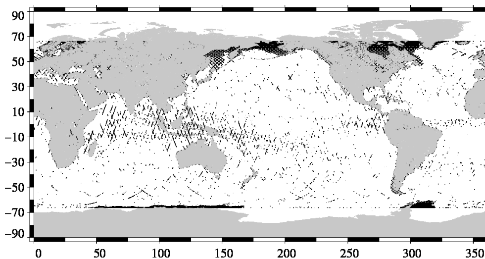
FIG. 2 – Edited measurements for cycle 137.
