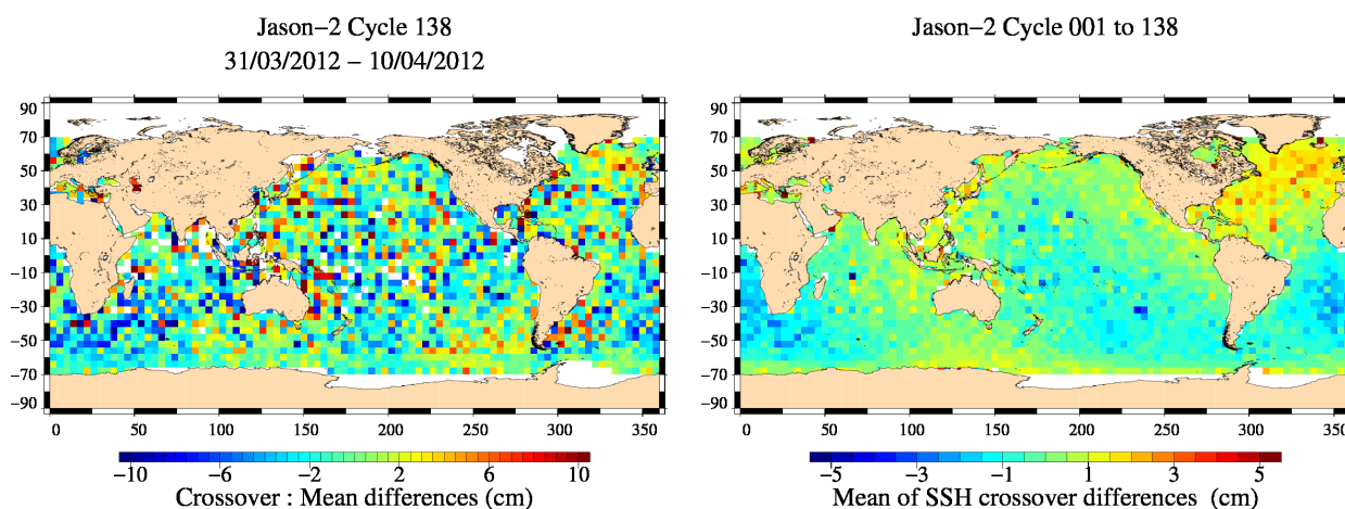
FIG. 13 – Mean SSH at crossovers for cycle 138 (left) and over the whole Jason-2 period (right).
