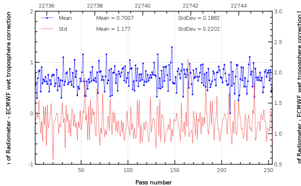
FIG. 11 – Pass monitoring of wet troposphere differences between radiometer and ECMWF model for Jason-2 cycle 138.
