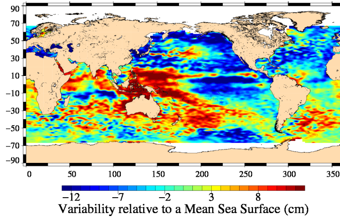
FIG. 18 – Sea level anomaly relative to MSS for cycle 138.
