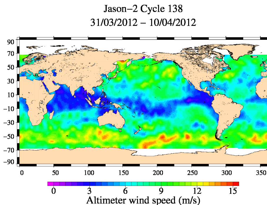
FIG. 9 – Altimeter wind speed for cycle 138.
