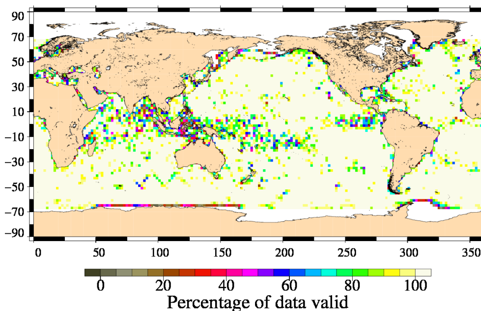
FIG. 3 – Percentage of valid measurements for cycle 138.
