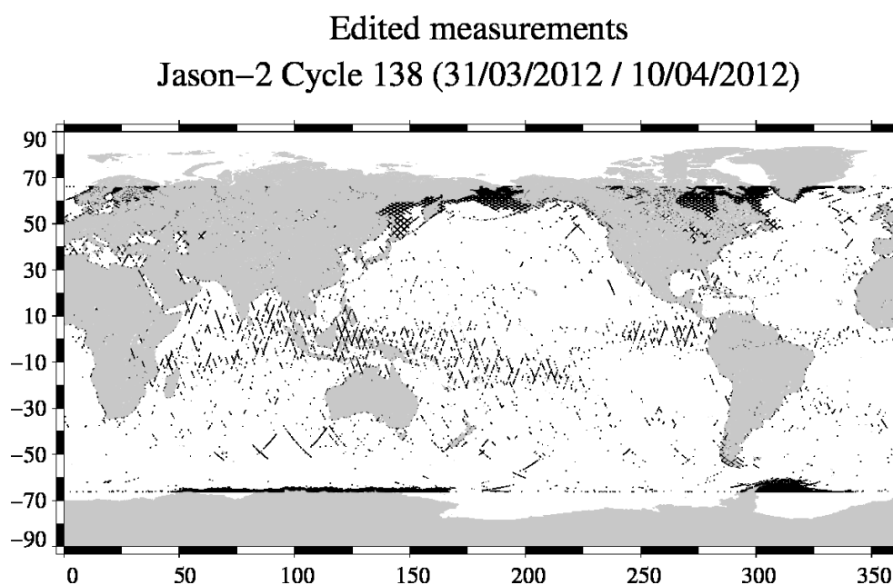
FIG. 2 – Edited measurements for cycle 138.
