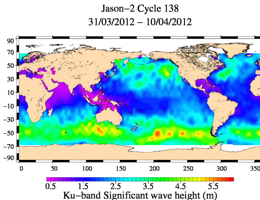
FIG. 5 – Significant wave height for cycle 138.
