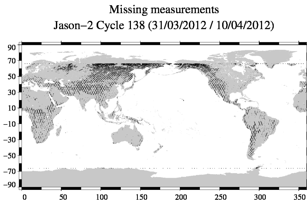
FIG. 1 – Missing measurements for cycle 138.
