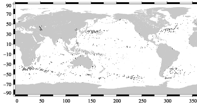
FIG. 19 – Differences higher than a 30 cm threshold for cycle 138.
