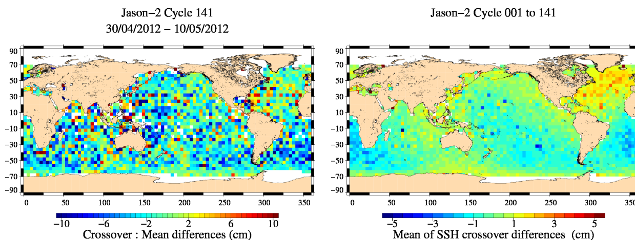
FIG. 13 – Mean SSH at crossovers for cycle 141 (left) and over the whole Jason-2 period (right).
