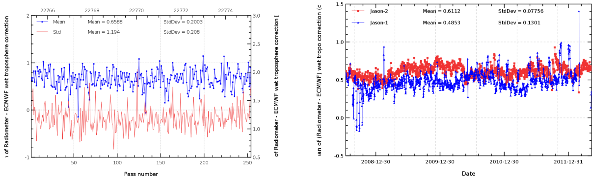
FIG. 12 – Pass monitoring of wet troposphere differences between radiometer and ECMWF model for Jason-2 cycle 141. (left) and Daily monitoring of wet troposphere differences between radiometer and ECMWF model (right).
