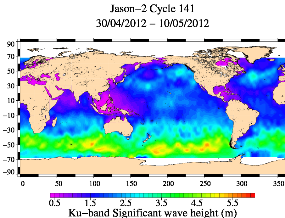
FIG. 6 – Significant wave height for cycle 141.
