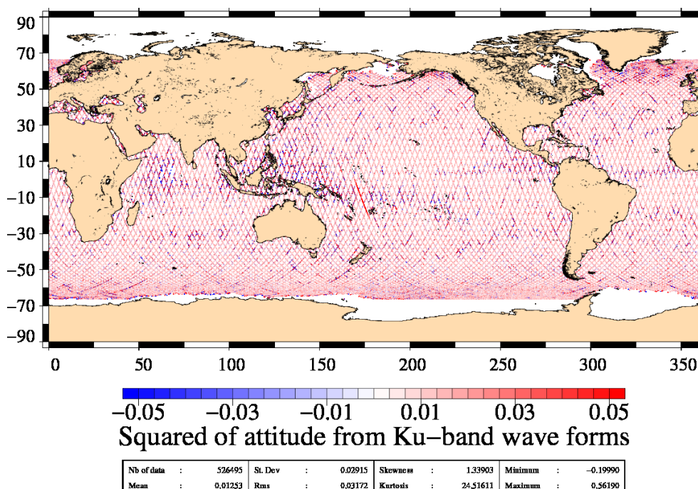
FIG. 4 – Apparent squared mispointing from waveforms for cycle 141.
