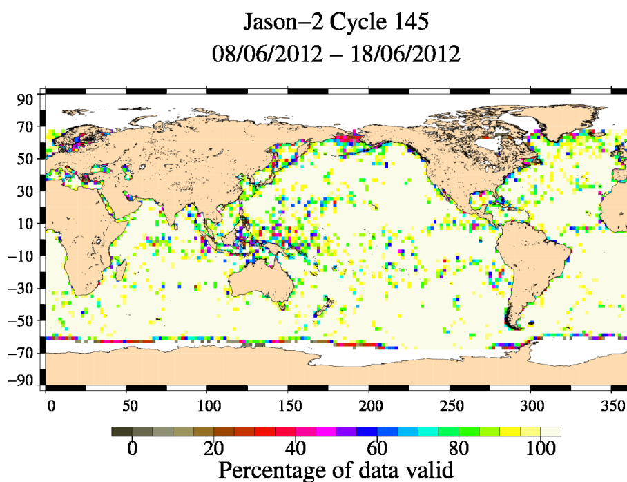
FIG. 3 – Percentage of valid measurements for cycle 145.
