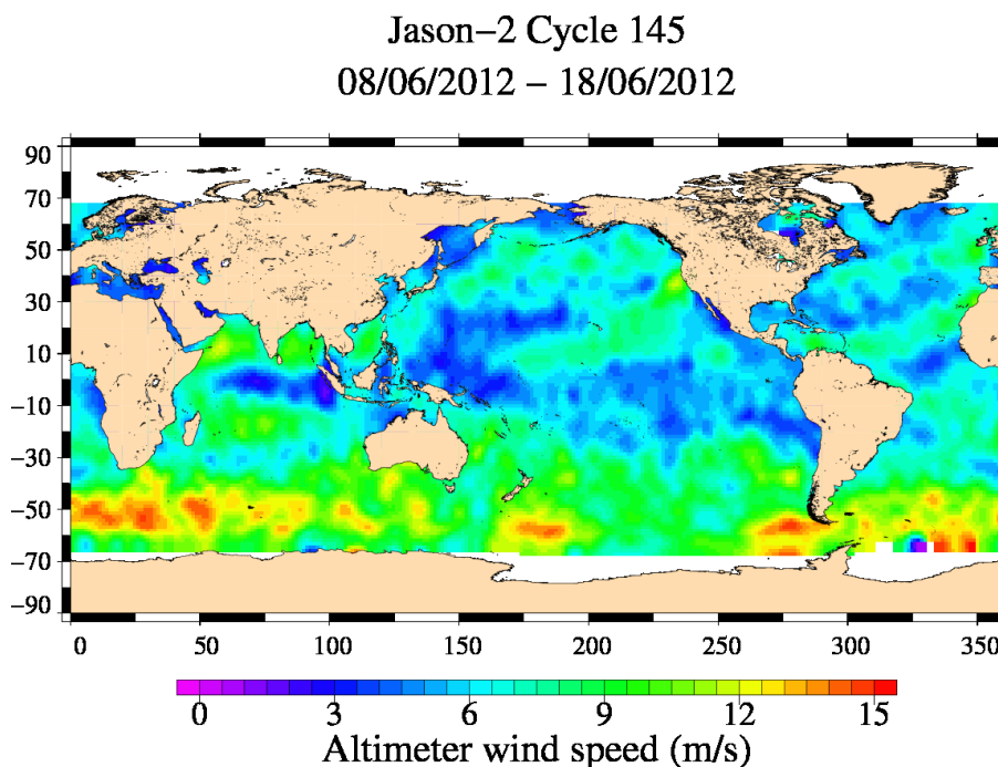
FIG. 9 – Altimeter wind speed for cycle 145.
