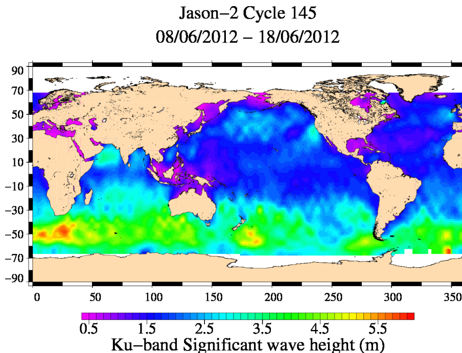
FIG. 5 – Significant wave height for cycle 145.
