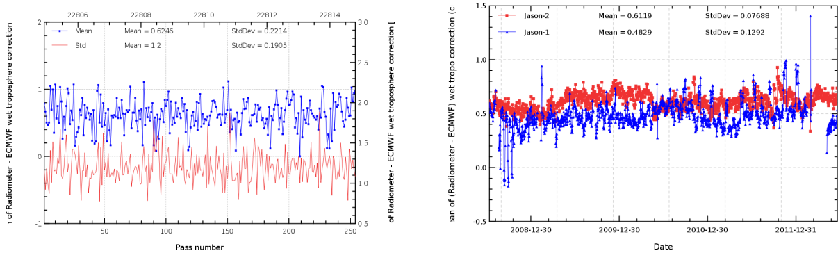
FIG. 11 – Pass monitoring of wet troposphere differences between radiometer and ECMWF model for Jason-2 cycle 145. (left) and Daily monitoring of wet troposphere differences between radiometer and ECMWF model (right).
