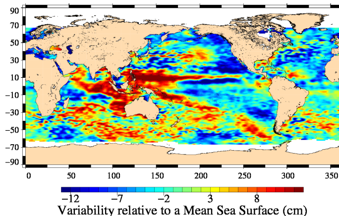
FIG. 17 – Sea level anomaly relative to MSS for cycle 145.
