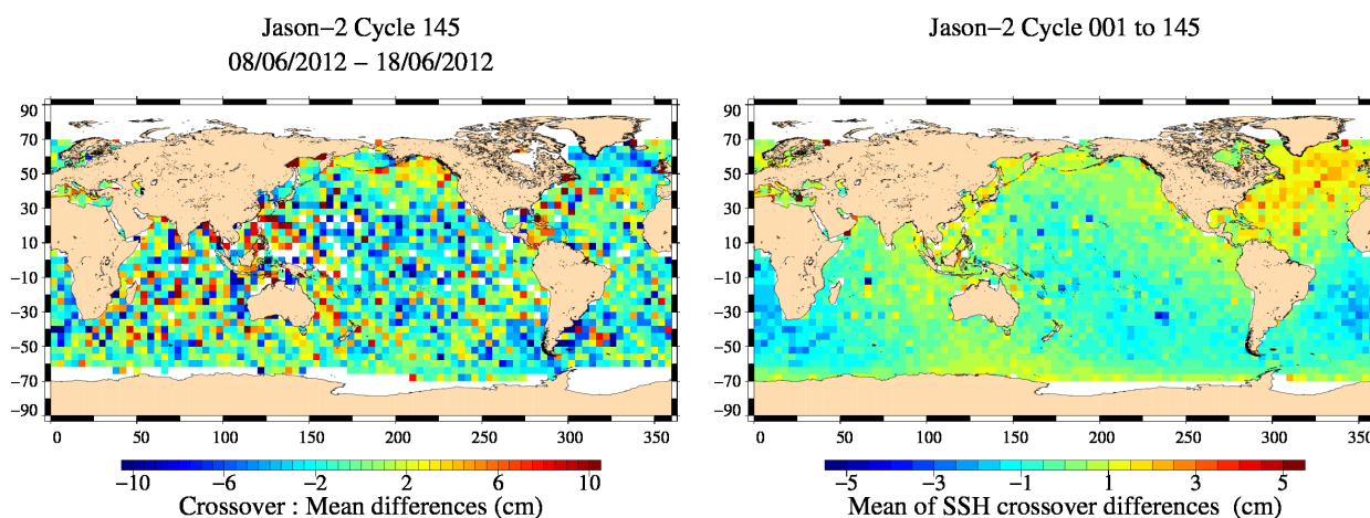
FIG. 12 – Mean SSH at crossovers for cycle 145 (left) and over the whole Jason-2 period (right).
