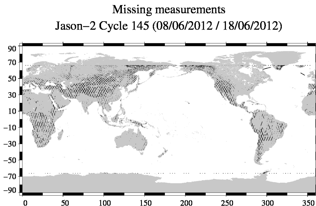
FIG. 1 – Missing measurements for cycle 145.
