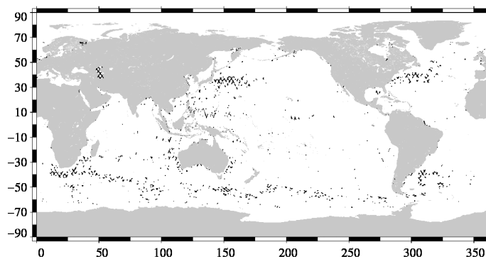
FIG. 18 – Differences higher than a 30 cm threshold for cycle 145.
