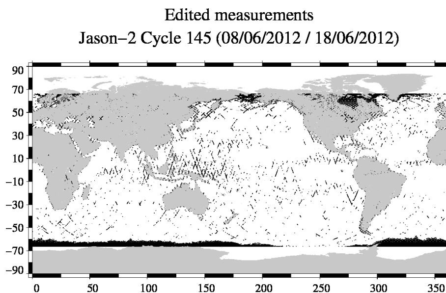
FIG. 2 – Edited measurements for cycle 145.
