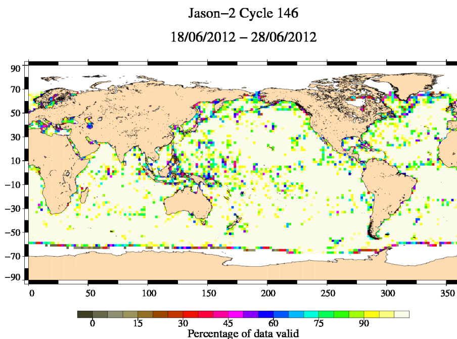
FIG. 3 – Percentage of valid measurements for cycle 146.
