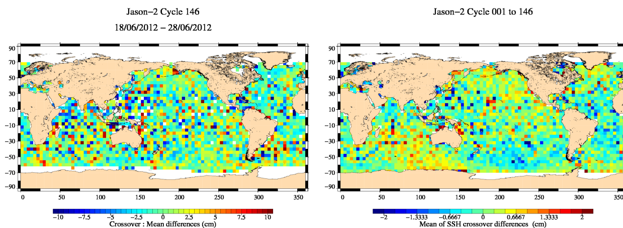
FIG. 12 – Mean SSH at crossovers for cycle 146 (left) and over the whole Jason-2 period (right).
