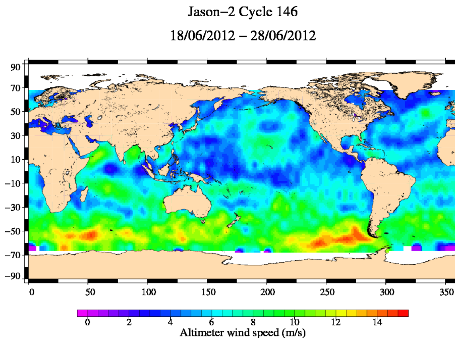
FIG. 9 – Altimeter wind speed for cycle 146.
