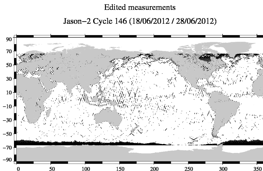
FIG. 2 – Edited measurements for cycle 146.
