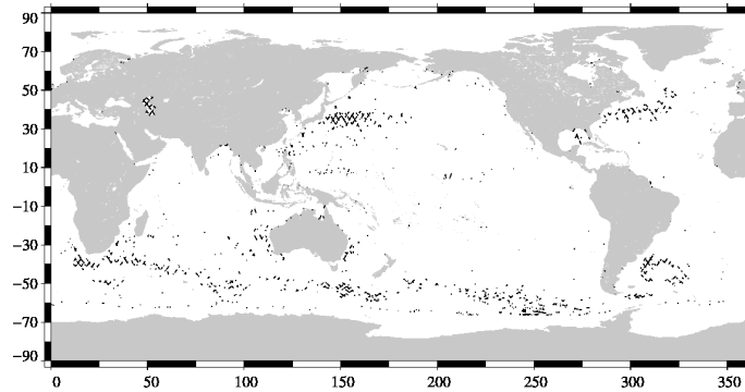
FIG. 18 – Differences higher than a 30 cm threshold for cycle 146.
