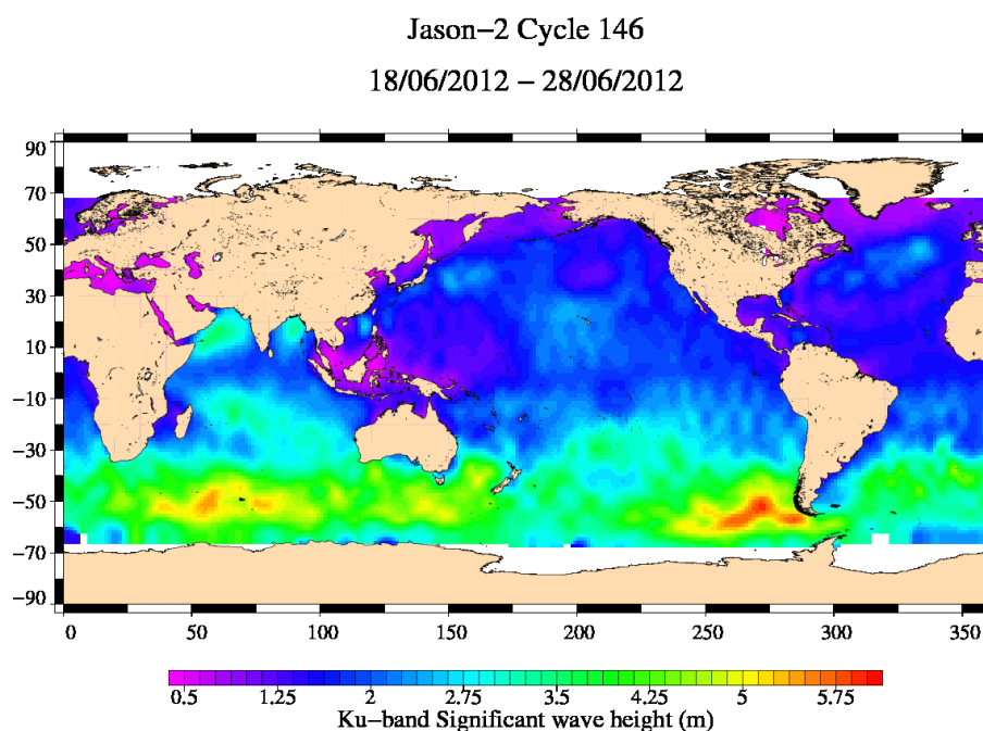
FIG. 5 – Significant wave height for cycle 146.
