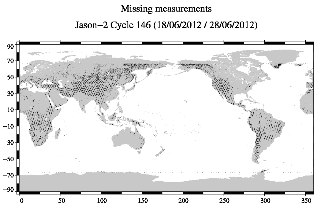
FIG. 1 – Missing measurements for cycle 146.
