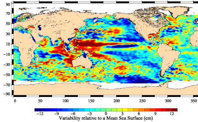
FIG. 17 – Sea level anomaly relative to MSS for cycle 146.
