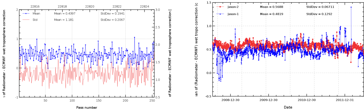
FIG. 11 – Pass monitoring of wet troposphere differences between radiometer and ECMWF model for Jason-2 cycle 146 (left) and daily monitoring of wet troposphere differences between radiometer and ECMWF model (right).
