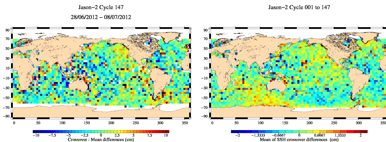
FIG. 13 – Mean SSH at crossovers for cycle 147 (left) and over the whole Jason-2 period (right).
