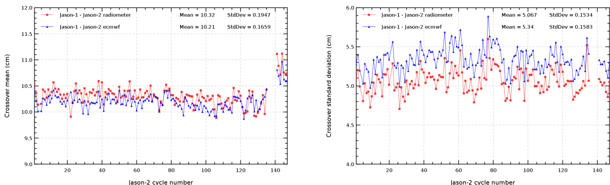
FIG. 15 – Cyclic monitoring of mean (left) and standard deviation (right) of (Jason-1 – Jason-2) SSH differences at crossovers.
