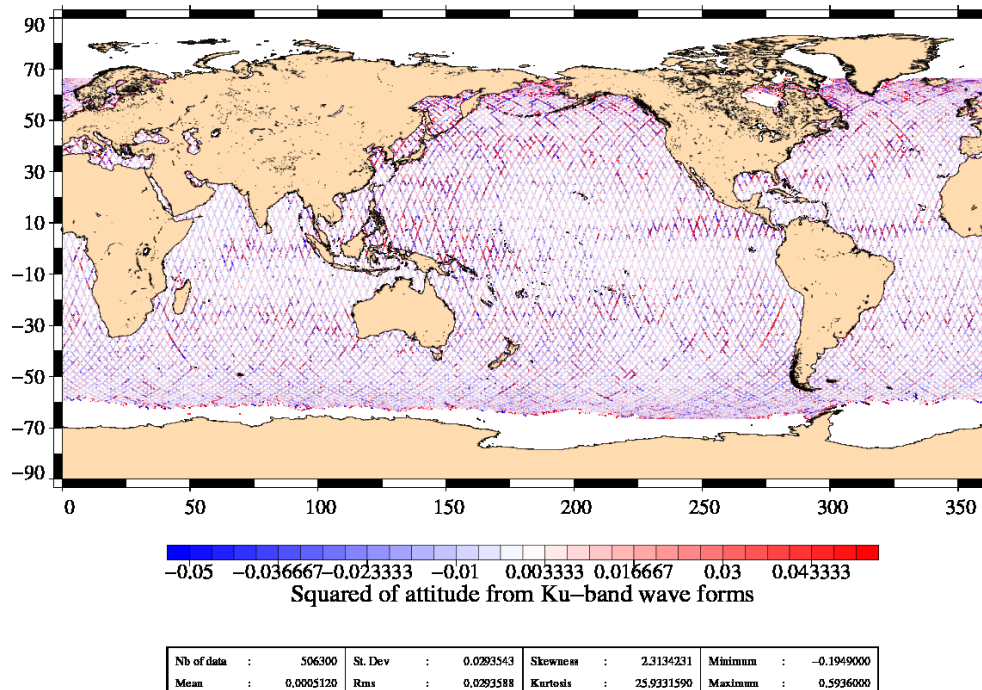
FIG. 4 – Apparent squared mispointing from waveforms for cycle 147.
