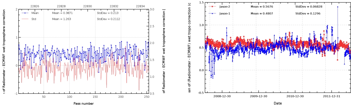
FIG. 12 – Pass monitoring of wet troposphere differences between radiometer and ECMWF model for Jason-2 cycle 147 (left) and daily monitoring of wet troposphere differences between radiometer and ECMWF model (right).
