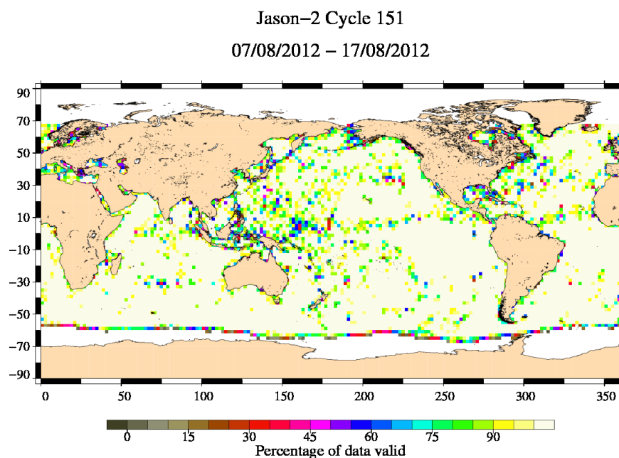
FIG. 3 – Percentage of valid measurements for cycle 151.
