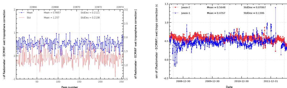
FIG. 11 – Pass monitoring of wet troposphere differences between radiometer and ECMWF model for Jason-2 cycle 151 (left) and daily monitoring of wet troposphere differences between radiometer and ECMWF model (right).
