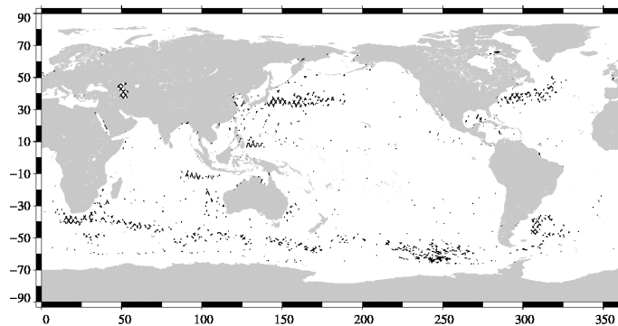
FIG. 18 – Differences higher than a 30 cm threshold for cycle 151.
