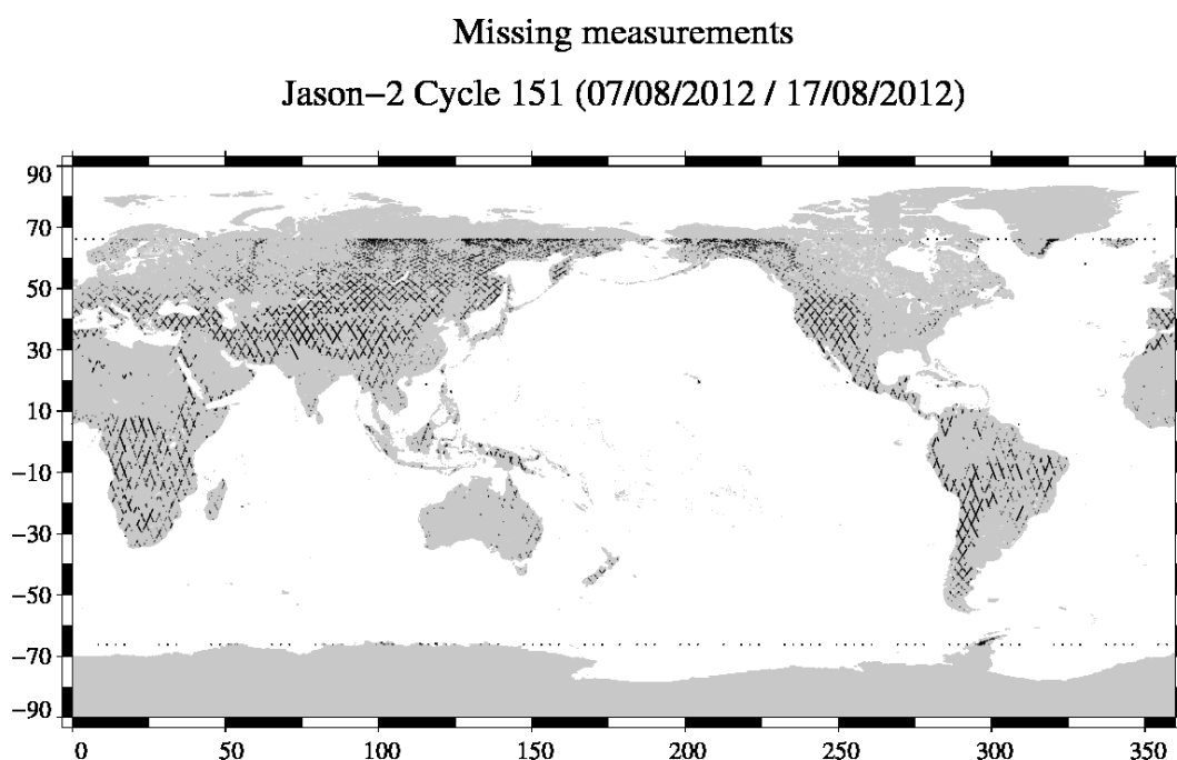
FIG. 1 – Missing measurements for cycle 151.
