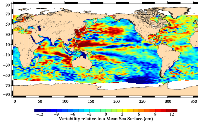
FIG. 17 – Sea level anomaly relative to MSS for cycle 151.
