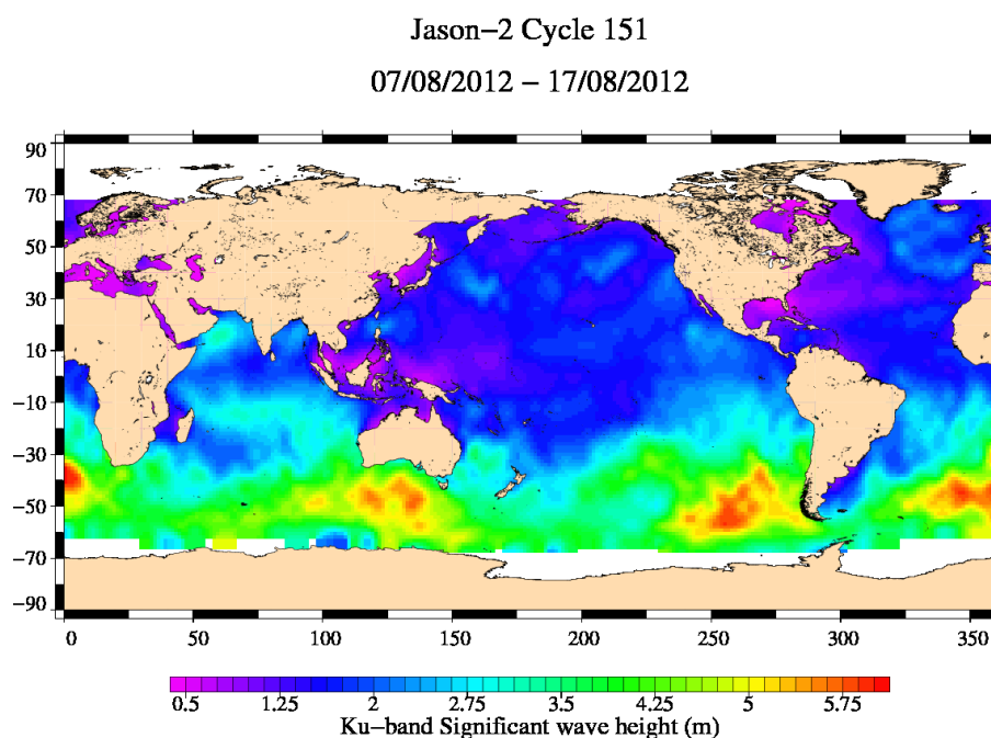
FIG. 5 – Significant wave height for cycle 151.
