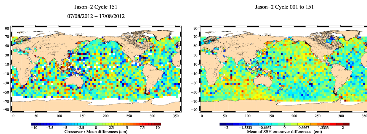
FIG. 12 – Mean SSH at crossovers for cycle 151 (left) and over the whole Jason-2 period (right).
