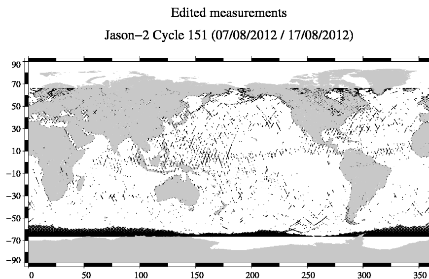
FIG. 2 – Edited measurements for cycle 151.
