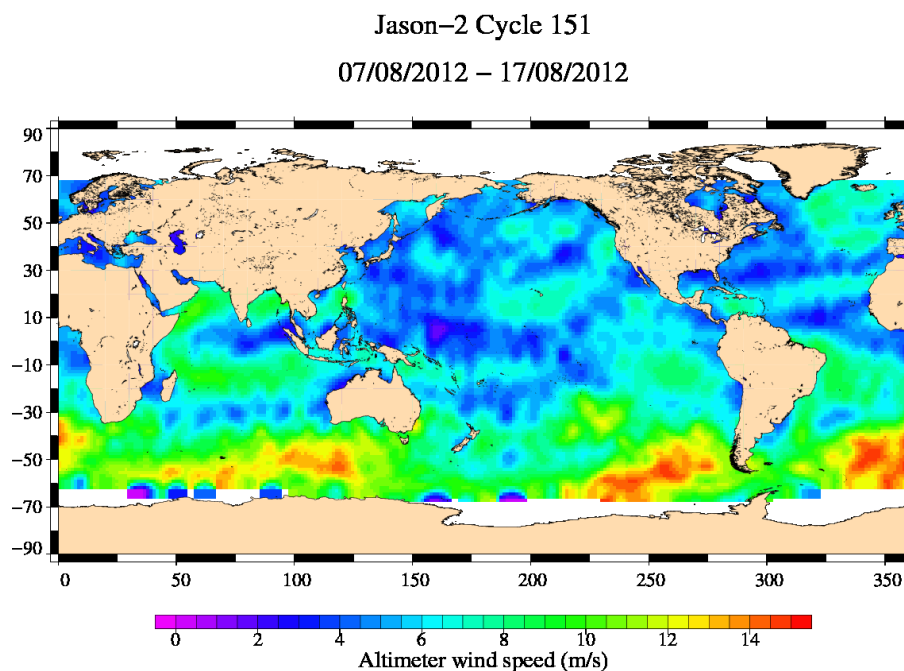
FIG. 9 – Altimeter wind speed for cycle 151.
