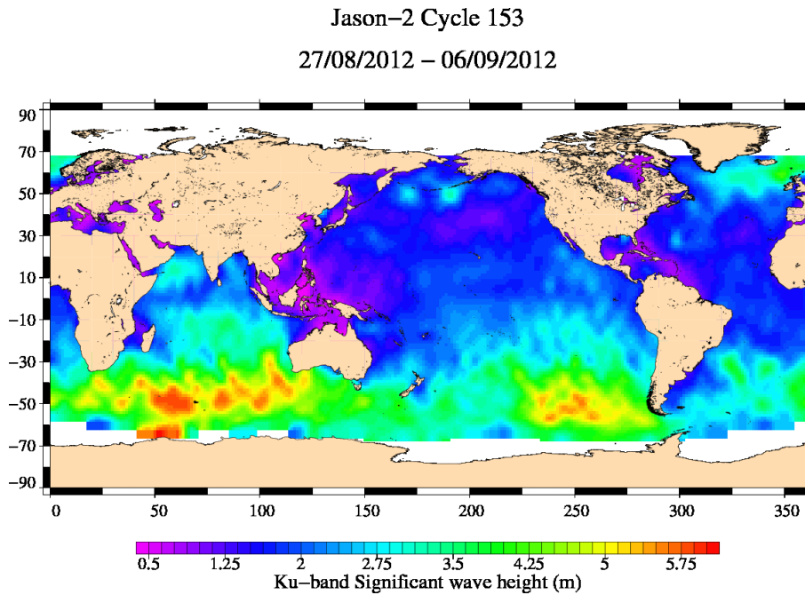
FIG. 6 – Significant wave height for cycle 153.
