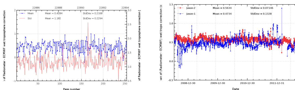
FIG. 12 – Pass monitoring of wet troposphere differences between radiometer and ECMWF model for Jason-2 cycle 153 (left) and daily monitoring of wet troposphere differences between radiometer and ECMWF model (right).
