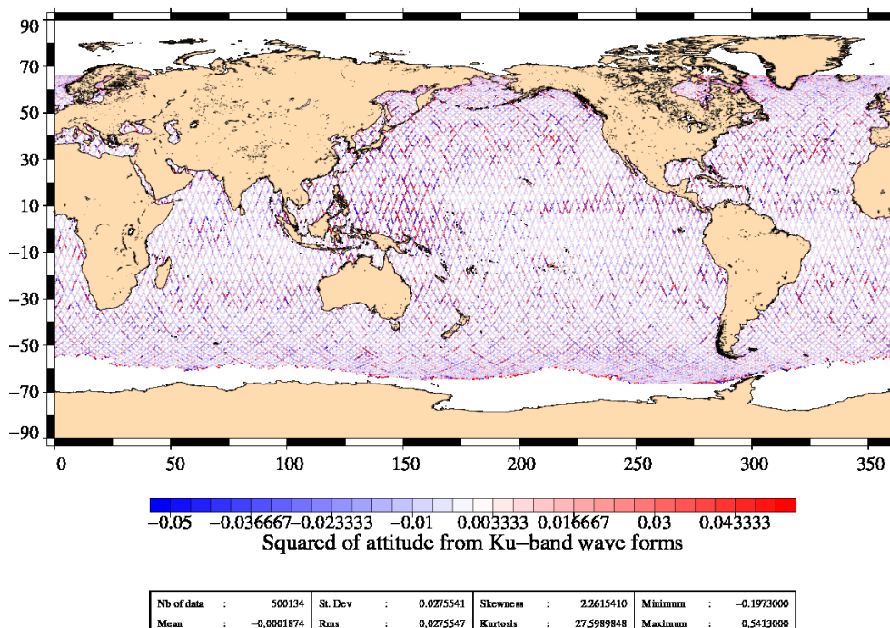
FIG. 4 – Apparent squared mispointing from waveforms for cycle 153.
