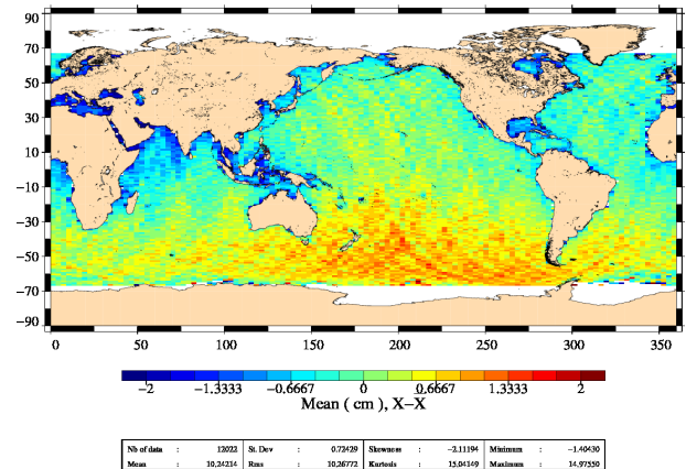
Differences of SLA before orbit error correction Jason-1 – Jason-2 (Cycle 1 – 020)
