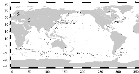
Valid data: (SSH – MSS) differences greater than 30 cm Jason-2 Cycle 157 (05/10/2012 / 15/10/2012)
