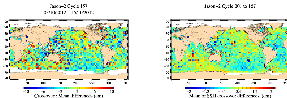
FIG. 12 – Mean SSH at crossovers for cycle 157 (left) and over the whole Jason-2 period (right).
