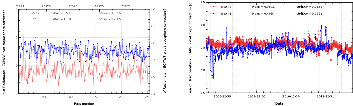
FIG. 11 – Pass monitoring of wet troposphere differences between radiometer and ECMWF model for Jason-2 cycle 157 (left) and daily monitoring of wet troposphere differences between radiometer and ECMWF model (right).
