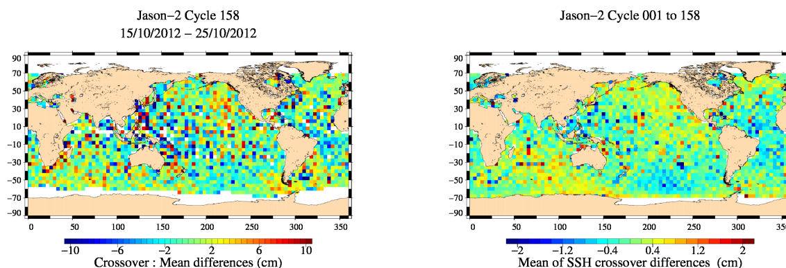
FIG. 12 – Mean SSH at crossovers for cycle 158 (left) and over the whole Jason-2 period (right).
