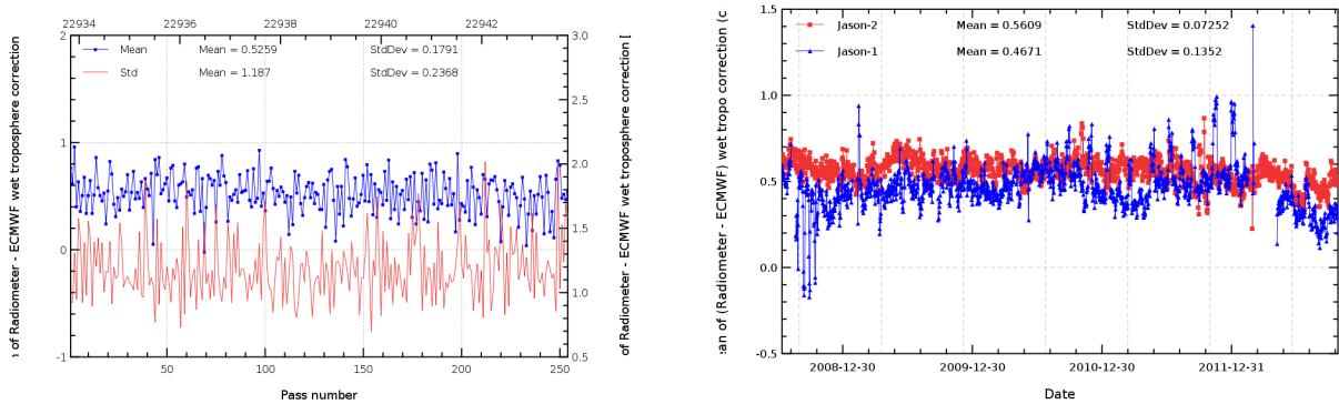
FIG. 11 – Pass monitoring of wet troposphere differences between radiometer and ECMWF model for Jason-2 cycle 158 (left) and daily monitoring of wet troposphere differences between radiometer and ECMWF model (right).
