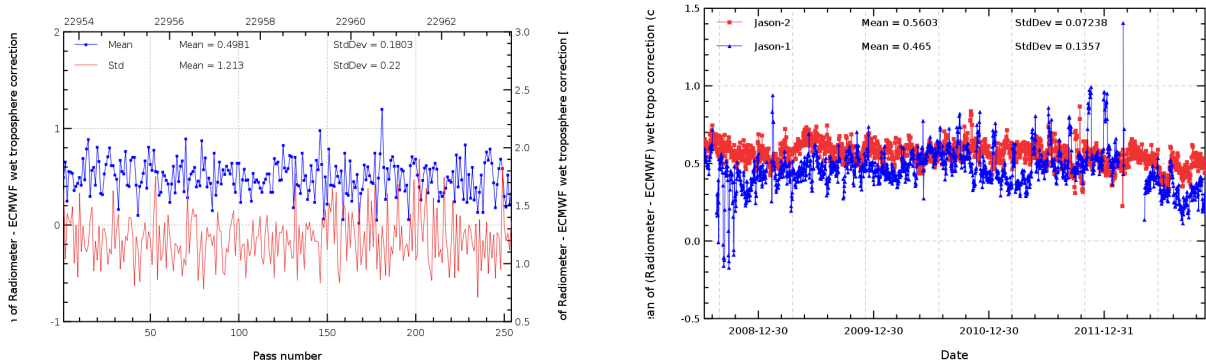
FIG. 11 – Pass monitoring of wet troposphere differences between radiometer and ECMWF model for Jason-2 cycle 160 (left) and daily monitoring of wet troposphere differences between radiometer and ECMWF model (right).
