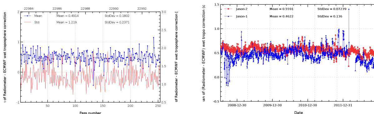
FIGURE 11 – Pass monitoring of wet troposphere differences between radiometer and ECMWF model for Jason-2 cycle 163 (left) and daily monitoring of wet troposphere differences between radiometer and ECMWF model (right).
