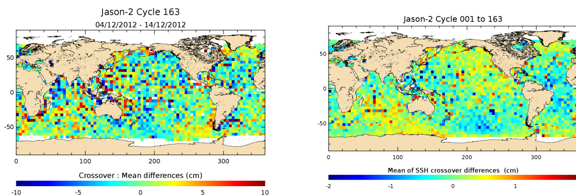
FIGURE 12 – Mean SSH at crossovers for cycle 163 (left) and over the whole Jason-2 period (right).
