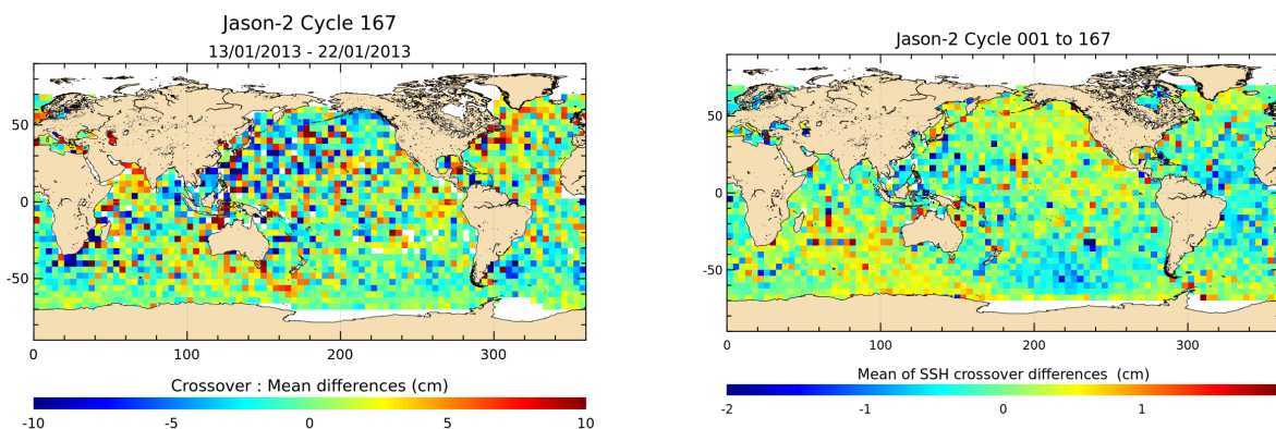
FIGURE 12 – Mean SSH at crossovers for cycle 167 (left) and over the whole Jason-2 period (right).
