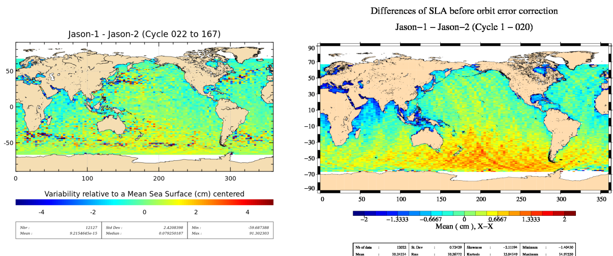
FIGURE 19 – Jason-1 – Jason-2 SLA differences averaged over whole Jason-2 period since cycle 022 (left), and for flight formation phase (cycle 001 to 020) (right).
