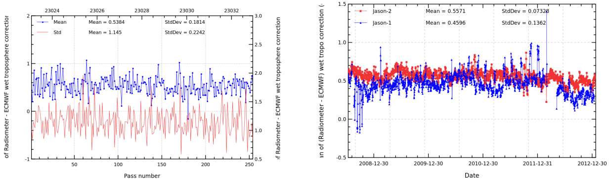
FIGURE 11 – Pass monitoring of wet troposphere differences between radiometer and ECMWF model for Jason-2 cycle 167 (left) and daily monitoring of wet troposphere differences between radiometer and ECMWF model (right).
