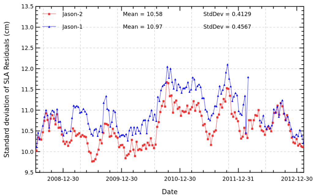
FIG. 20 – Cyclic monitoring standard deviation of along track SLA for Jason-1 and Jason-2.
