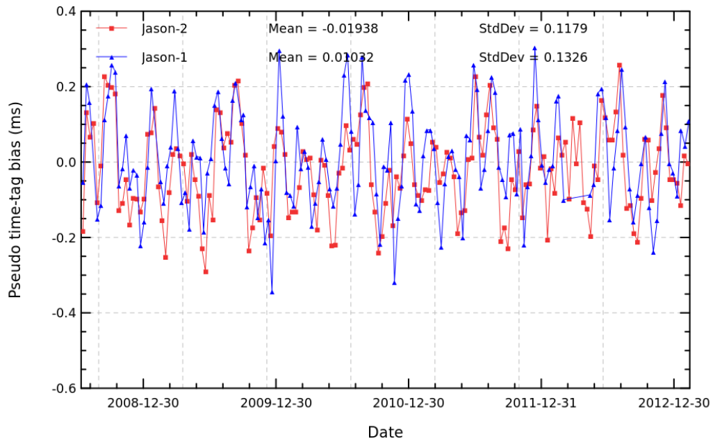
FIG. 15 – Cyclic monitoring of pseudo time tag bias for Jason-1 and Jason-2.
