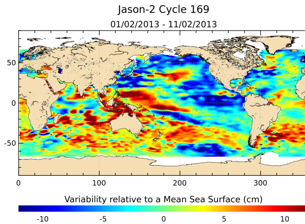
FIG. 17 – Sea level anomaly relative to MSS for cycle 169.
