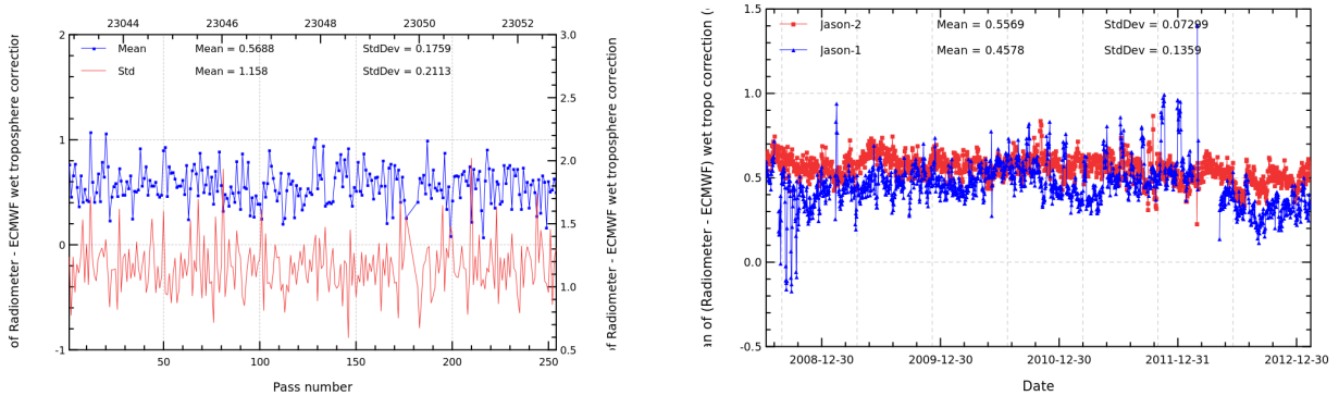
FIG. 11 – Pass monitoring of wet troposphere differences between radiometer and ECMWF model for Jason-2 cycle 169 (left) and daily monitoring of wet troposphere differences between radiometer and ECMWF model (right).
