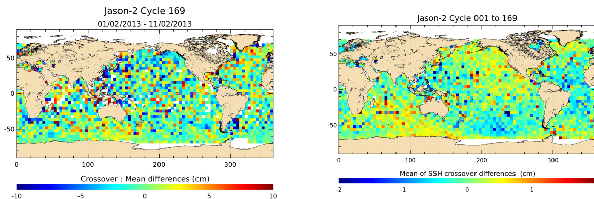
FIG. 12 – Mean SSH at crossovers for cycle 169 (left) and over the whole Jason-2 period (right).
