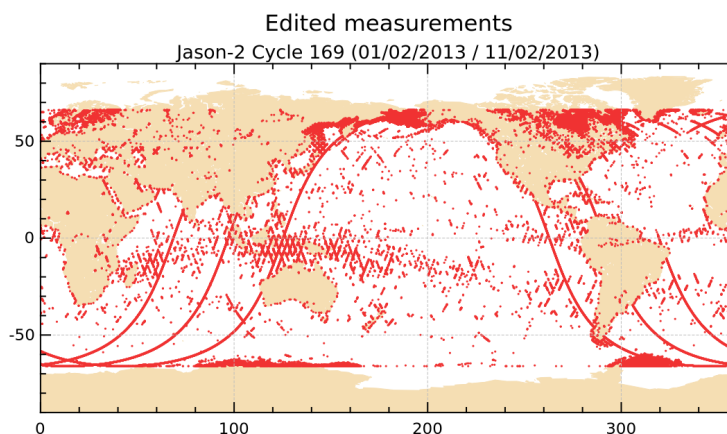
FIG. 2 – Edited measurements for cycle 169.
