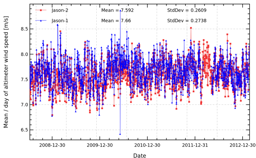
FIG. 10 – Daily monitoring of altimeter wind speed for Jason-2 and Jason-1.
