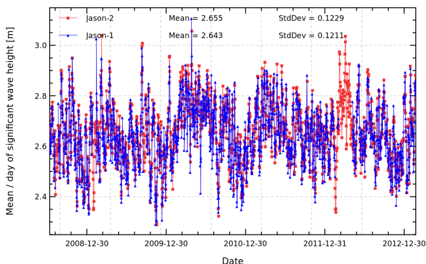
FIG. 6 – Daily monitoring of Ku-band significant wave height for Jason-2 and Jason-1.
