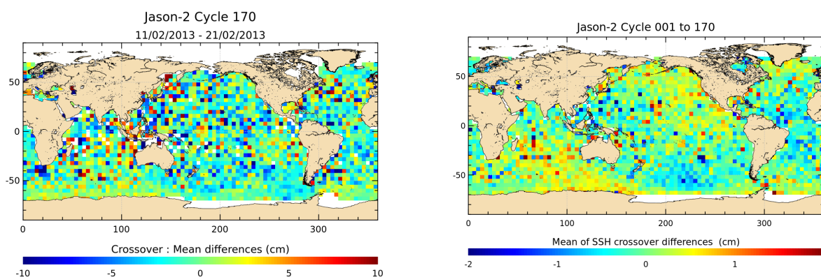
FIG. 12 – Mean SSH at crossovers for cycle 170 (left) and over the whole Jason-2 period (right).
