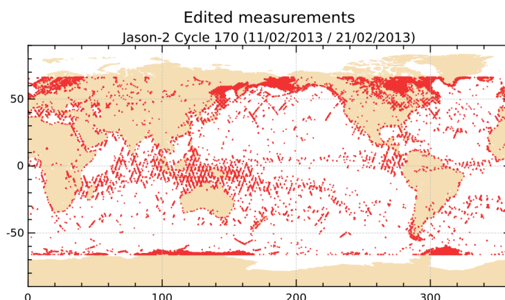
FIG. 2 – Edited measurements for cycle 170.
