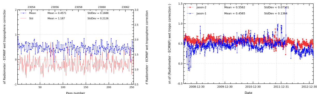
FIG. 11 – Pass monitoring of wet troposphere differences between radiometer and ECMWF model for Jason-2 cycle 170 (left) and daily monitoring of wet troposphere differences between radiometer and ECMWF model (right).
