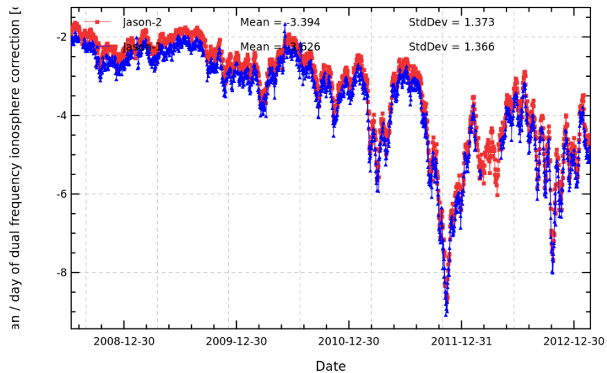
FIG. 8 – Daily monitoring of dual-frequency ionosphere correction for Jason-2 and Jason-1.
