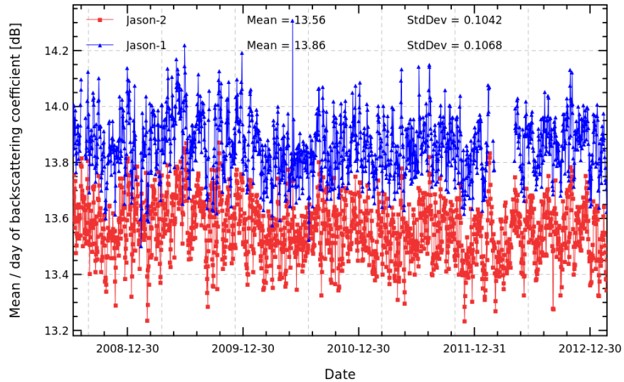
FIG. 7 – Daily monitoring of Ku-band backscattering coefficient for Jason-2 and Jason-1.
