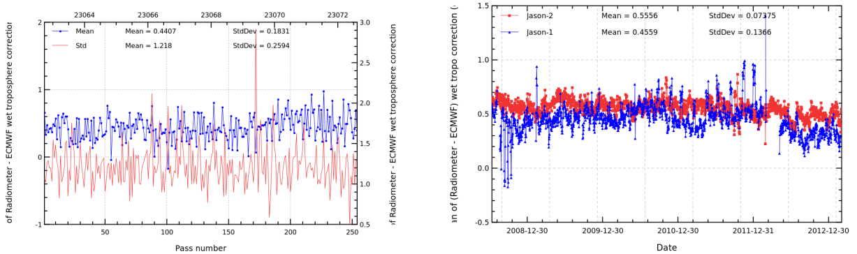
FIG. 11 – Pass monitoring of wet troposphere differences between radiometer and ECMWF model for Jason-2 cycle 171 (left) and daily monitoring of wet troposphere differences between radiometer and ECMWF model (right).
