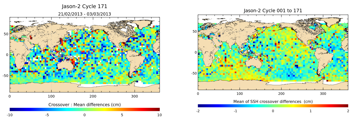
FIG. 12 – Mean SSH at crossovers for cycle 171 (left) and over the whole Jason-2 period (right).
