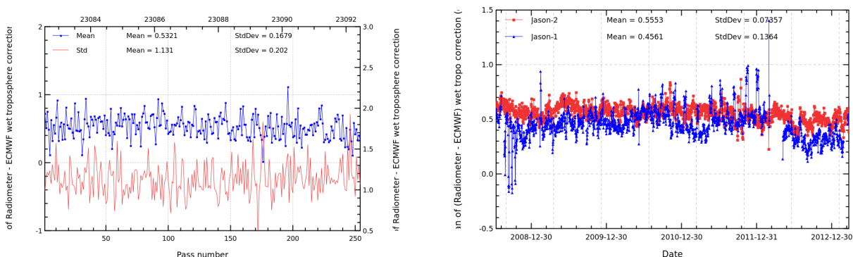
FIGURE 11 – Pass monitoring of wet troposphere differences between radiometer and ECMWF model for Jason-2 cycle 173 (left) and daily monitoring of wet troposphere differences between radiometer and ECMWF model (right).
