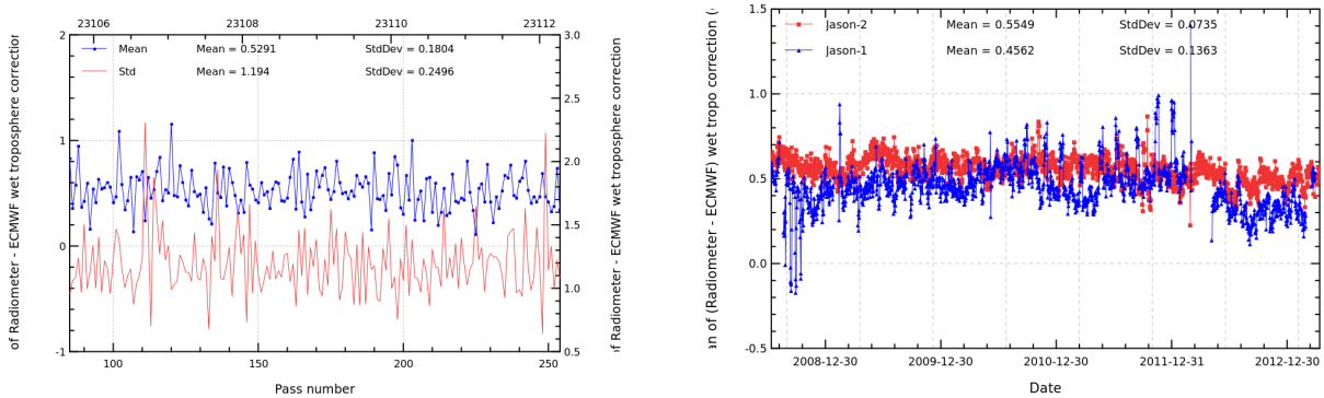
FIGURE 11 – Pass monitoring of wet troposphere differences between radiometer and ECMWF model for Jason-2 cycle 175 (left) and daily monitoring of wet troposphere differences between radiometer and ECMWF model (right).
