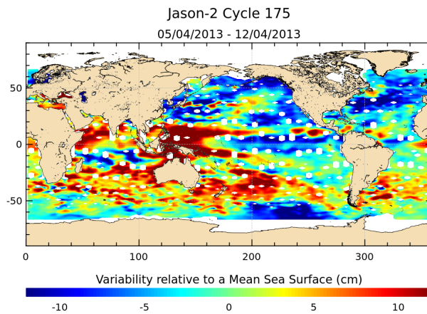
FIGURE 17 – Sea level anomaly relative to MSS for cycle 175.
