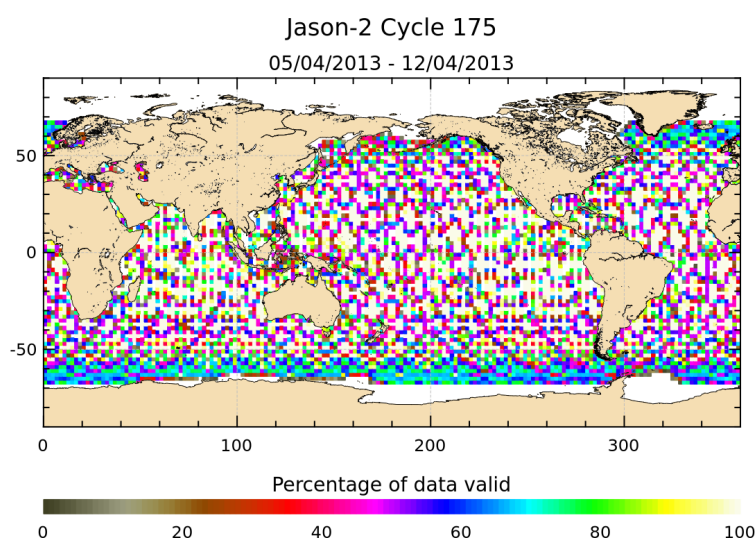
FIGURE 3 – Percentage of valid measurements for cycle 175.
