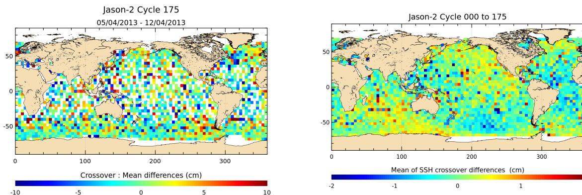
FIGURE 12 – Mean SSH at crossovers for cycle 175 (left) and over the whole Jason-2 period (right).
