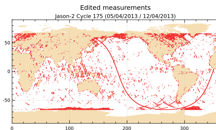
FIGURE 2 – Edited measurements for cycle 175.
