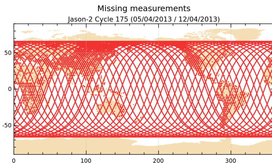
FIGURE 1 – Missing measurements for cycle 175.
