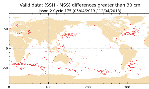
FIGURE 18 – Differences higher than a 30 cm threshold for cycle 175.
