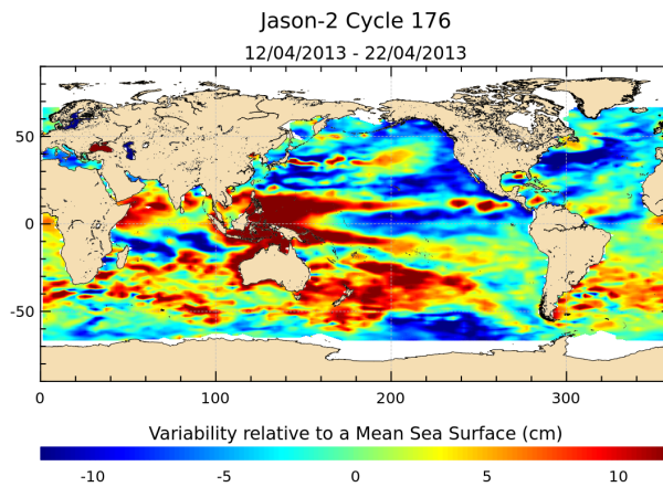
FIGURE 17 – Sea level anomaly relative to MSS for cycle 176.
