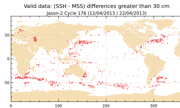
FIGURE 18 – Differences higher than a 30 cm threshold for cycle 176.
