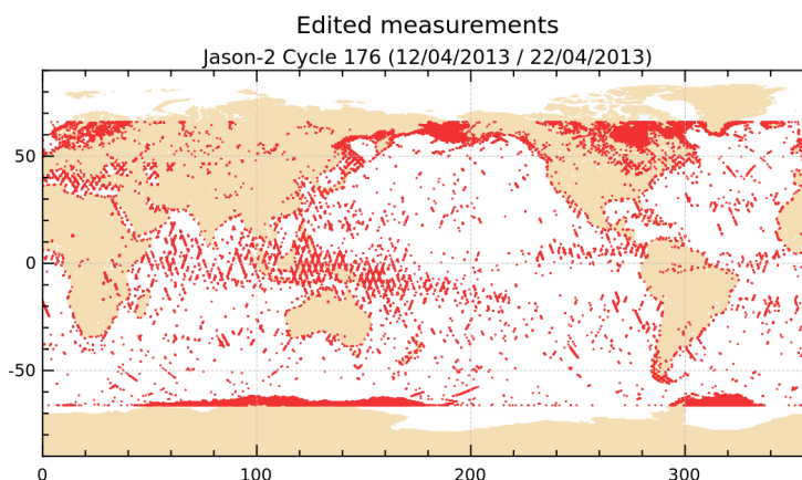
FIGURE 2 – Edited measurements for cycle 176.
