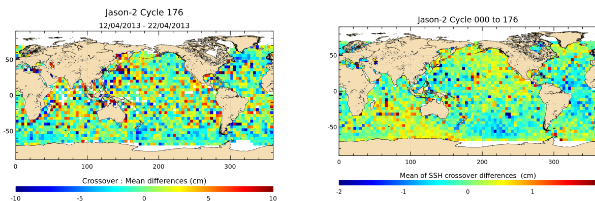
FIGURE 12 – Mean SSH at crossovers for cycle 176 (left) and over the whole Jason-2 period (right).
