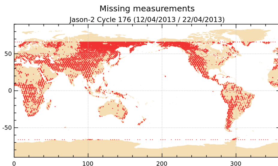
FIGURE 1 – Missing measurements for cycle 176.
