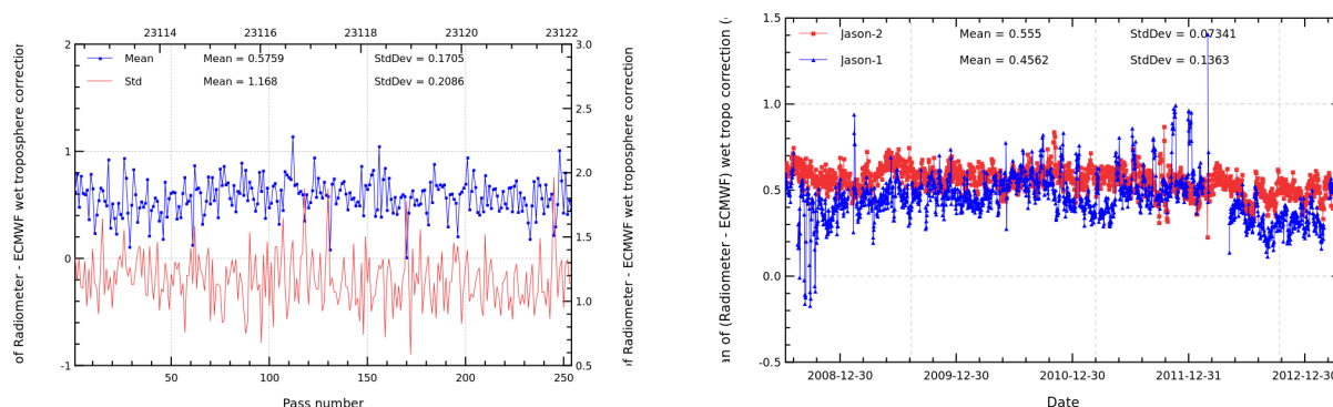
FIGURE 11 – Pass monitoring of wet troposphere differences between radiometer and ECMWF model for Jason-2 cycle 176 (left) and daily monitoring of wet troposphere differences between radiometer and ECMWF model (right).
