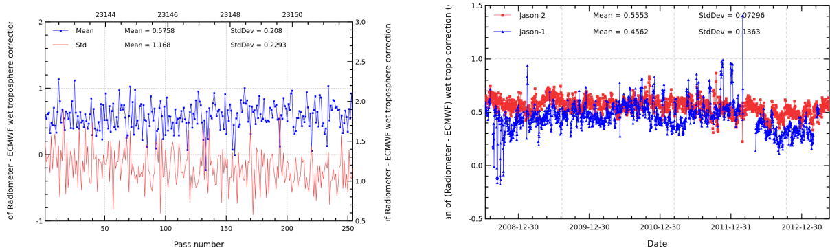
FIGURE 11 – Pass monitoring of wet troposphere differences between radiometer and ECMWF model for Jason-2 cycle 179 (left) and daily monitoring of wet troposphere differences between radiometer and ECMWF model (right).
